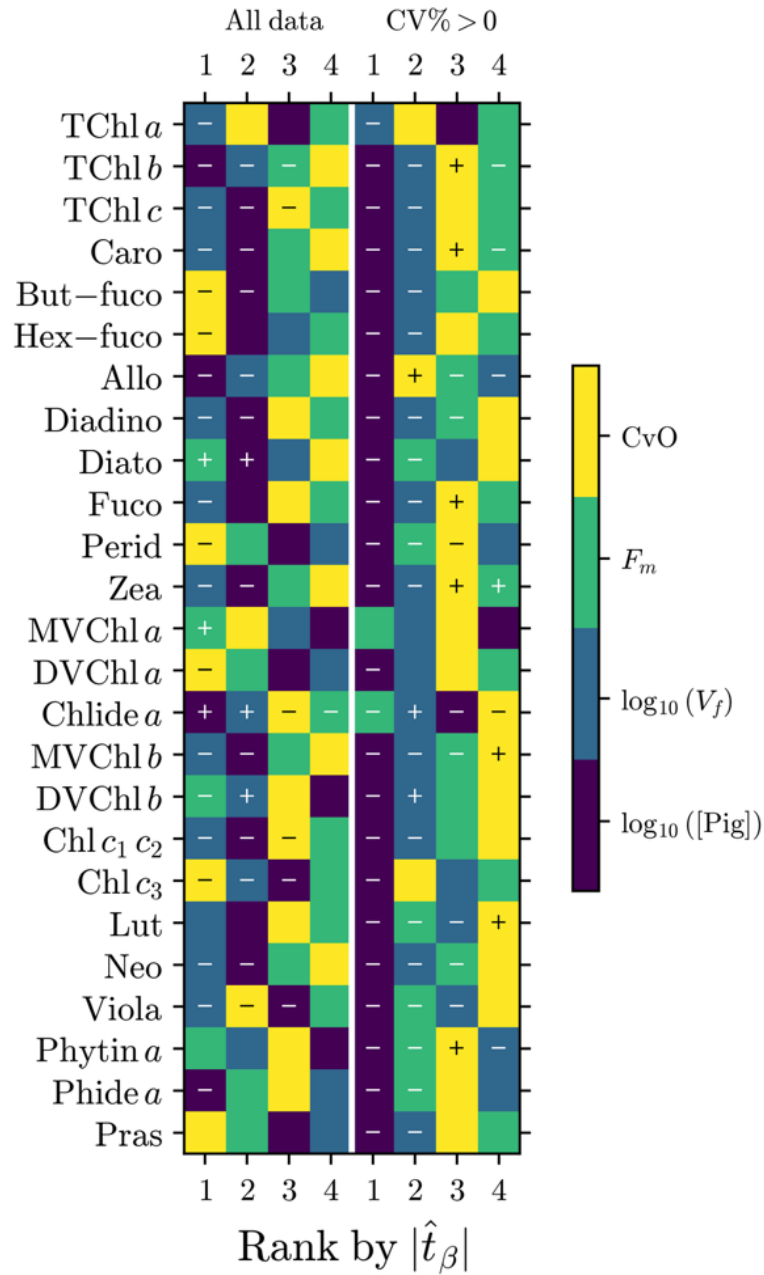
405 Figure 10: Variable importance rankings (1–4, based on normalized regression coefficient magnitudes |\hat{t}_\beta| ) from multivariate models predicting pigment precision. Left: full dataset. Right: censored dataset (CV% > 0, excluding invariant replicates). Symbols show effect direction: '+' = increases CV% (worsens precision), '-' = decreases CV% (improves precision), blank = non-significant ( \alpha = 0.05 ). Variables [color-coded]: \log_{10}([Pig]) = pigment concentration, \log_{10}(V_f) = filtered volume, F_m = microplankton fraction, CvO = coastal vs. oceanic.
