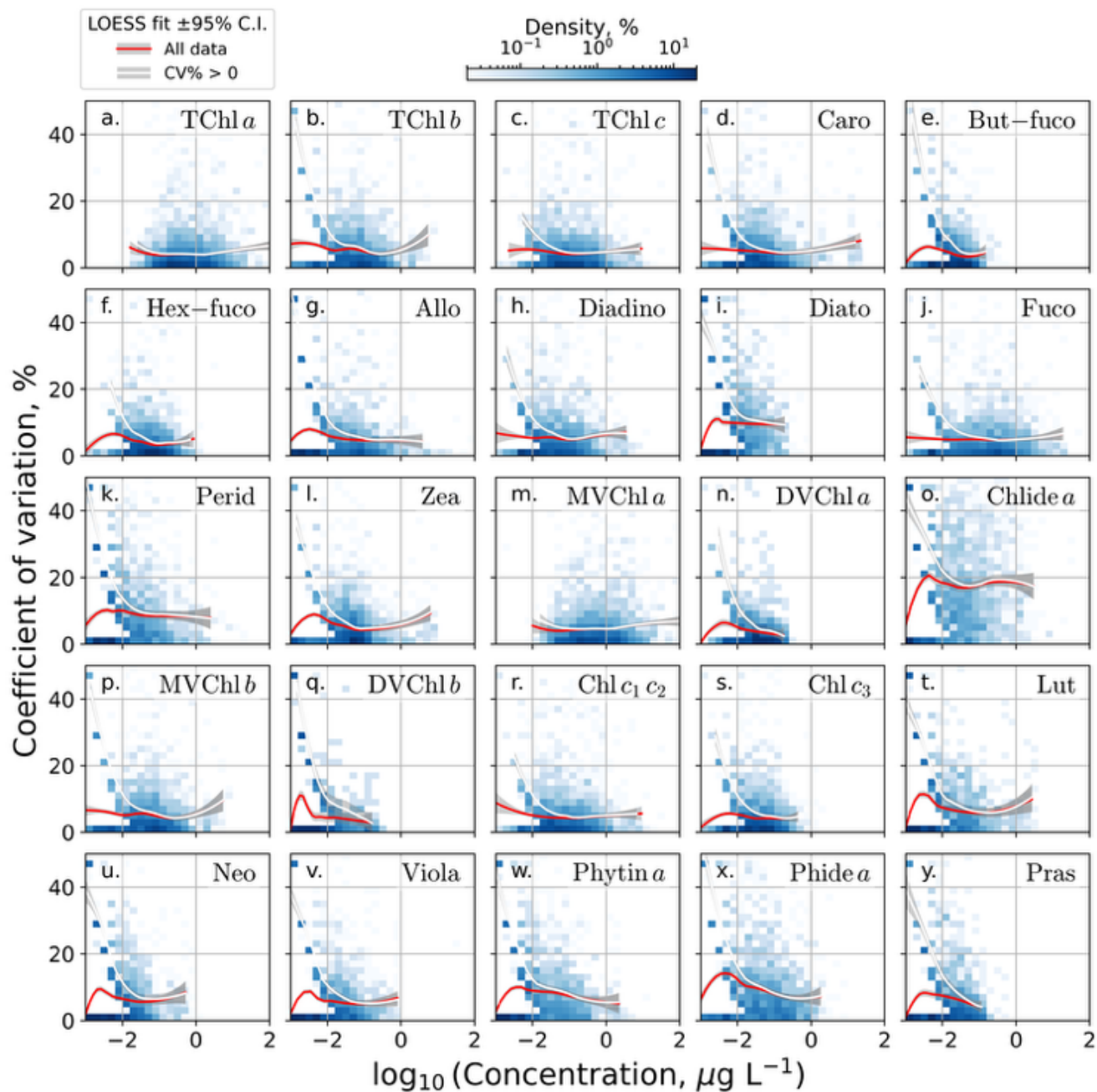
385 Figure 5: Replicate sample precision (CV %) versus \log_{10} -transformed pigment concentration for each phytoplankton pigment. LOESS regression fits on all data (red line) and CV % > 0 only data (white line), with 95 % CIs shaded. 2D histograms display CV % sample density, with color bar showing percent sample density.
