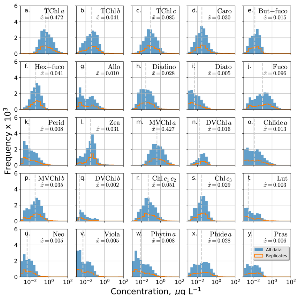
Figure 1: Distribution of phytoplankton pigment concentrations (mg m -3 ) analyzed by HPLC at the NASA GSFC facility during 2011-2022. Bars indicate counts for all samples, while orange stairs show replicate sample fraction. Vertical lines denote the median concentration.
