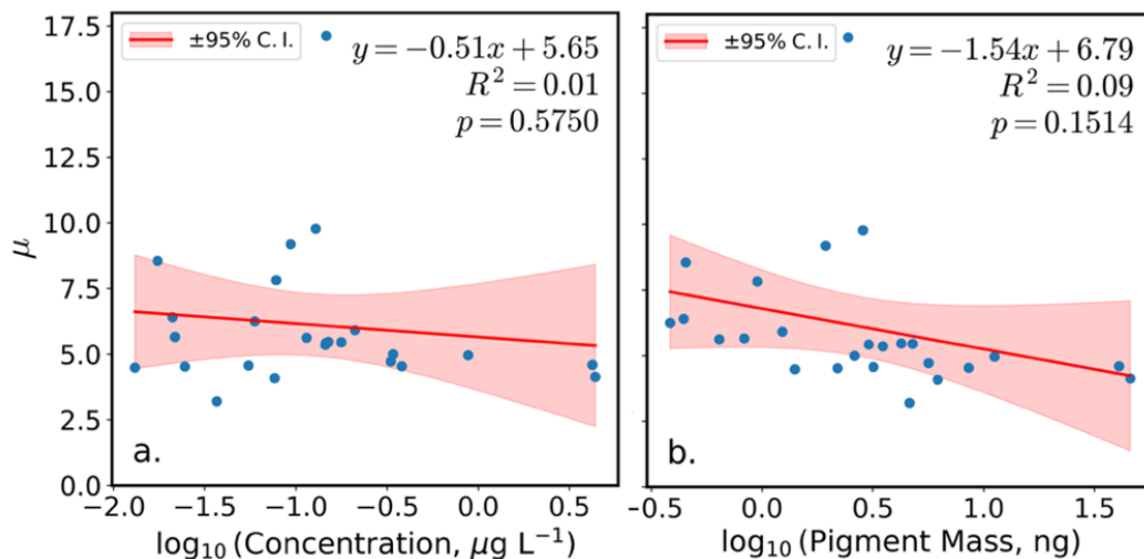
Figure 4: Mean coefficient of variation percentage (CV %) precision versus (a.) mean \log_{10} -transformed pigment concentration, and (b.) \log_{10} -transformed mean pigment mass. The adjusted R^2 quantifies goodness of fit, while the p -value tests significance of the slope.
