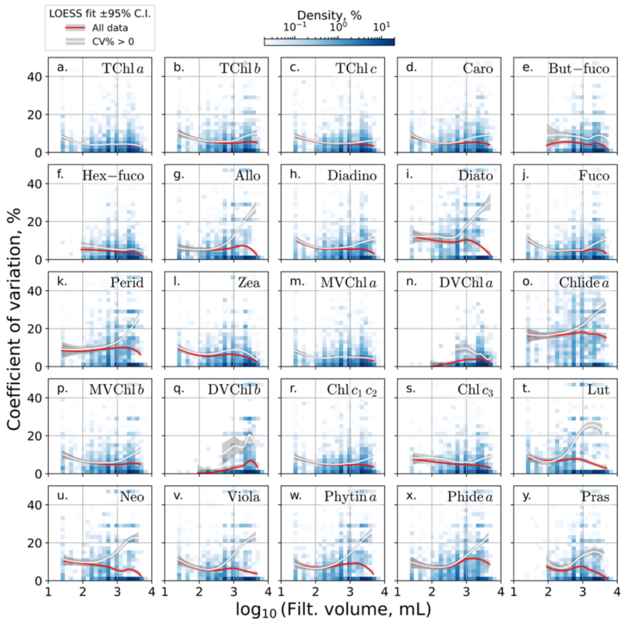
395 Figure 7: Replicate sample precision (CV %) versus \log_{10} -transformed filtered volume for each phytoplankton pigment. LOESS regression fits on all data (red line) and CV % > 0 only data (white line), with 95 % CIs shaded. 2D histograms display CV % sample density, with color bar showing percent sample density.
