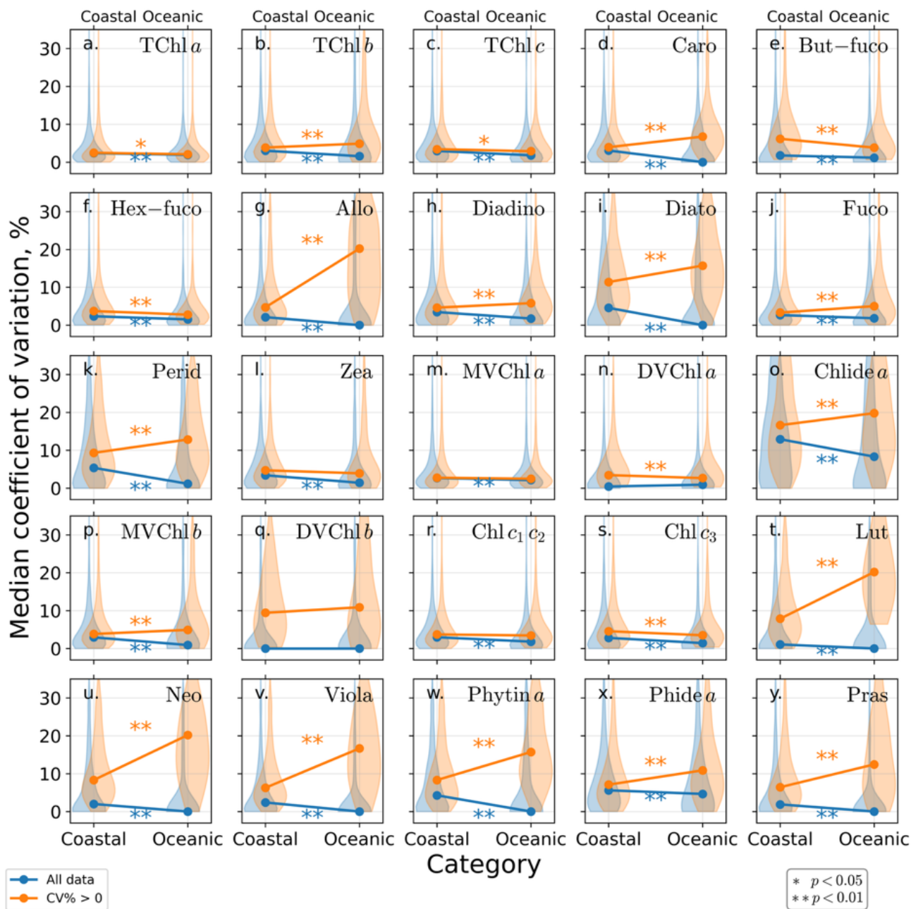
Figure 9: Median sample precision (CV %) for phytoplankton pigments from coastal (<200km from shore) versus oceanic (>200km). Differences assessed using Mann-Whitney U test on full dataset (blue) and subset with CV > 0 only (orange). Violin plots depict data distribution per category. Comparisons marked “*” and “**” indicate statistically significant precision differences between coastal and oceanic at \alpha=0.05 and \alpha=0.01 , respectively.
