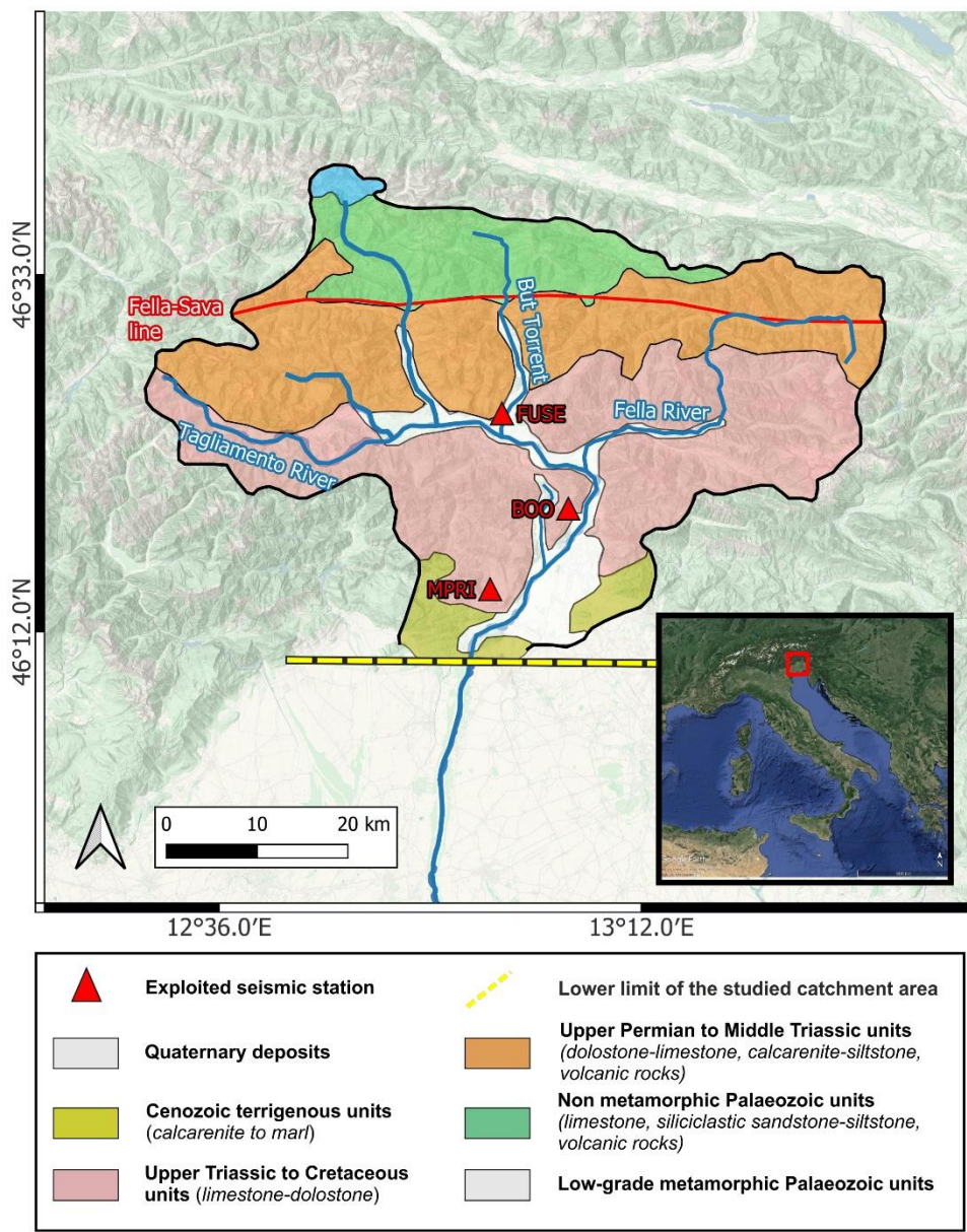
Figure 1: Geological setting of the Tagliamento catchment with exploited seismic stations and main tributaries. The red line is the Fella-Sava fault and the yellow dashed line indicates the lower limit of the studied area. The inset shows the Italy satellite map with the location of the study area. The satellite map was uploaded from Google Earth on QGIS, the topographic map was uploaded from ESRI, while the layer of geological units was drawn on the map by the authors based on Monegato and Stefani (2010) geological map of the catchment.
