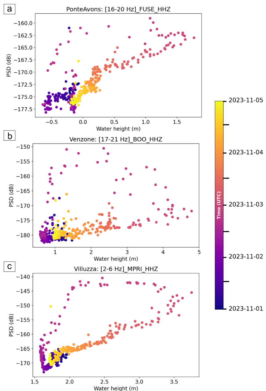
Figure 8: PSD related to the water height color-coded with time of occurrence for the FUSE (a), BOO (b-e) and MPRI (c-f) stations in 16-20, 1-5 and 17-21, and 2-6 Hz frequency bands respectively during the Ciarán storm flood event.
