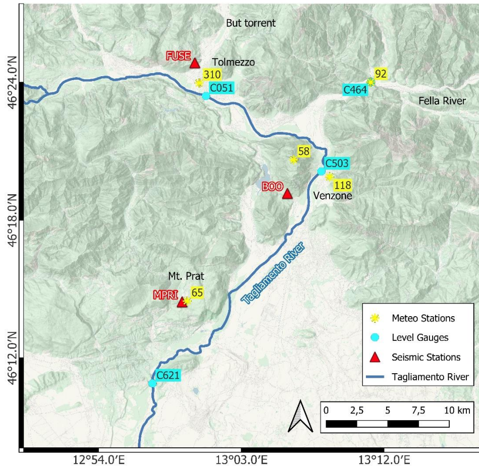
Figure 2: Map of “Alto Tagliamento” showing the selected seismic stations closest to the riverbed, pluviometric stations (referred to: 310-Tolmezzo Campo Sportivo, 92-Moggio Udinese, 58-Mt. S. Simeone, 118-Venzone, 65-Mt.Prat) and level gauges (C051-Ponte Avons, C464-Moggio Udinese, C503-Venzone, C621-Villuzza). The satellite topographic map was uploaded from Google EarthESRI on QGIS.
