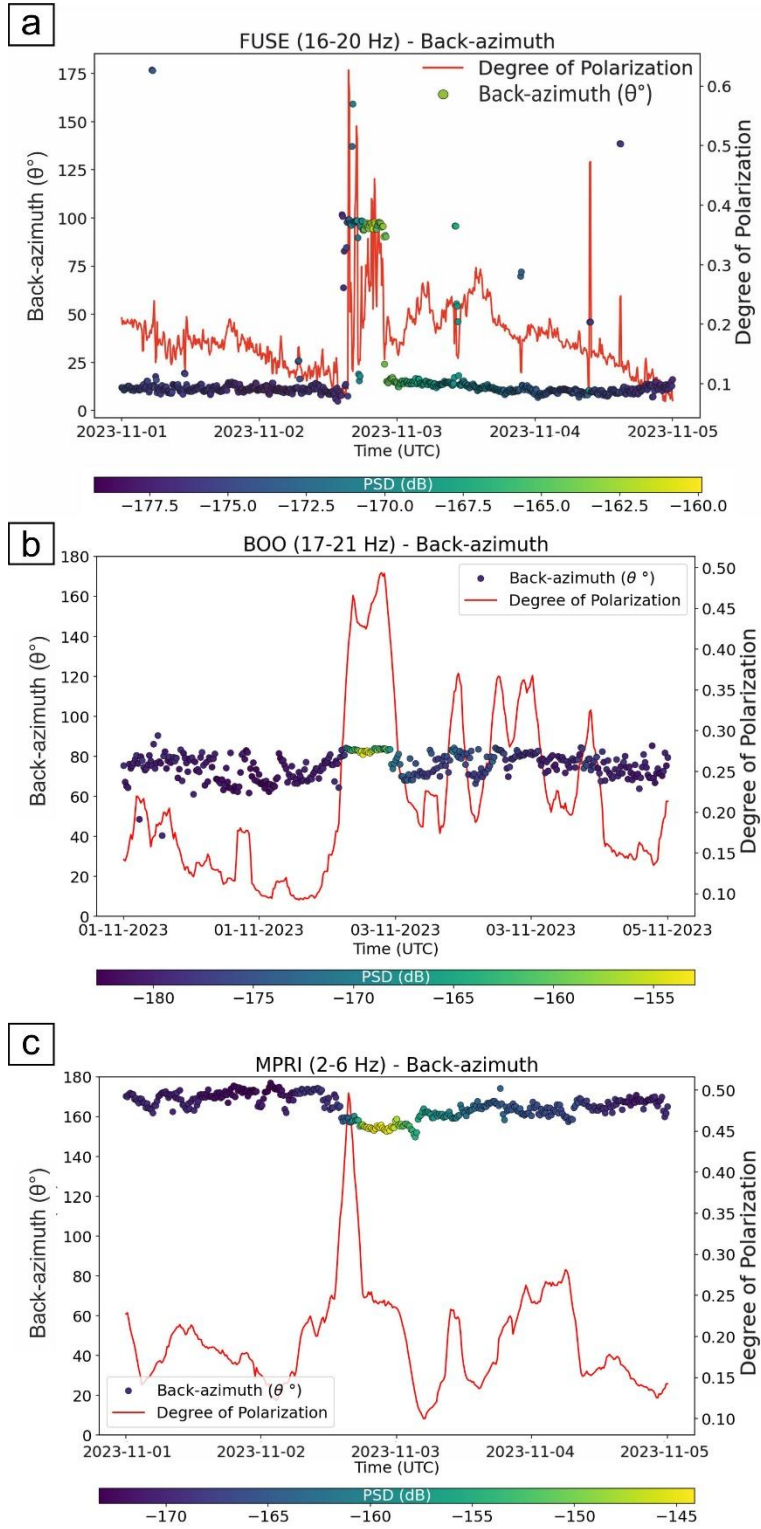
Figure 9: Polarization analysis for (a) FUSE, (b) BOO and (c) MPRI seismic stations in frequency ranges with the highest value obtained by Spearman correlation results. The back azimuth value ( \theta^\circ ) over the investigated period is related to the PSD (dB) with a colour palette, underlining the peak of the seismic event during the flood, while in red line the degree of polarization is shown.
