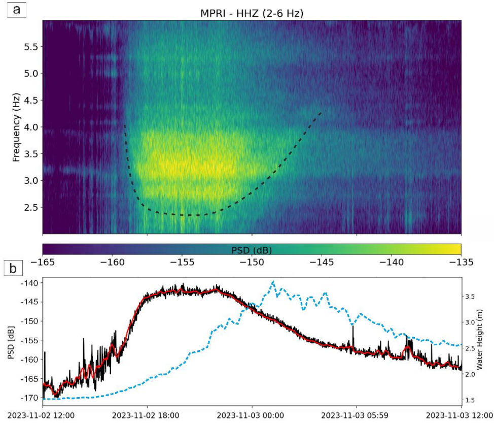
Figure 4: a) Zoom in the 24-hour spectrogram of the vertical component at station MPRI between 2 and 6 Hz highlighting the V shape contouring the high PSD values (dashed black line). b) Average PSD (in dB, black line) calculated from the above spectrogram. The red line corresponds to the median PSD values over a sliding window of 120 s length, while the blue line refers to the water height variation data.
