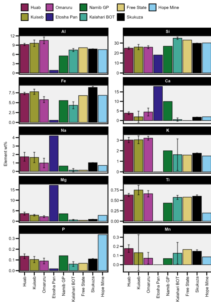
465 Figure 2. Fractions of crustal elements (wt%) in Saf dust aerosols by source region. Standard deviations are calculated from multiple samples; if not shown, this indicates that only a single sample was available. Samples collected across Botswana from the Kalahari are grouped into the Kalahari BOT dataset. Namib GP refers to the Central Namib Gravel Plain.
