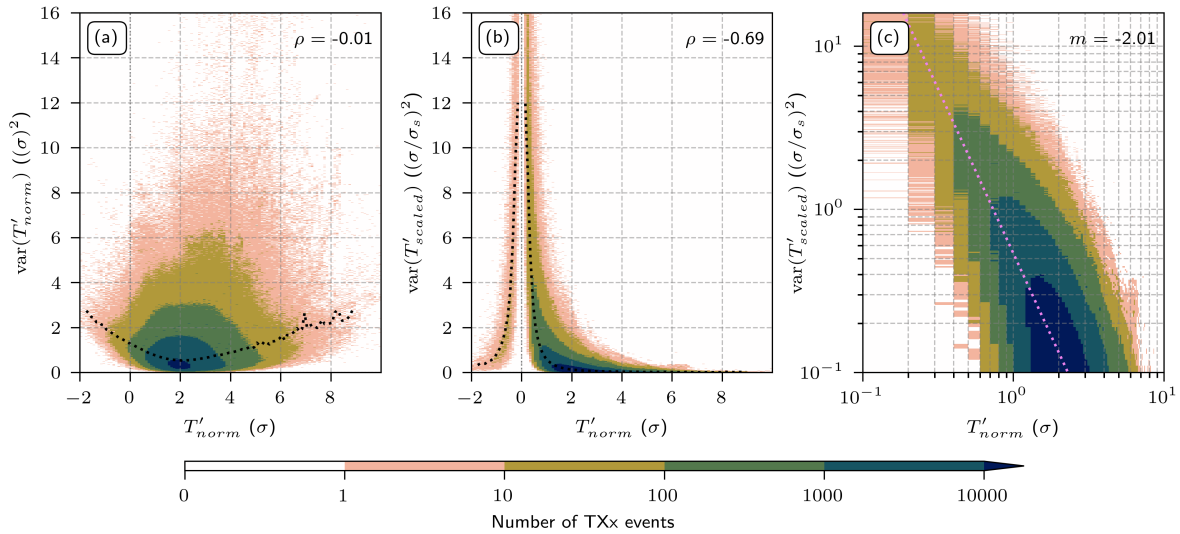
Figure 7. Joint distributions of the mean vertical variance of individual TXx event profiles relative to their median profile and near-surface T'_{scaled}(k=0) (lowest model level), (a) for T'_{norm} , (b) T'_{scaled} , and (c) T'_{scaled} in log-log-scale. The values of \rho in the upper right corner in (a, b) denote the Spearman correlation (both p-values < 10^{-3} ). Bin widths are 0.1 \sigma (x-axis) and 0.02 \sigma or 0.02 \sigma/\sigma_s (y-axis). The black dotted line marks the weighted median. The violet dotted line and the m value in the upper right corner in (c) indicate the regression line and slope, respectively. Note that the negative T'_{scaled}(k=0) values on the x-axes arise from our event definition and make up 0.03 % of the TXx events.
