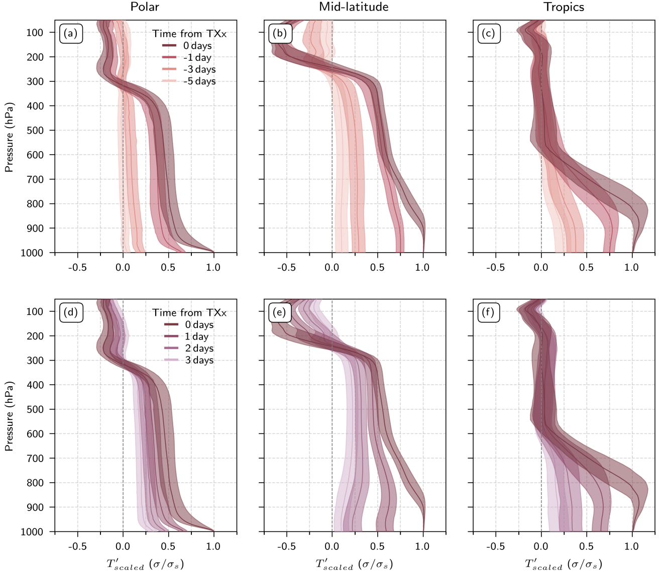
Figure 3. Temporal evolution of the median and interquartile range of the median scaled temperature anomalies ( T'_{scaled,C} ) of all the grid points (a–c) during the 5-day genesis and (d–f) 3-day decay of TXx events for (a, d) the polar, (b, e) mid-latitude, and (c, f) tropical clusters. The surface pressure is set again to a reference pressure of 1000 hPa.
