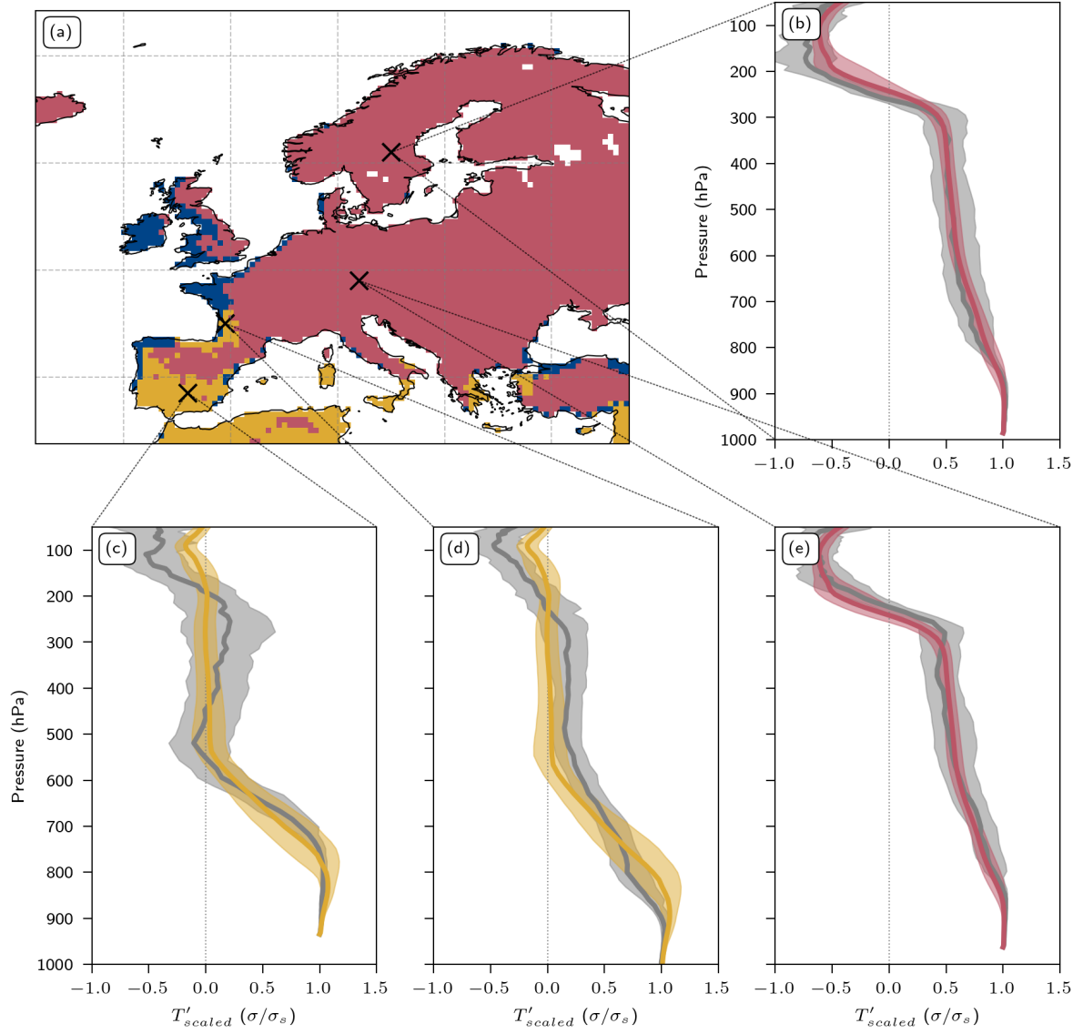
Figure D1. Area-weighted k -means clustering with three clusters from Fig. 2a shown as (a) a zoomed in map of Europe and (b–e) vertical T'_{scaled} profiles for individual grid points at (b) 61^{\circ} N, 15^{\circ} E, (c) 38.5^{\circ} N, 4^{\circ} W, (d) 45^{\circ} N, 0.5^{\circ} W, and (e) 49^{\circ} N, 12^{\circ} E. The grey line and its shading denote the median and interquartile range of all TXx events at that grid point, the yellow, red, and blue lines and shading the clusters' median and interquartile range of all \overline{T'_{scaled}} within the tropical, mid-latitude, and polar clusters, respectively. For the cluster \overline{T'_{scaled}} profiles, we use the median surface pressure of the TXx events as a reference pressure to interpolate on pressure levels.
