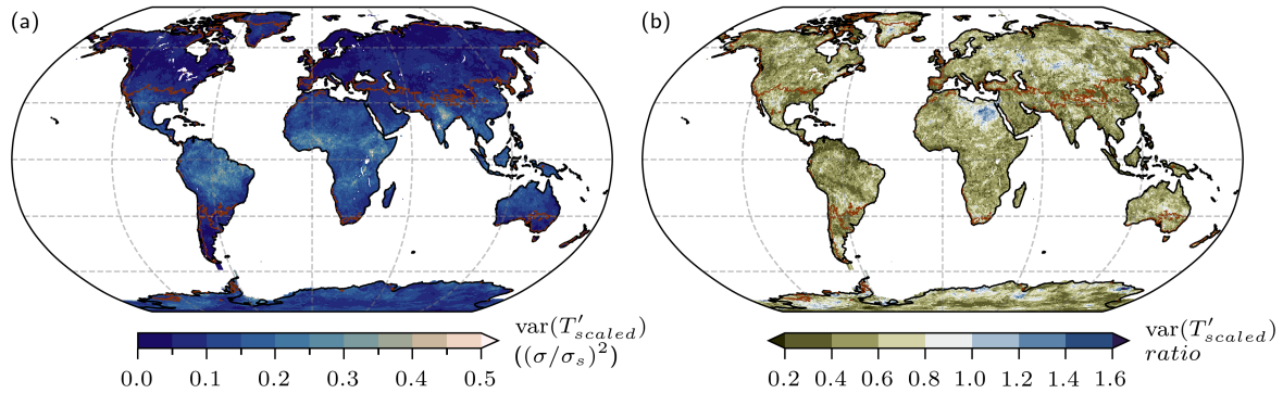
Figure 6. (a) Variance of T'_{scaled} profiles for the 10 hottest TXx events relative to the median profile of all TXx events ( \text{var}(T'_{scaled}) ), and (b) the ratio of \text{var}(T'_{scaled}) between the hottest 10 TXx events and moderate TXx events (which exclude the hottest and coldest 10 TXx events). Fields in both panels are vertically averaged over all hybrid sigma–pressure levels. The brown lines denote the boundaries between the three clusters.
