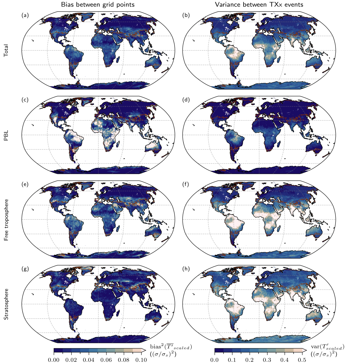
Figure 5. Distribution of (left) \text{bias}^2(\overline{T'}_{scaled}) and (right) \text{var}(T'_{scaled}) , vertically averaged over (a, b) all hybrid sigma–pressure levels, (c, d) only the PBL, (e, f) only the free troposphere, and (g, h) only the stratosphere. The brown lines denote the boundaries between the three clusters. The coldest 10 TXx events are excluded at each grid point. Note the different scales used for \text{bias}^2(\overline{T'}_{scaled}) and \text{var}(T'_{scaled}) .
