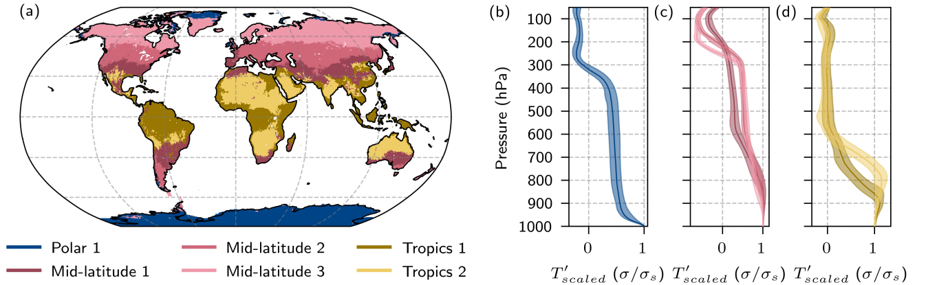
Figure 4. Refinement of the global area-weighted clustering with now six clusters over land: (a) map of clusters polar 1 (dark blue, N = 30,127 grid points), mid-latitude 1 (red, N = 9,124 ), mid-latitude 2 (dark pink, N = 10,312 ), mid-latitude 3 (light pink, N = 17,422 ), tropics 1 (brown, N = 11,299 ), and tropics 2 (yellow, N = 9,865 ). (b–d) Median and interquartile range of the vertical median scaled T' profile of all the grid points within each cluster for the (b) polar, (c) mid-latitude, and (d) tropical clusters on pressure levels (surface pressure set again to the reference pressure 1000 hPa).
