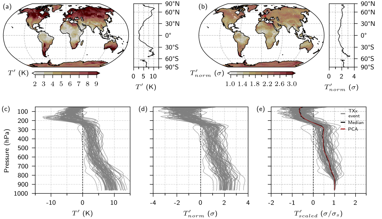
Figure 1. Global distribution of the (a) median temperature anomaly ( T' ) and (b) median normalised temperature anomaly ( T'_{norm} ) on the lowermost model level, of TXx events from 1951 to 2023. Vertical profiles (grey lines) of (c) T' , (d) T'_{norm} , and (e) scaled temperature anomaly ( T'_{scaled} ) of all TXx events at a land grid point in central Europe (49° N, 12° E), marked in (a, b) with a red cross. The black and red lines in (e) show the median profile of T'_{scaled} ( \overline{T'_{scaled}} ) over all TXx events and \overline{T'_{scaled}} after the PCA, respectively (see Sect. 2.3 for details).
