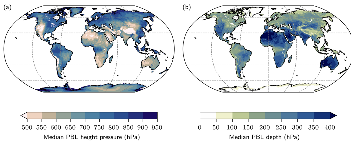
Figure A1. Global distribution of (a) the median PBL height (in hPa), and (b) the median PBL depth (also in hPa) during the 73 TXx events at each grid point.
