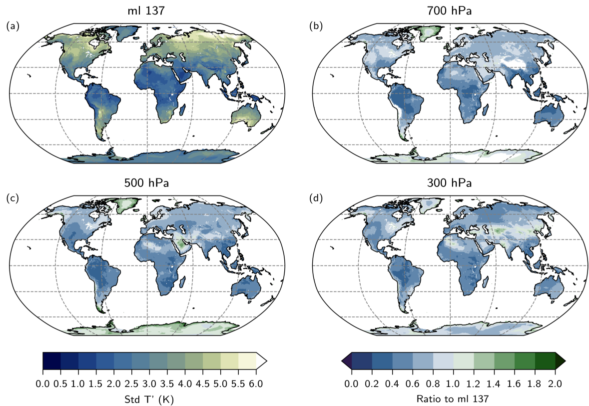
Figure C1. Global distribution of the mean standard deviation of the temperature anomaly at TXx events (a) at the lowest model level and the ratio of (b) interpolated to 700 hPa, (c) 500 hPa, and (d) 300 hPa to the lowest model level. The white areas over land in (b) are where the surface pressure is below 700 hPa.
