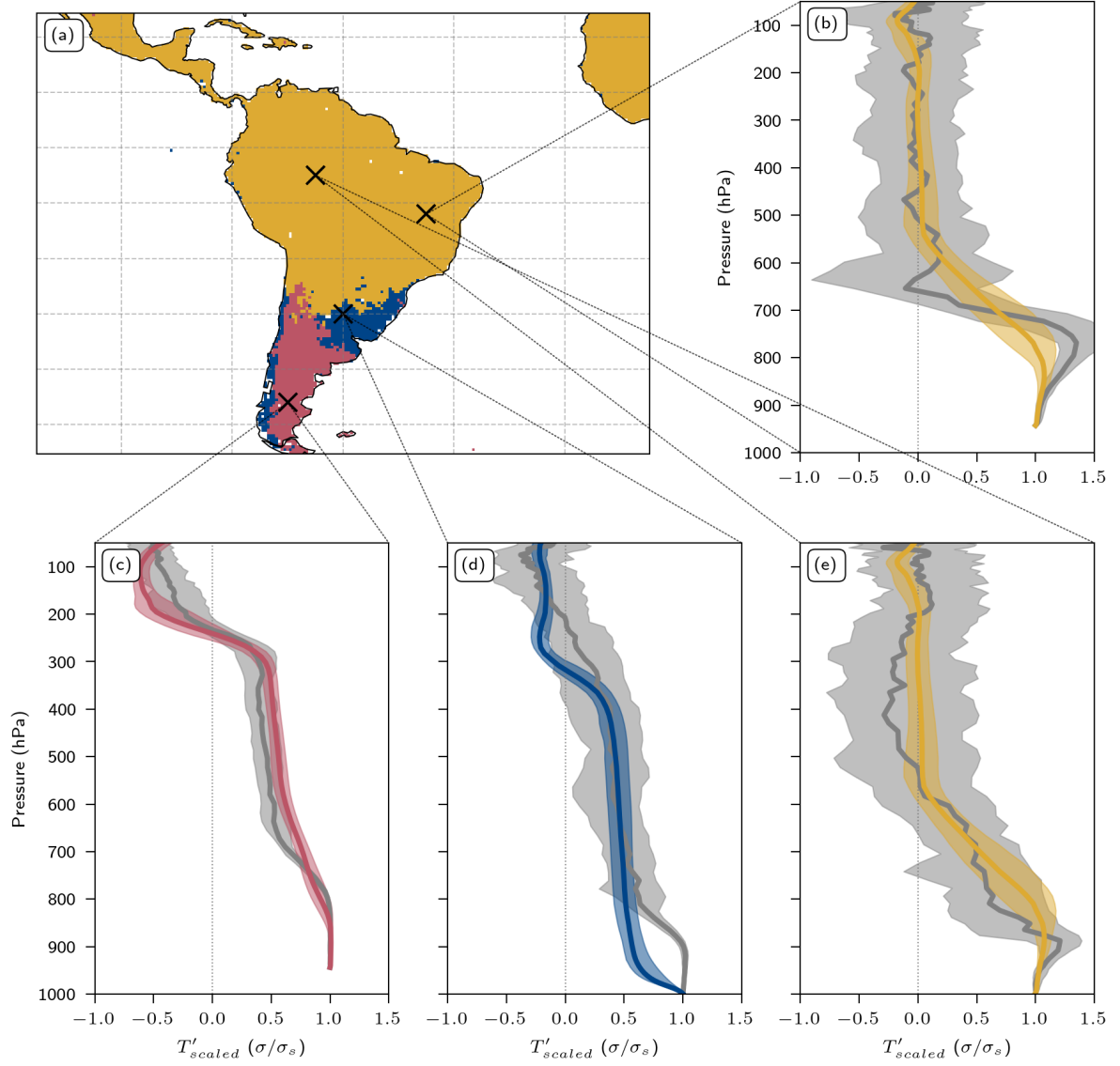
Figure D3. Area-weighted k -means clustering with three clusters from Fig. 2a shown as (a) a zoomed in map of South America and (b–e) vertical T'_{scaled} profiles for individual grid points, (b) 12° S, 45° W, (c) 46° S, 70° W, (d) 30° S, 60° W, and (e) 5° S, 65° W. The grey line and its shading denote the median and interquartile range of all TXx events at that grid point, the yellow, red, and blue lines and shading the clusters' median and interquartile range of all \overline{T'}_{scaled} within the tropical, mid-latitude, and polar clusters, respectively. For the cluster \overline{T'}_{scaled} profiles, we use the median surface pressure of the TXx events as a reference pressure to interpolate on pressure levels.
