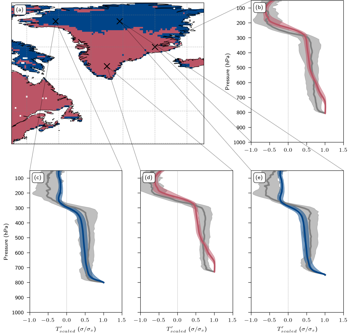
Figure D2. Area-weighted k -means clustering with three clusters from Fig. 2a shown as (a) a zoomed in map of Greenland and (b–e) vertical T'_{scaled} profiles for individual grid points, (b) 70° N, 30° W, (c) 78° N, 61° W, (d) 64° N, 45° W, and (e) 78° N, 41° W. The grey line and its shading denote the median and interquartile range of all TXx events at that grid point, the red and blue lines and shading the clusters' median and interquartile range of all \overline{T'_{scaled}} within the mid-latitude and polar clusters, respectively. For the cluster \overline{T'_{scaled}} profiles, we use the median surface pressure of the TXx events as a reference pressure to interpolate on pressure levels.
