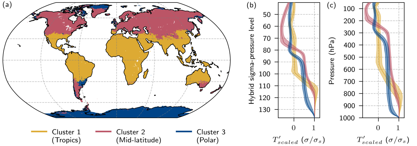
Figure 2. (a) Global distribution of the three area-weighted clusters over land: cluster 1 (yellow, N = 26,325 grid points), cluster 2 (red, N = 30,138 ), and cluster 3 (blue, N = 31,626 ). (b, c) median and interquartile range of the median vertical T'_{scaled} profiles of all grid points in each cluster, (b) on sigma-hybrid model levels and (c) on pressure levels (surface pressure set to the reference pressure 1000 hPa).
