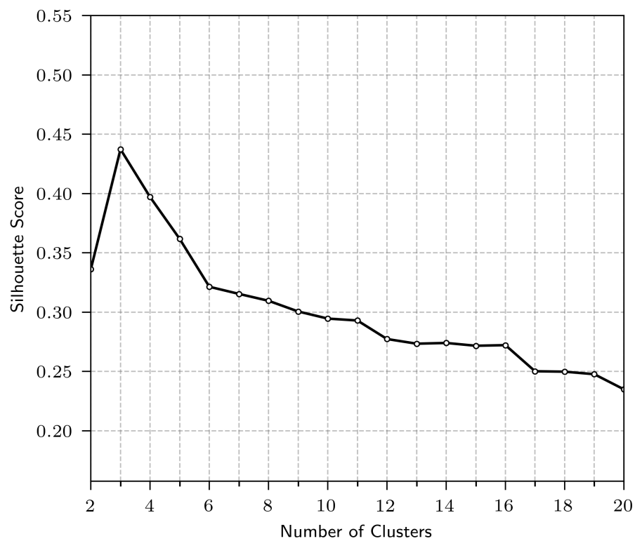
Figure B1. Silhouette score for finding an optimal number of clusters of the median scaled T' profiles over land grid points with the area-weighted k -means clustering approach, using the eight retaining components of all hybrid sigma-pressure levels.
