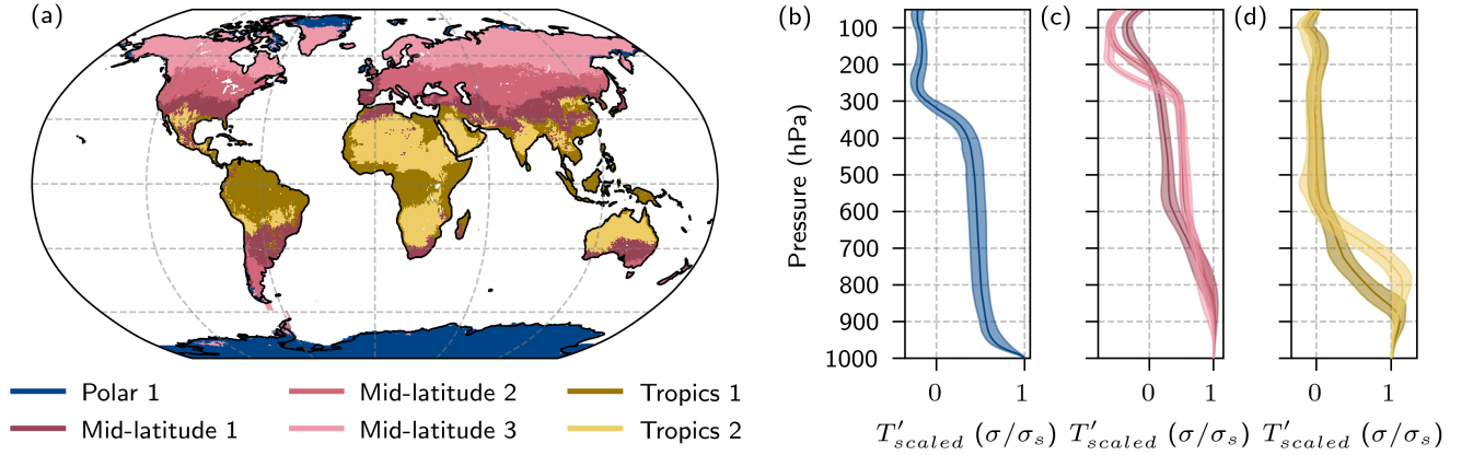
Figure 4. Refinement of the global area-weighted clustering with now six clusters over land: (a) map of clusters polar 1 (dark blue, N=30,127 grid points), mid-latitude 1 (red, N=9,124 ), mid-latitude 2 (dark pink, N=10,312 ), mid-latitude 3 (light pink, N=17,422 ), tropics 1 (brown, N=11,299 ), and tropics 2 (yellow, N=9,865 ). (b–d) Median and interquartile range of the vertical median scaled T' profile of all the grid points within each cluster for the (b) polar, (c) mid-latitude, and (d) tropical clusters on pressure levels (surface pressure set again to the reference pressure 1000 hPa).
