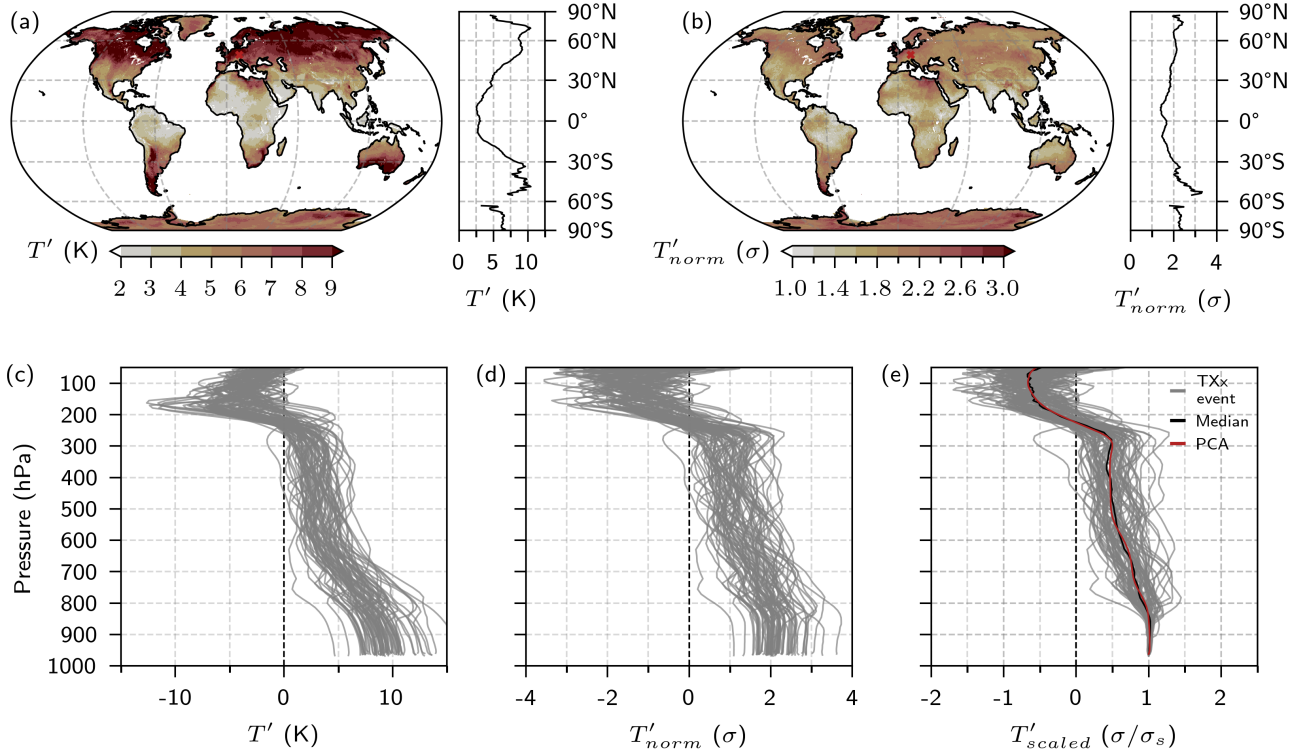
Figure 1. Global distribution of the median (a) median temperature anomaly ( T' ) and (b) median normalized temperature anomaly ( T'_{norm} ) on the lowermost model level, of TXx events from 1951 to 2023. Vertical profiles (grey lines) of (c) T' , (d) T'_{norm} , and (e) scaled temperature anomaly ( T'_{scaled} ) of all TXx events at a land grid point in central Europe (49° N, 12° E), marked in (a, b) with a red cross. The black and red lines in (e) show the median profile of T'_{scaled} ( \overline{T'_{scaled}} ) over all TXx events and \overline{T'_{scaled}} after the PCA, respectively (see Sect. 2.3 for details).
