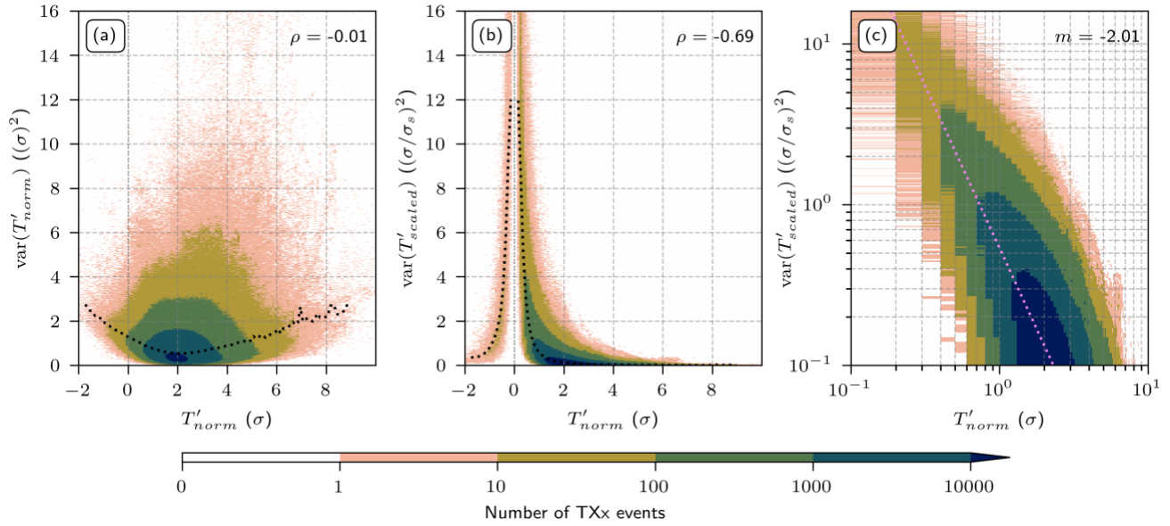
Figure R5: Joint distributions of the mean vertical variance of individual TXx event profiles relative to their median profile and near-surface T'_{scaled}(k = 0) (lowest model level), (a) for T'_{norm} , (b) T'_{scaled} , and (c) T'_{scaled} in log-log-scale. The values of \rho in the upper right corner in (a, b) denote the Spearman correlation (both p -values < 10^{-3} ). Bin widths are 0.1 \sigma (x-axis) and 0.02 \sigma or 0.02 \sigma/\sigma_s (y-axis). The black dotted line marks the weighted median. The violet dotted line and the m value in the upper right corner in (c) indicate the regression line and slope, respectively. Note that the negative T'_{scaled}(k = 0) values arise from our event definition and make up 0.03 % of the TXx events.
