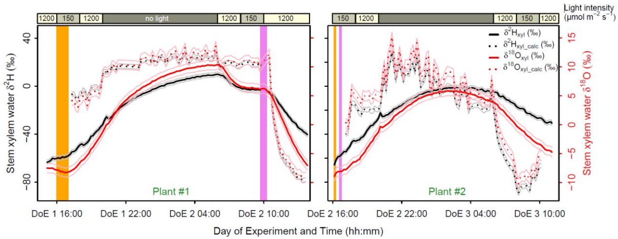
Figure 4: Comparison between calibrated observations (solid lines) and simulations of the hydrogen (black color) and oxygen (red) isotopic compositions of stem xylem water ( \delta_{xyl} ) over the courses of the 1 st experiment (sunflower plant #1, left hand side) and the 2 nd experiment (plant #2, right hand side). \delta_{xyl} was obtained from \delta_{stem} measurements and by applying the calibration functions (Eqs 6a and 6b). The error in the determination of \delta_{stem} is indicated on the same plot panel by the grey and light red lines for ^2\text{H} and ^{18}\text{O} , respectively. \delta_{xyl\_calc} was obtained from root water uptake measurements with the Soil Water Profiler and from simulated soil water isotopic composition profiles using Eq (1bis). The orange (violet) vertical stripes indicate the time when isotopically enriched (depleted) water was added to the upper (middle) soil layers of the columns. The yellow, light grey, and dark grey boxes above the plot indicate the time periods of high light intensity, low light intensity, and where there was no light inside the climate chamber.
