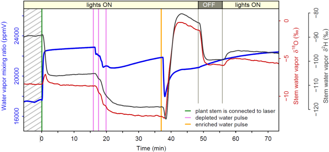
685 Figure E1. Investigation of the response times in stem water vapor \delta^2\text{H} (‰, black curve) and \delta^{18}\text{O} (‰, red curve) of one individual plant following several “cold” labeling pulses (water temperature \sim 10^\circ\text{C} versus soil initial water temperature \sim 20^\circ\text{C} ) and following light intensity changes. The depleted and enriched water pulses were applied 16 and 37 minutes (see the violet and orange vertical lines) after connection of the plant stem to the laser spectrometer (as indicated by the green vertical line). LED lights were switched off 48 minutes after stem connection to the laser spectrometer and turned off again 7 minutes later.
