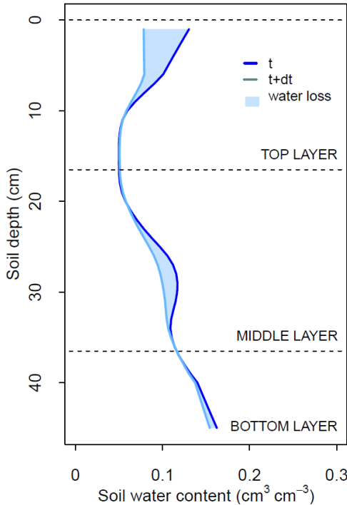
Figure B1. Graphical illustration of the method for determining the plant total root water uptake (RWU, expressed in ml water per time) between time t and (t+dt) on basis of the data collected by the Soil Water Profiler.
