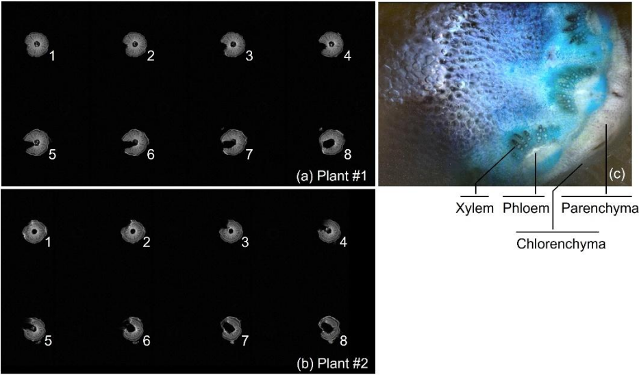
Figure G1. Magnetic Resonance Imaging (MRI) pictures of the stems of plant #1 (panel a) and plant #2 (panel b).
