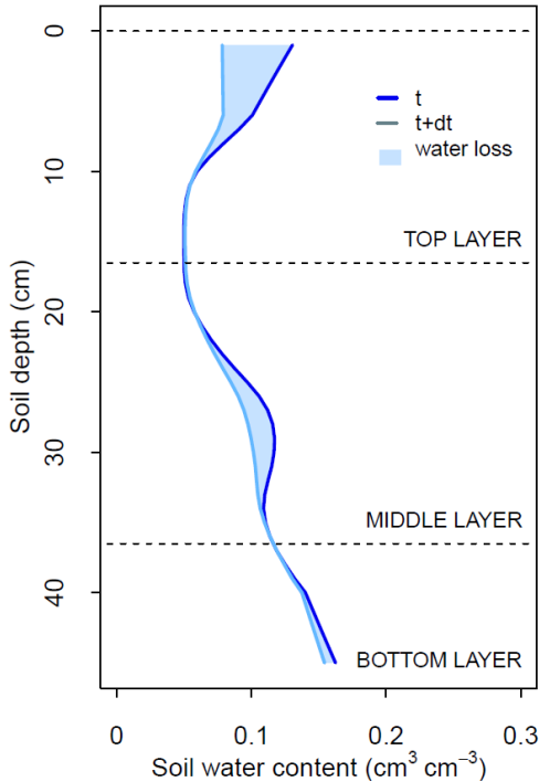
Figure A+B1. Graphical illustration of the method for determining the plant total root water uptake (RWU, expressed in ml water per time) between time t and (t+dt) on basis of the data collected by the Soil Water Profiler.
