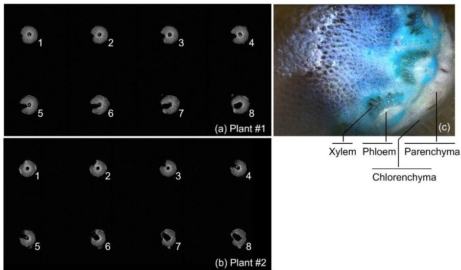
Figure F4G1. Magnetic Resonance Imaging (MRI) pictures of the stems of plant #1 (panel a) and plant #2 (panel b).
