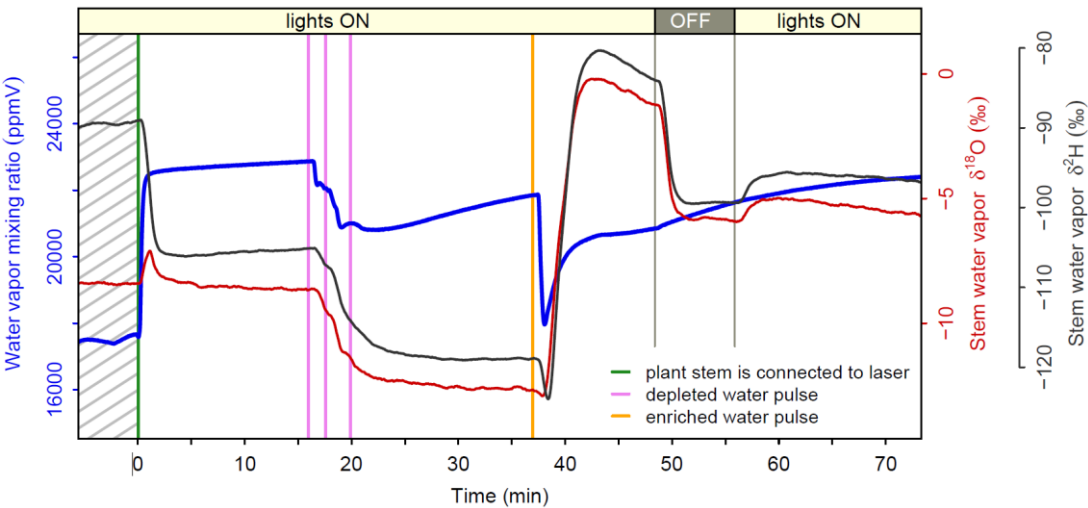
Figure D4E1. Investigation of the response times in stem water vapor \delta^2\text{H} (‰, black curve) and \delta^{18}\text{O} (‰, red curve) of one individual plant following several “cold” labeling pulses (water temperature \sim 10^\circ\text{C} versus soil initial water temperature \sim 20^\circ\text{C} ) and following light intensity changes. The depleted and enriched water pulses were applied 16 and 37 minutes (see the violet and orange vertical lines) after connection of the plant stem to the laser spectrometer (as indicated by the green vertical line). LED lights were switched off 48 minutes after stem connection to the laser spectrometer and turned off again 7 minutes later.
