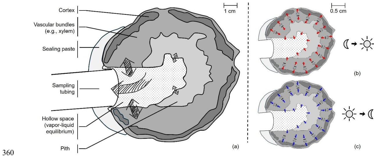
365 Figure 5: Conceptual drawing of one sunflower plant stem section based on one of the magnetic resonance imaging pictures of plant #1 made after the experiment (panel a; see also Appendix FG , Fig. F4G1 ). The hollow space resulting from the drilling and the installation of the sampling tubing is thought to contain water vapor equilibrated with different (liquid) water bodies contained in different stem tissues, but mainly from the vascular bundles (e.g., xylem vessel). In panels (b) and (c), situations are depicted where lights are switched from low to high intensity and from high to low intensity, respectively. In the first case (b), the opening of the stomata induces an increase in transpiration, which is initially only partly counterbalanced by an increase in root water uptake. Water is mobilized from other non-conducting tissues located in the pith and the cortex and contributes to stem water flow. In the second case (c), the closing of the stomata induces a decrease in transpiration, which is initially only partly counterbalanced by a decrease in root water uptake. Water is redistributed from the vascular bundles (e.g., xylem) back to the pith and to the cortex regions. 370
