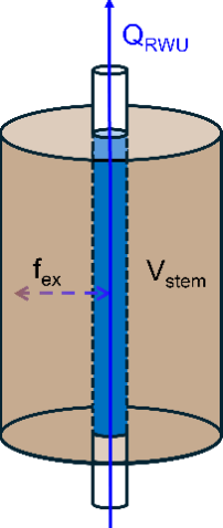
Figure B4C1. Graphical illustration of the stem water replacement model with xylem water.
