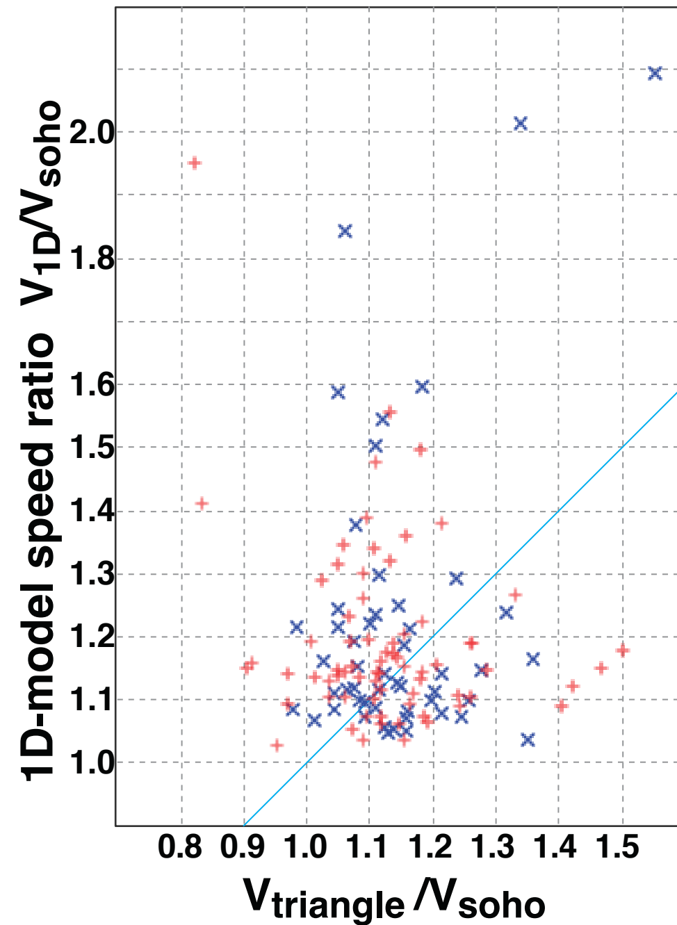
V_{\text{triangle}}/V_{\text{soho}} vs V_{1\text{D}}/V_{\text{soho}}
