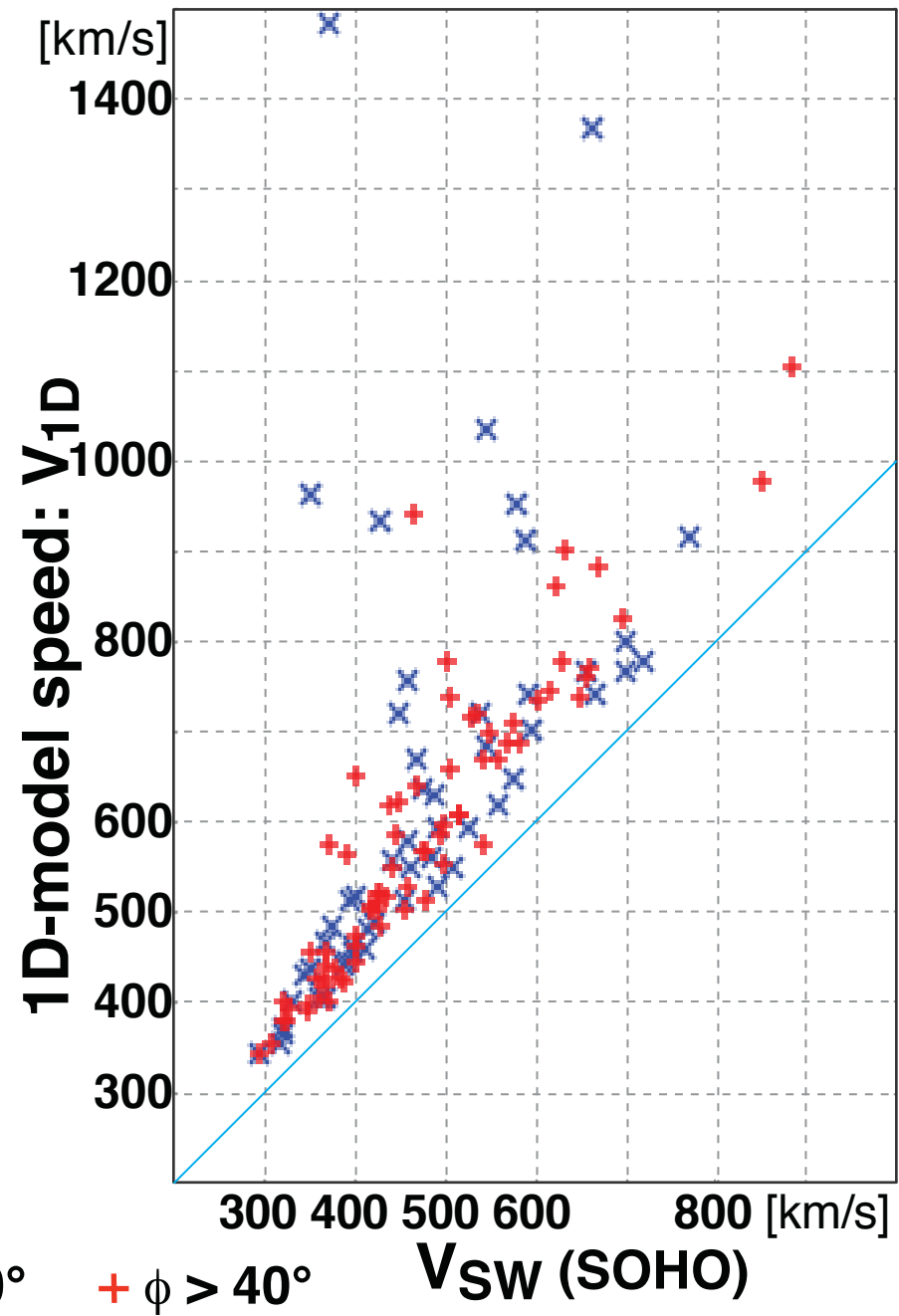
V_{1\text{D-model}} vs V_{\text{SW}}
