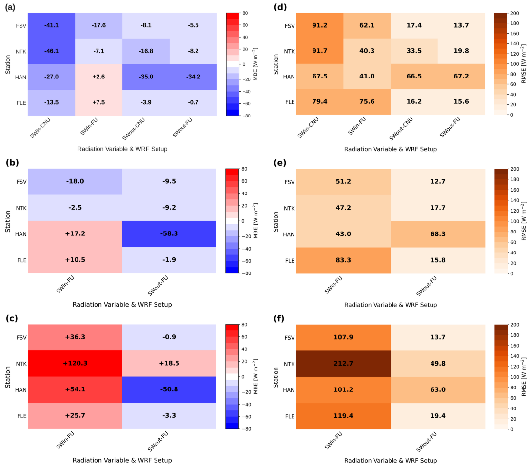
Figure 2. Summary Mean Bias Errors (MBE; a–c) and Root Mean Square Errors (RMSE; d–f) of short-wave incoming (SWin) and short-wave outgoing (SWout) radiation across 4 observational stations (FSV, NTK, HAN, and FLE) and different WRF driving data setups. Each cell contains the error averaged over the corresponding episode selection for a specific variable, observational station, and WRF model driving setup. Panels (a) and (d) correspond to the common simulated episodes driven by both CNU and FU WRF model setups, panels (b) and (e) refer to the clear-sky FU WRF model setup, while non-clear-sky episodes with the FU WRF model setup are depicted on panels (c) and (f). The colour bars represent the magnitude of the MBE and RMSE values in \text{W m}^{-2} .
