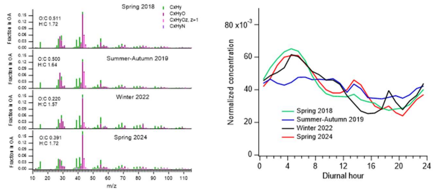
205 Figure 2: Mass spectra and average diurnal patterns of HOA (a), TrOA (b), and SV-OOA (c) from four campaigns. Concentrations in diurnal patterns were normalized to cumulative concentrations over the whole day.
