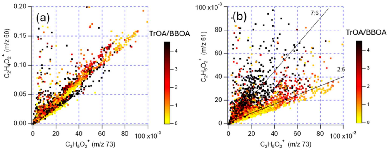
365 Figure 5: Scatter plots of C_2H_4O_2^+ and C_3H_5O_2^+ (a) and C_2H_5O_2^+ and C_3H_5O_2^+ (b) in the Winter 2022 data. The dots are colored according to the ratio of TrOA to BBOA.
