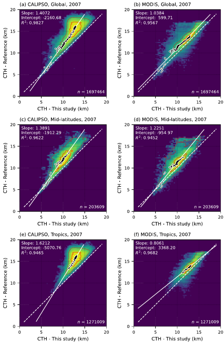
Figure 1. Cloud top height (CTH) estimated using the method developed in this study and reference data from CloudSat/CALIPSO (a, c, e) and MODIS (b, d, f) for the global domain excluding the polar regions (a, b), the mid-latitudes (c, d), and the tropics (e, f). Frequencies are shown on a logarithmic scale, with the solid red line enclosing 50% of all cases and the dashed red line enclosing 95% of cases. Black dots represent CTH averaged over 1° latitude bands to account for the significant latitudinal disproportions in DCC occurrence. The white line indicates the best linear fit (coefficients given in the top-left corner) to the zonally averaged CTH estimates ( R^2 applies to the zonally averaged means).
