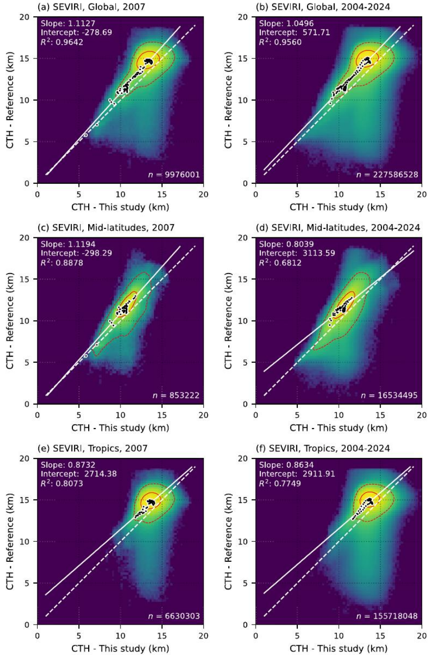
Figure 2. Cloud top height (CTH) estimated using the method developed in this study and reference data from SEVIRI CLAAS-3 dataset for year 2007 (a, c, e) and 2004-2024 (b, d, f) for the global domain excluding the polar regions (a, b), the mid-latitudes (c, d), and the tropics (e, f). Frequencies are shown on a logarithmic scale, with the solid red line enclosing 50% of all cases and the dashed red line enclosing 95% of cases. Black dots represent CTH averaged over 1^\circ latitude bands to account for the significant latitudinal disproportions in DCC occurrence. The white line indicates the best linear fit (coefficients given in the top-left corner) to the zonally averaged CTH estimates ( R^2 applies to the zonally averaged means).
