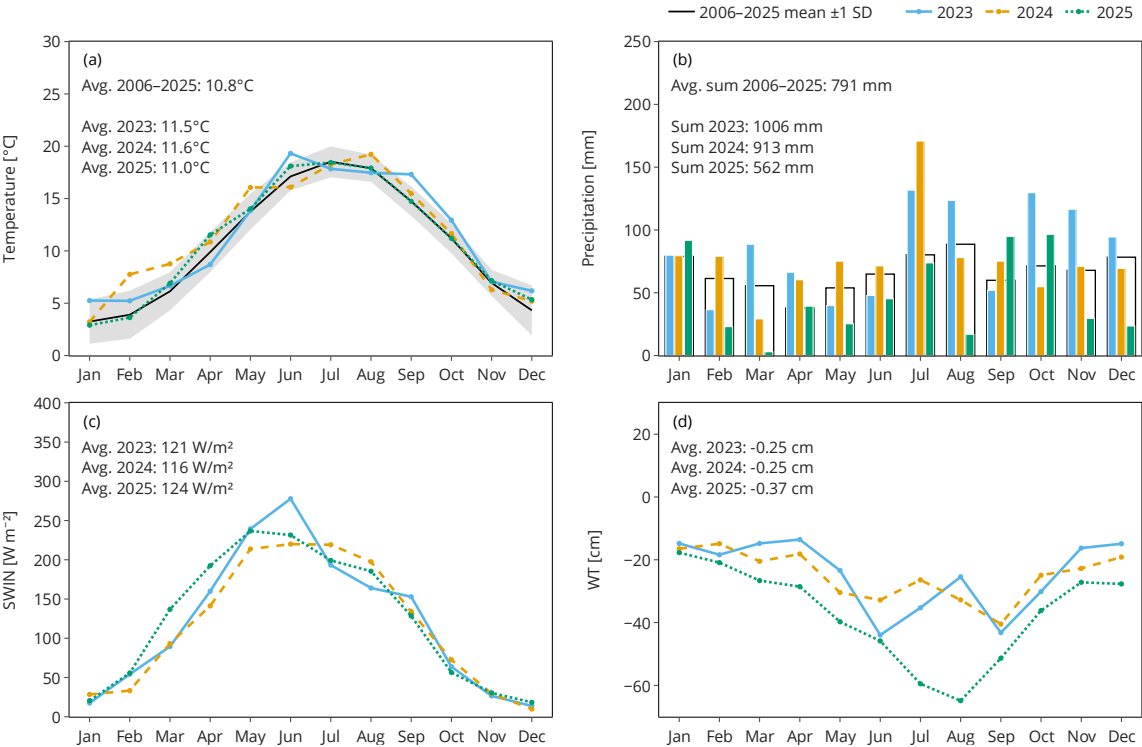
Figure 2: Monthly mean values of air temperature (TA), water table (WT), shortwave incoming radiation (SWIN) and sums of monthly precipitation (P) across the three measurement years. The grey band in (a) and the black background bar in (b) show the mean monthly and annual TA and P from 2006 until 2025. For SWIN and WT no comparable long-term measurements are available from any nearby source. Annotations show the annual means of TA (a), SWIN (c) and WT (d), the annual sums of P (b) and the long-term annual averages of TA (a) and P (b).
