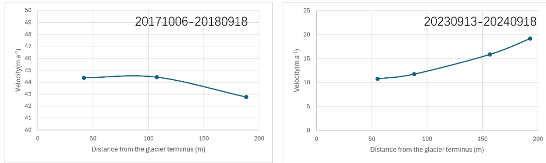
Figure 7 Near-terminus velocity gradients derived from manually tracked feature points along the glacier centerline.
