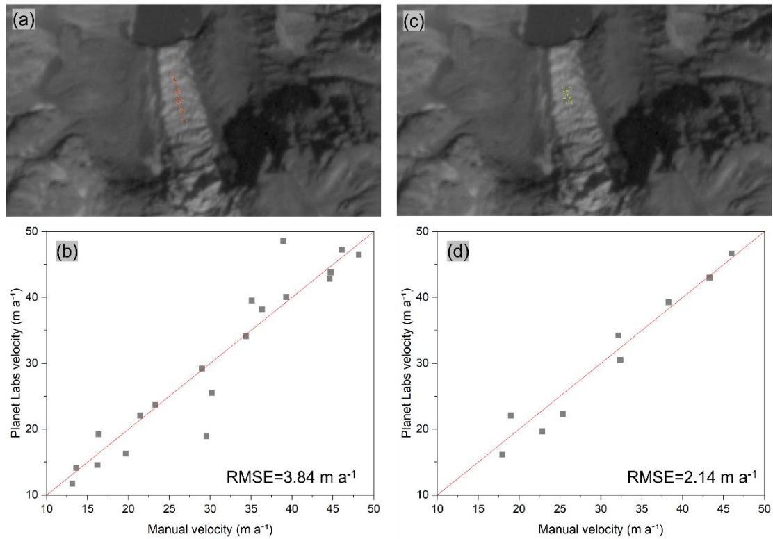
Figure 5 Validation of PlanetScope-derived ice velocities using manual feature tracking. (a, c) Locations of manually tracked surface features on the glacier tongue. (b, d) Comparison between manually measured velocities and PlanetScope-derived velocities.
