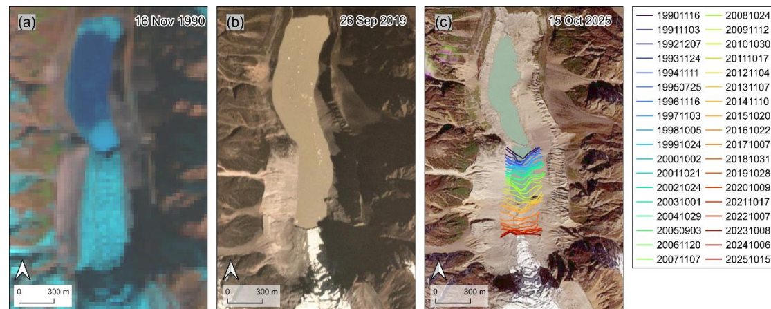
Figure 9 Multi-temporal evolution of the glacier terminal. (a) Landsat 5 TM imagery as the basemap acquired on 16 November 1990; (b–c) PlanetScope imagery as the basemap acquired on 26 September 2019 and 15 October 2025, respectively. Colored lines indicate glacier terminus positions mapped from satellite images between 1990 and 2025.
