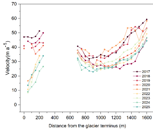
Figure 3 Longitudinal ice-velocity profiles along the centerline of Jinwu Glacier from 2017 to 2025. The x-axis indicates the distance from the glacier terminus. Different colored lines represent annual velocity profiles derived from PlanetScope feature tracking. Velocities were sampled along the glacier centerline at 50 m intervals.
