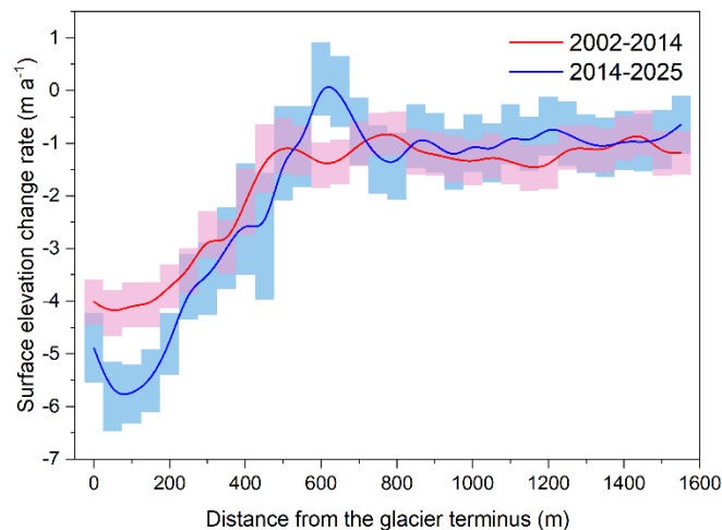
Figure 2 Surface elevation-change rates along the centerline of Jinwu Glacier during 2002–2014 and 2014–2025. The x-axis indicates the distance from the glacier terminus. Red and blue solid lines represent the mean surface elevation-change rates for 2002–2014 and 2014–2025, respectively. Shaded areas indicate the corresponding uncertainty ranges.
