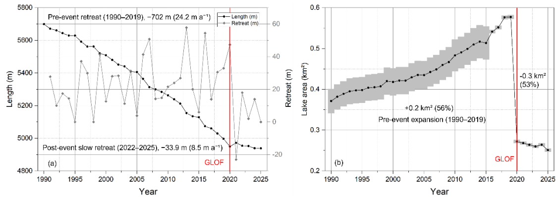
Figure 10 Changes in glacier terminus position and lake area during 1990–2025. (a) Glacier length and annual terminus retreat of Jinwu Glacier measured along the glacier centerline. (b) Lake area changes of Jinwu Glacier during 1990–2025. Black dots denote the mapped lake area for each year. The grey shading indicates the uncertainty of lake area.
