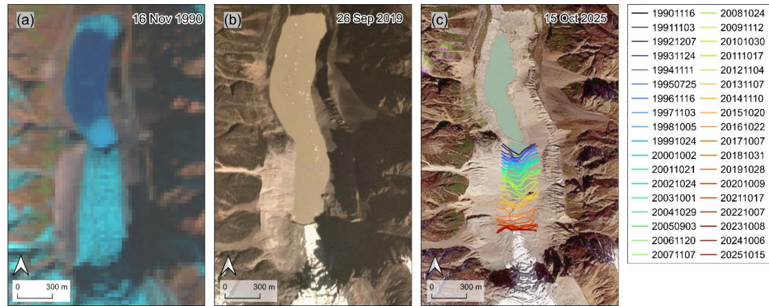
Figure 1 Multi-temporal evolution of the glacier terminal. (a) Landsat 5 TM imagery as the basemap acquired on 16 November 1990; (b–c) PlanetScope imagery as the basemap acquired on 26 September 2019 and 15 October 2025, respectively. Colored lines indicate glacier terminus positions mapped from satellite images between 1990 and 2025 .
