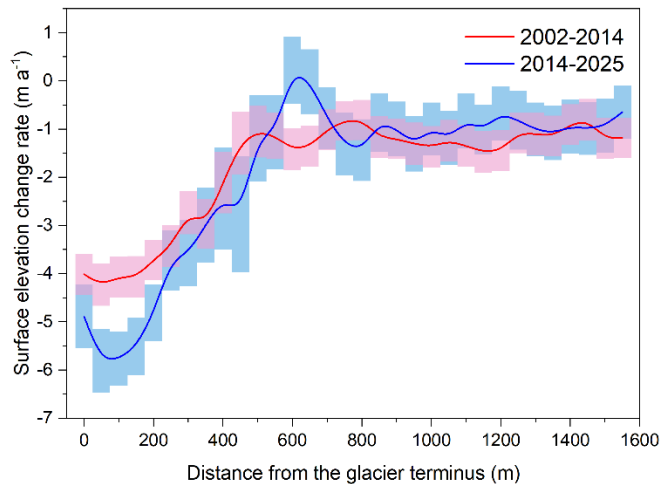
Figure 8 Surface elevation-change rates along the centerline of Jinwu Glacier during 2002–2014 and 2014–2025. The x-axis indicates the distance from the glacier terminus. Red and blue solid lines represent the mean surface elevation-change rates for 2002–2014 and 2014–2025, respectively. Shaded areas indicate the corresponding uncertainty ranges.
