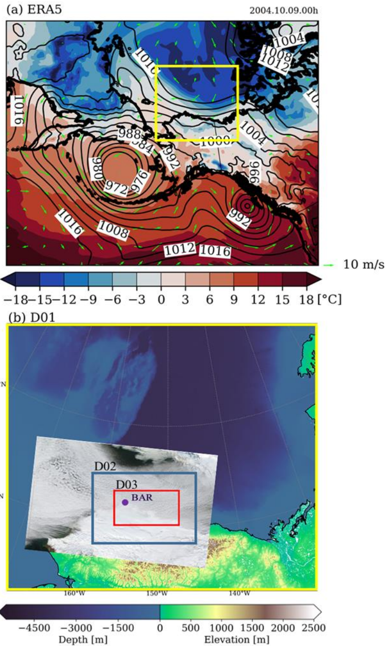
Figure 1: (a) ERA5 data showing sea level pressure (contours), 2-meter temperature (shading), and 10-m wind (vectors) at 00:00 UTC 9 October 2004. The yellow box indicates the WRF model domain (D01). (b) Nested model domains with D01 (18-km resolution), D02 (6-km resolution), and D03 (1-km resolution). Ocean depth and land elevation are shaded using the GEBCO_2023 grid (color bar at bottom), overlaid with the MODIS visible image at 00:00 UTC 9 October 2004 over the Arctic Ocean and northern Alaska.
