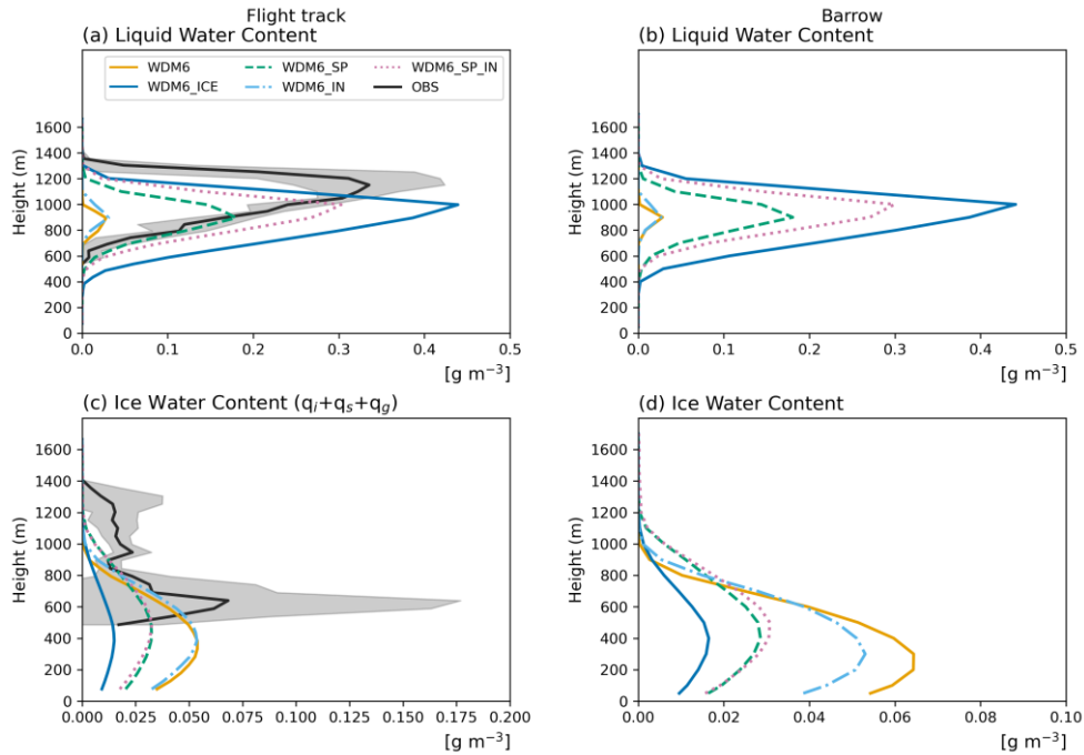
Figure 7: Vertical profiles of (a, b) LWC and (c, d) IWC. The left column (a, c) shows the profile over the flight region (red domain in Fig. 2a) during 01:00–02:00 UTC 10 October 2004, and the right column (b, d) shows the time-averaged (12:00 UTC 9 October – 11:00 UTC 10 October 2004) profile at BAR. Black lines with gray shading indicate observations ( \pm 1\sigma ), and colored lines represent sensitivity experiments: WDM6 (orange, solid), WDM6_ICE (blue, solid), WDM6_SP (bluish green, dashed), WDM6_IN (sky blue, dash-dot), and WDM6_SP_IN (purple, dotted).
