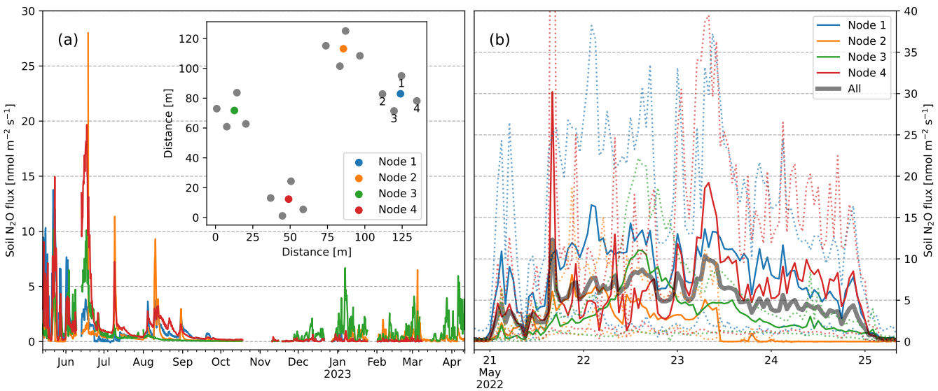
Figure 3. Time series of soil N 2 O flux (nmol m -2 s -1 ) measured from May 2022 to April 2023 using automated chambers deployed at four nodes in a conventionally tilled maize field near Villa Grove, Illinois. (a) Node-averaged fluxes at 6-hourly resolution showing the temporal and spatial variability, with distinct emission pulses during the early growing season. The inset shows the spatial arrangement of nodes and chambers within an area of ~5 ha. (b) Expanded view of 21–25 May 2022, highlighting the hourly flux variability. Solid lines represent node-averaged fluxes, dashed lines denote the minimum and maximum chamber values within each node, and the thick grey line represents the average across all nodes.
