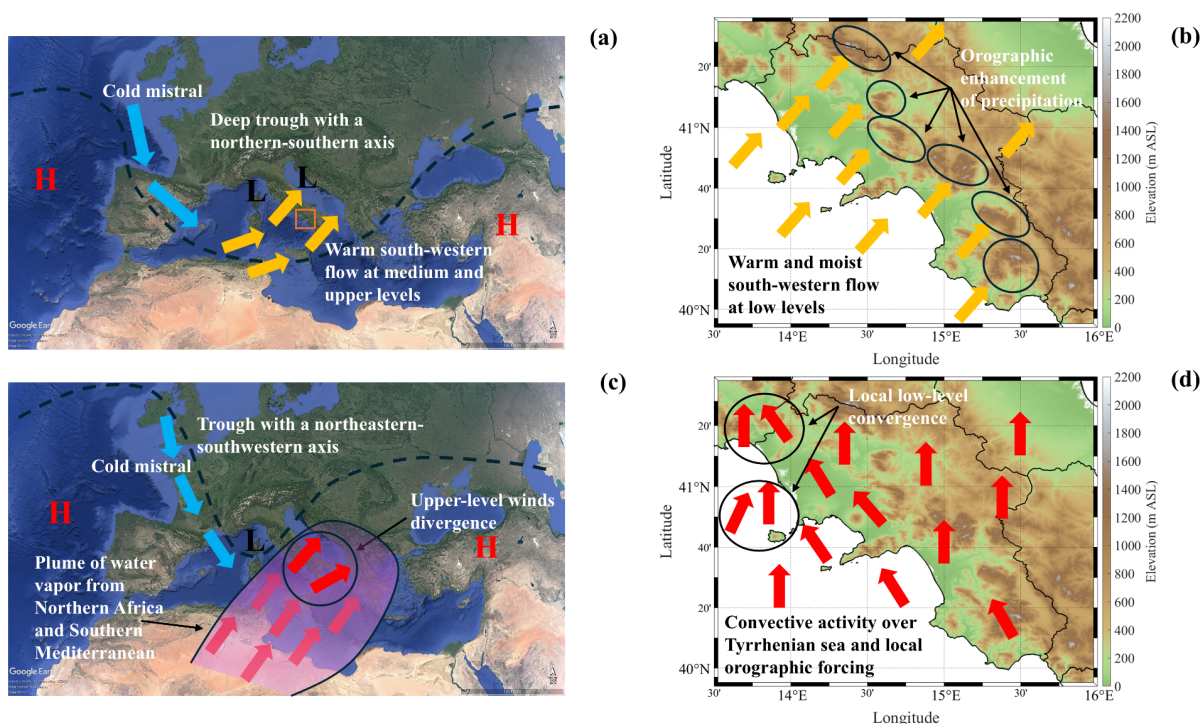
230 231 Figure 4: Schematic illustration of two of the six large-scale configurations associated with heavy-precipitation events in the 232 Campania Region (southern Italy) identified by Capozzi et al. (2023a). Panels (a)–(b) show Pattern 1 (warm and moist 233 southwesterly flow and orographic enhancement of precipitation along the main Apennine ranges); panels (c)–(d) represent 234 Pattern 6 (convective activity over the Tyrrhenian Sea and the northern sector under local low-level convergence). In (a) and 235 (c), the black dashed line marks the approximate position of the 552-dam 500-hPa geopotential-height contour, while the orange
