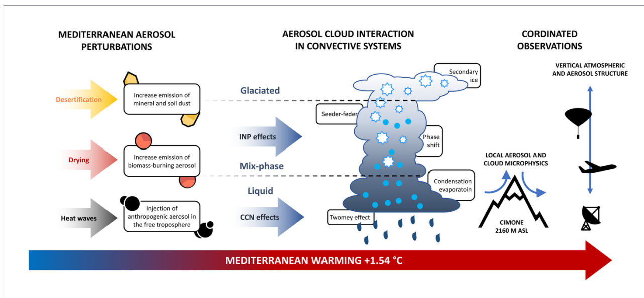
Figure 7. Schematic representing the aerosol cloud interactions (ACI) under the warming scenario in the Mediterranean. The cloud condensation nuclei (CCN) and ice nucleating particles (INPs) trigger different processes during severe storm development. To isolate the ACI contribution, observations of aerosol and cloud microphysics must be coordinated with vertically resolved dynamics observations.
