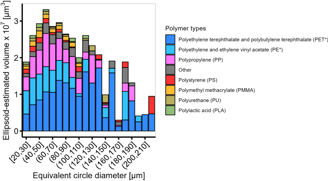
Figure 6. Particle volume size distribution including polymer type as estimated based on measured sizes of microplastic particles (n = 7150) detected in wet and dry deposition collected between May 2024 and May 2025 in Zurich (urban), Duebendorf (suburban), Magadino (rural), Payerne (rural) and Chaumont (mountainous), Switzerland. The polymer type "other" includes polyacrylonitrile, silicone, polyvinyl chloride, acrylonitrile butadiene styrene, ethylene vinyl alcohol, polyoxymethylene and polyether ether ketone.
