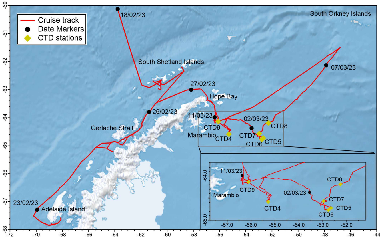
Figure 1. Map showing the cruise track in red along with date markers and the locations of the CTD samples discussed in this paper. The box shows an expanded view of the Weddell Sea.
