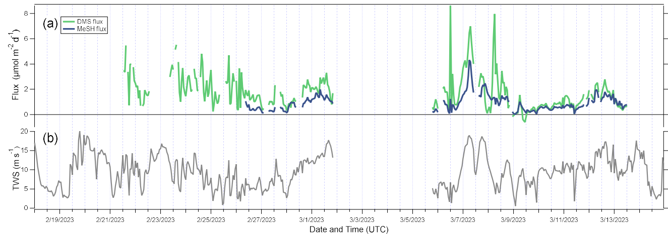
Figure 8. (a) Sea to air fluxes of DMS and MeSH, and (b) true wind speed (TWS, relative to ground).
