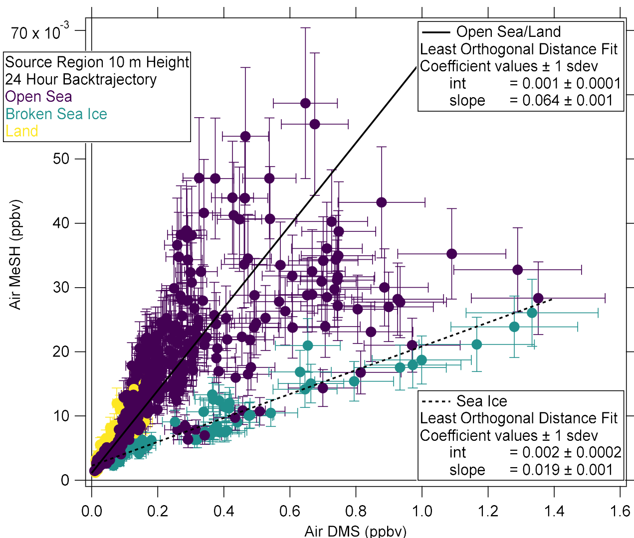
Figure 7. Scatter plot of the air concentration of MeSH vs the air concentration of DMS. Colour indicates 24 hour backtrajectory passing over open sea, sea ice (<50%) or land.
