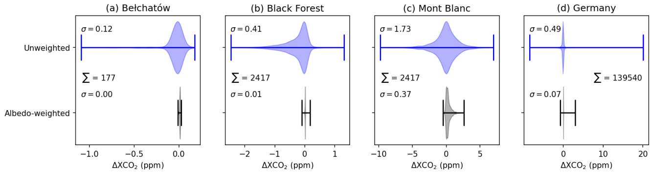
Figure 16. Variability of \Delta\text{XCO}_2 for the regions discussed in this section: (a) Bełchatów, (b) Black Forest, (c) Mont Blanc and (d) Germany. Note that the total number of data points differs largely between the panels. The \sigma values correspond to the standard deviations of the \text{XCO}_2 values (in ppm).
