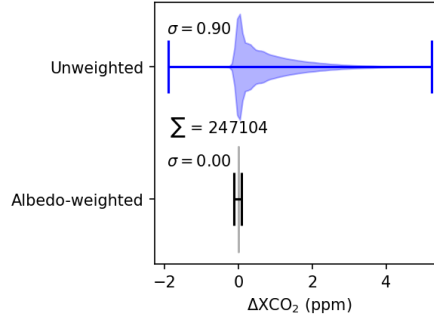
Figure 6. Differences of \Delta XCO_2 for all combinations of a spatial sample split into two parts, with one part z_{s,1} = 0 m and albedo of 0.001 in all fit windows, and the other part changing z_{s,2} between \{0, 8, \dots, 96\} m, spectral band albedos between \{0.001, 0.05, 0.1, 0.2, \dots, 1\} and fractions between \{0, 0.1, \dots, 1\} . The blue graph corresponds to the experiment with mean surface altitude and the black graph shows the experiment with albedo-weighted averaged surface altitude. The horizontal lines show minimum and maximum and the shaded ranges show the distribution of values. The total number of data points is 247104 ( 12^3 albedo, 13 altitude and 11 fraction values). The \sigma values correspond to the standard deviations of the \Delta XCO_2 values (in ppm).
