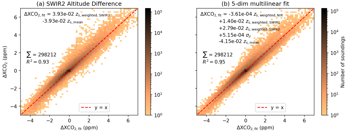
Figure 19. Two-dimensional histograms of the \text{XCO}_2 changes and fitting methods for all regions analyzed (see description in the text): (a) fitting linear regression of \Delta z_s in the SWIR2 band, and (b) fitting a linear combination of altitude changes, surface roughness and surface altitude. Only \Delta\text{XCO}_2 values between -5 and 7 ppm are shown. Note the \Delta\text{XCO}_{2,\text{fit}} corresponds to different fitting methods and also note the logarithmic color scale in each panel.
