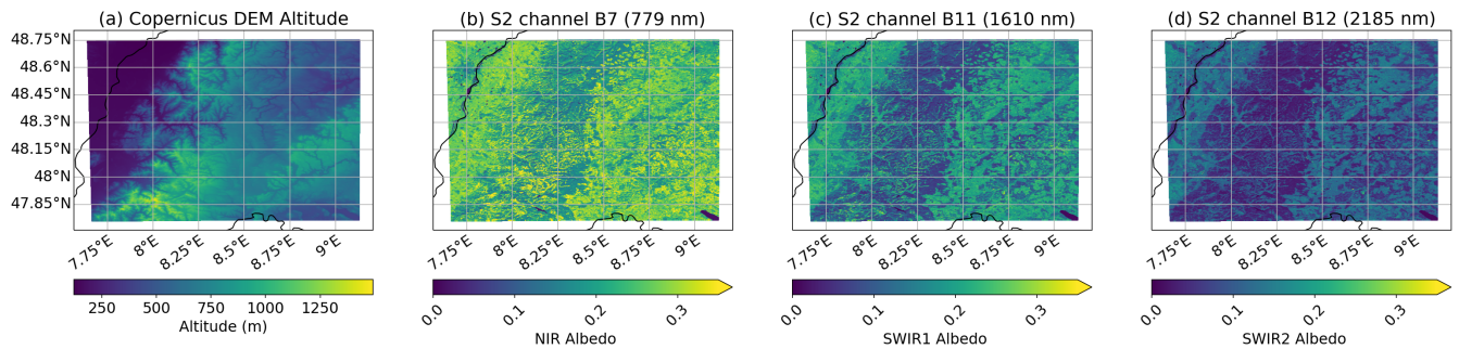
Figure 10. (a) Surface altitude by CopDEM and surface reflectance by S2 regrided to CopDEM grid points in the (b) NIR, (c) SWIR1 and (d) SWIR2 in the Black Forest.
