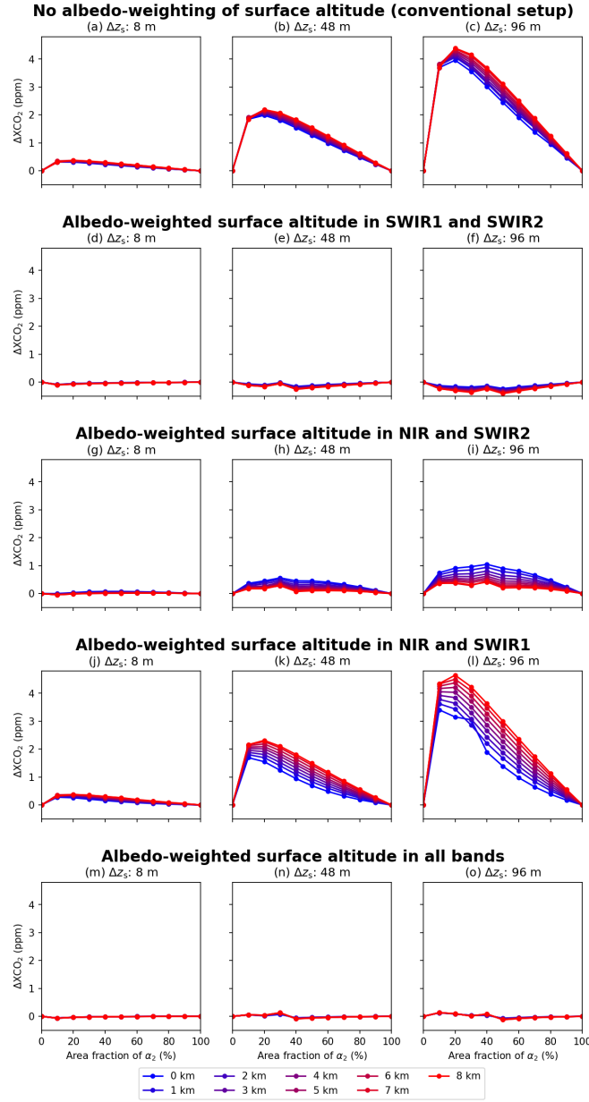
Figure 5. Similar to Fig. 4, but showing results with the VEG50 scenario in the second part of the spatial sample split into two, i.e. \alpha_{NIR,2} = 0.2 , \alpha_{SWIR1,2} = 0.1 , \alpha_{SWIR2,2} = 0.05 (ESA, 2020). Additional experiments where the average surface altitude is taken in only one of the three bands are shown (second to fourth row). In the other bands, the albedo-weighted average of the surface altitude is used. As in some of the panels the values are close to zero, we added the figures without shared y-axes in the supplementary material of this study (Fig. S3).
