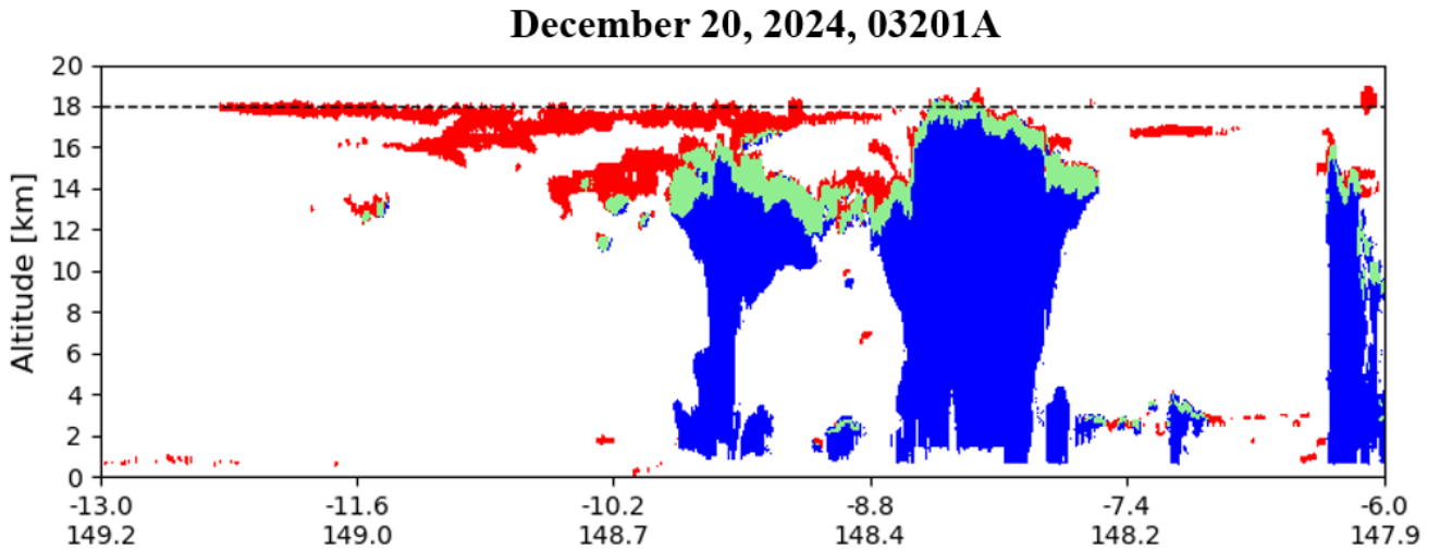
355 Figure 7: Cloud regions detected by CPR and ATLID for Frame 03201A acquired on December 20, 2024. Red, blue, and green indicate cloud regions detected by ATLID, CPR, and their overlap, respectively. The upper and lower ticks on the horizontal axis denote latitude and longitude, respectively. The dashed line indicates an altitude of 18 km.
