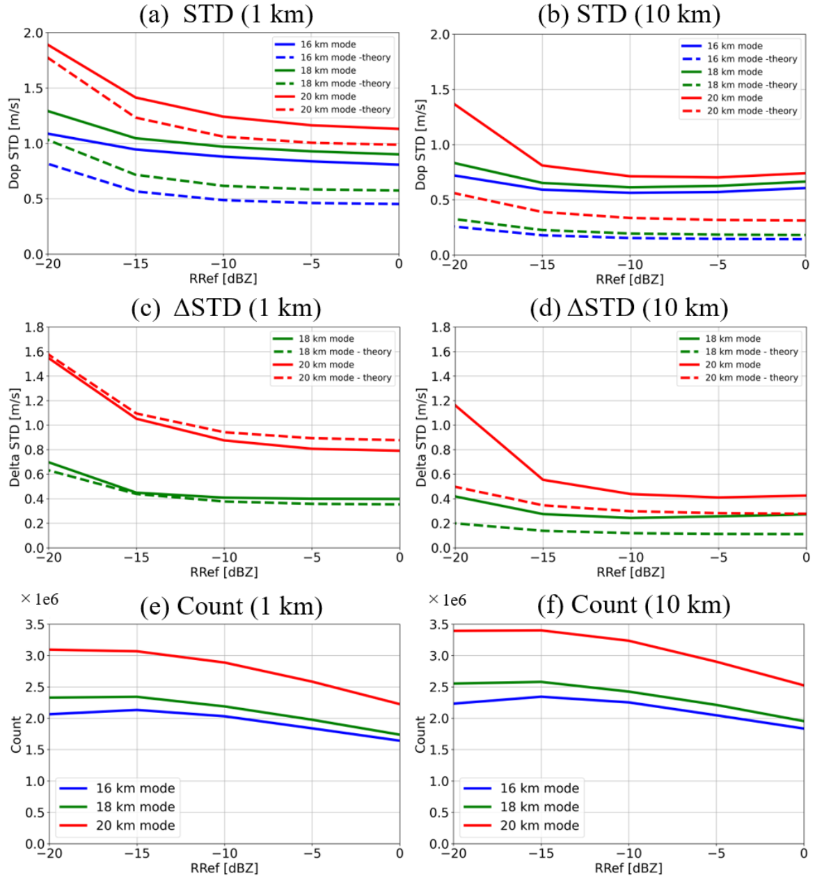
Figure 5: (a, b) STDs of Doppler velocity ( \text{m s}^{-1} ) as a function of radar reflectivity; (c, d) STD differences ( \text{m s}^{-1} ) of the 18-km and 20-km modes relative to the 16-km mode; and (e, f) sample counts for each radar reflectivity bin. The left and right panels correspond to the 1-km and 10-km integrations, respectively. The second row shows \Delta\text{STD} , defined as Eqs. (5) and (6), which represent the difference in random Doppler velocity uncertainty relative to the 16-km mode, removing the common contribution from natural variability. The 16-km, 18-km, and 20-km modes are indicated by blue, green, and red lines, respectively. In panels (a)–(d), the solid and dashed lines represent observed values and theoretical estimates, respectively. The observed data from 1–12 November 2024 were used, and the analysis region is limited to latitudes within 60^\circ and temperatures below 273 K. To ensure a consistent comparison among the modes, only clouds below 16 km were analyzed.
