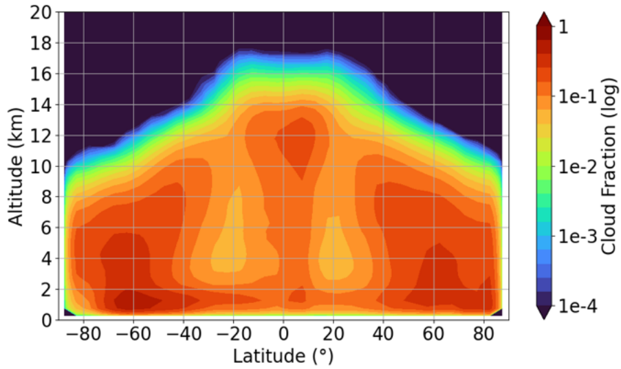
350 Figure 6: Zonal-mean cloud fraction derived from CPR observations, averaged over a one-year period from August 2024 to July 2025. Values are displayed on a logarithmic scale to highlight regions of low cloud fraction and to emphasize the presence of clouds at high altitudes. Clouds above the cloud-top heights detected by ATLID are excluded from this analysis.
