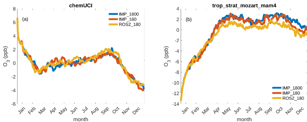
365 Figure 5. Daily global-mean surface-ozone anomaly (ppb), calculated by subtracting the annual-mean IMP_1800 surface-ozone value from each configuration, for (a) chemUCI and (b) trop_strat_mozart_mam4. Blue denotes IMP_1800, red denotes IMP_180, and dark yellow denotes ROS2_180.
