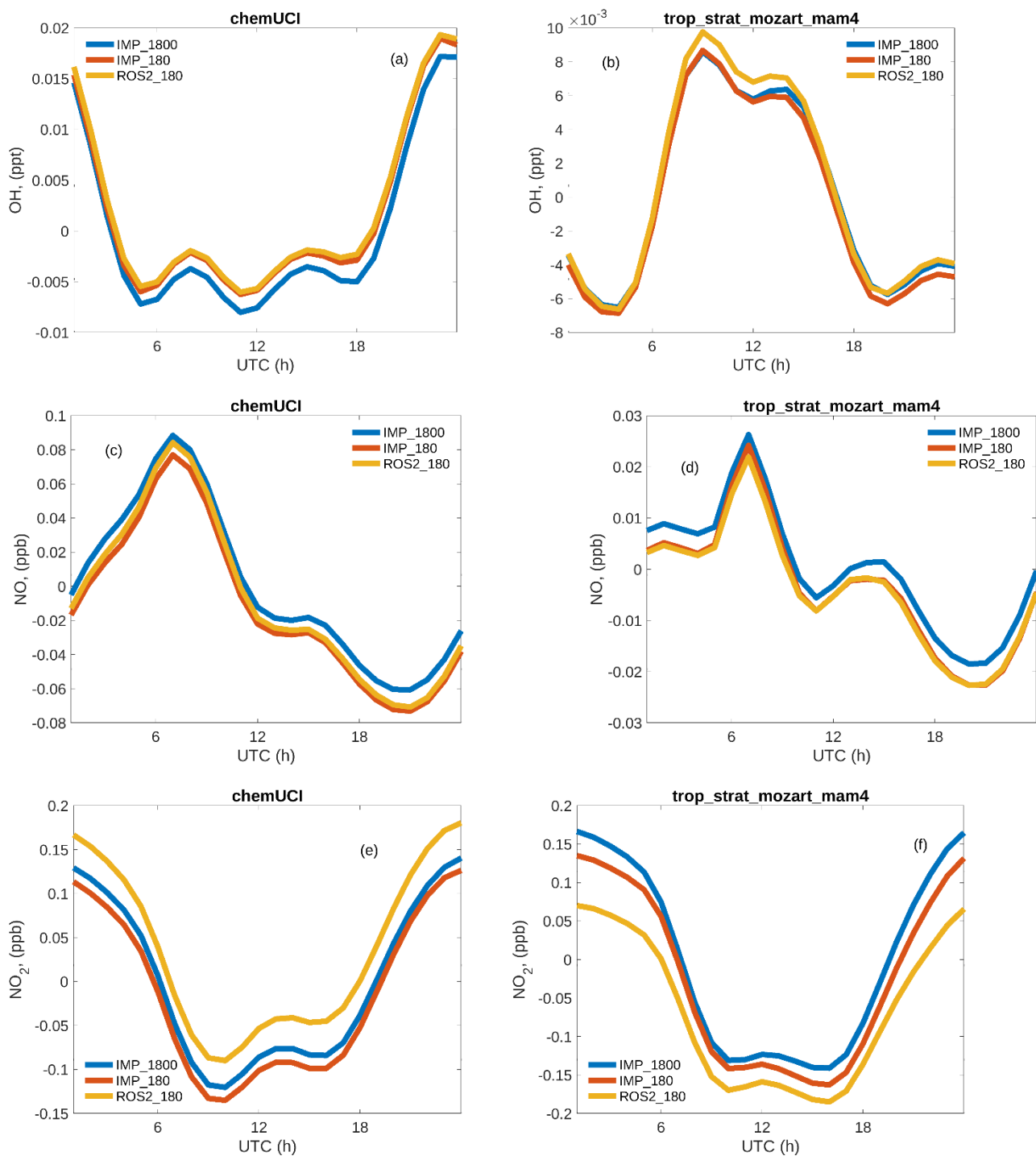
Figure 7. Global surface diurnal cycles of (a) \text{OH} , (c) \text{NO} , and (e) \text{NO}_2 using chemUCI and (b) \text{OH} , (d) \text{NO} , and (f) \text{NO}_2 using trop_strat_mozart_mam4. Blue denotes IMP_1800, red denotes IMP_180, and dark yellow denotes ROS2_180.
