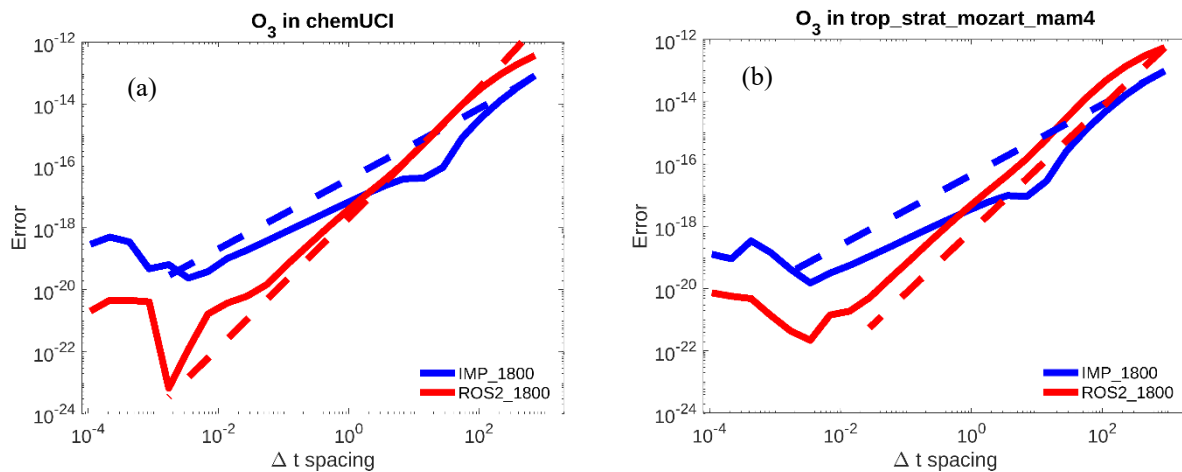
Figure 2. Timestep-refinement error estimate on log-log axes for (a) chemUCI and (b) trop_strat_mozart_mam4. Solid lines 350 show one representative grid column, and dashed lines show the mean fitted trend across 10,000 randomly sampled grid columns. Blue denotes the iterative implicit solver and red denotes ROS2. The fitted slopes are interpreted as empirical convergence-rate diagnostics, not as direct measurements of the formal solver order.
