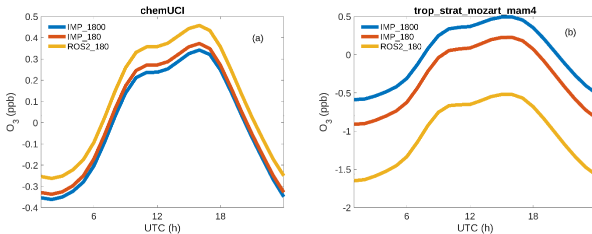
Figure 6. Global surface-ozone diurnal cycle for (a) chemUCI and (b) trop_strat_mozart_mam4. Blue denotes IMP_1800, red 370 denotes IMP_180, and dark yellow denotes ROS2_180. The curves are shown to compare temporal behavior and are not used as an absolute accuracy ranking.
