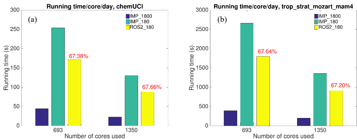
355 Figure 3. The running time for (a) chemUCI and (b) trop_strat_mozart_mam4. The dark blue is the iterative implicit solver with 1800s timestep (IMP_1800), and light green is IMP_180, and the yellow is the semi-implicit two-stage Rosenbrock solver with 180s timestep (ROS2_180) under 693 cores and 1350 cores. The efficiency of ROS2, expressed as a percentage, is shown for each number of cores and chemistry mechanism in red.
