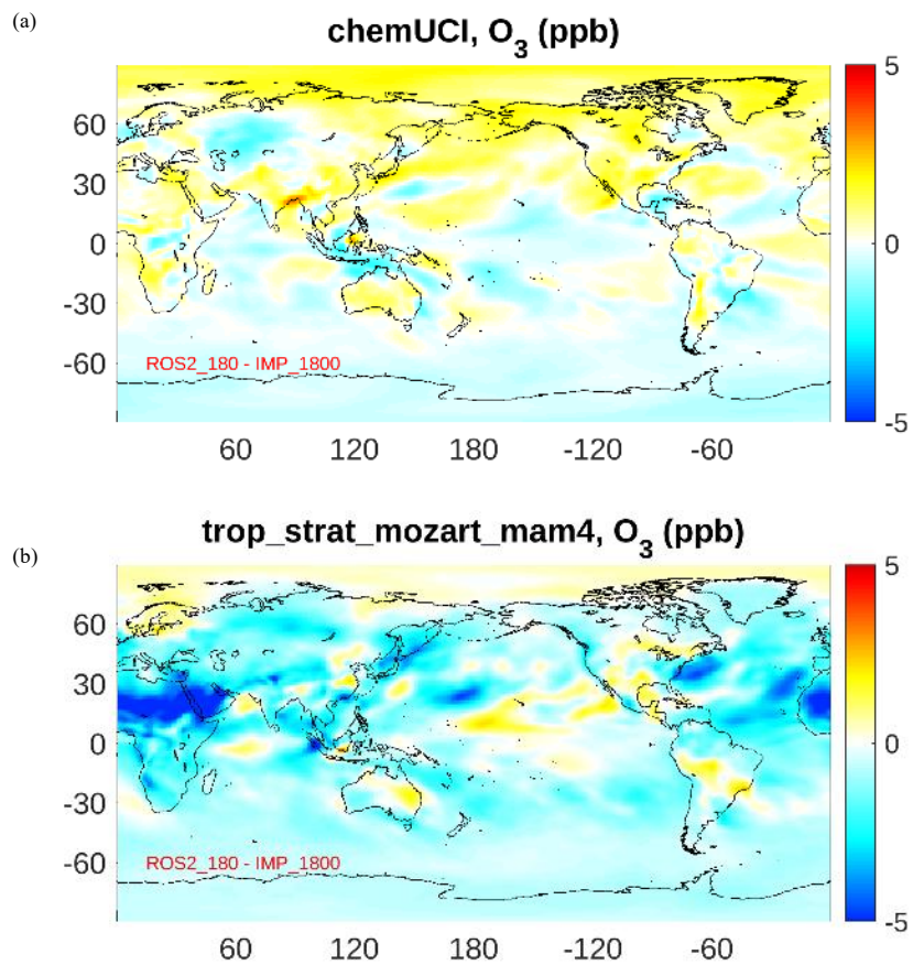
Figure 4. Global surface-ozone difference (ROS2_180 minus IMP_1800) for (a) chemUCI and (b) trop_strat_mozart_mam4.
