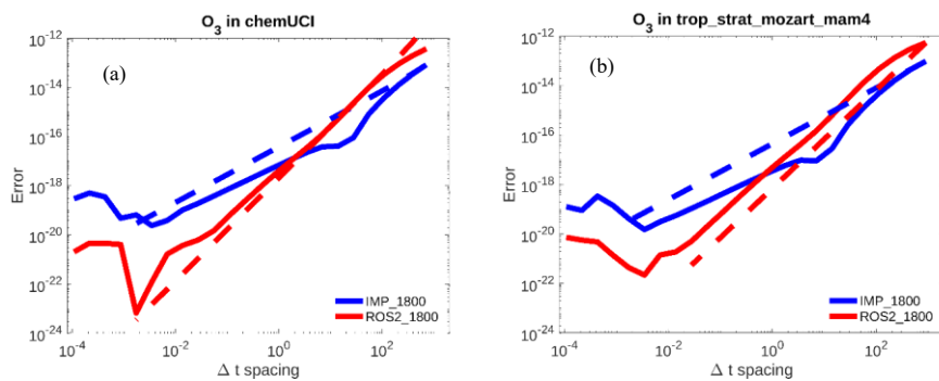
Figure 2. Timestep-refinement error estimate on log-log axes for (a) chemUCI and (b) trop_strat_mozart_mam4. Solid lines show one representative grid column, and dashed lines show the mean fitted trend across 10,000 randomly sampled grid columns. Blue denotes the iterative implicit solver and red denotes ROS2. The fitted slopes are interpreted as empirical convergence-rate diagnostics, not as direct measurements of the formal solver order.
