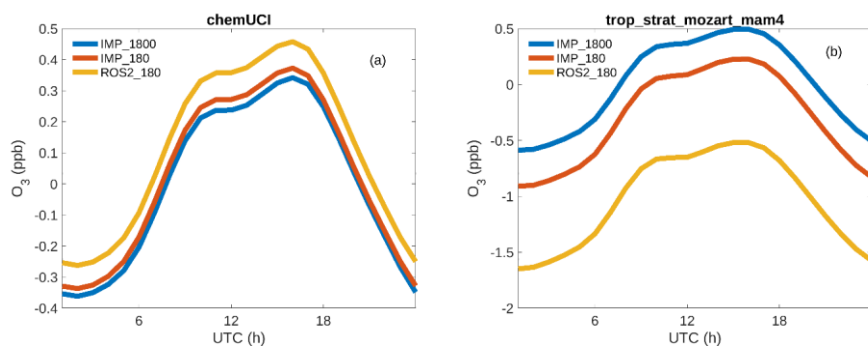
Figure 6. Global surface-ozone diurnal cycle for (a) chemUCI and (b) trop_strat_mozart_mam4. Blue denotes IMP_1800, red denotes IMP_180, and dark yellow denotes ROS2_180. The curves are shown to compare temporal behavior and are not used as an absolute accuracy ranking.
