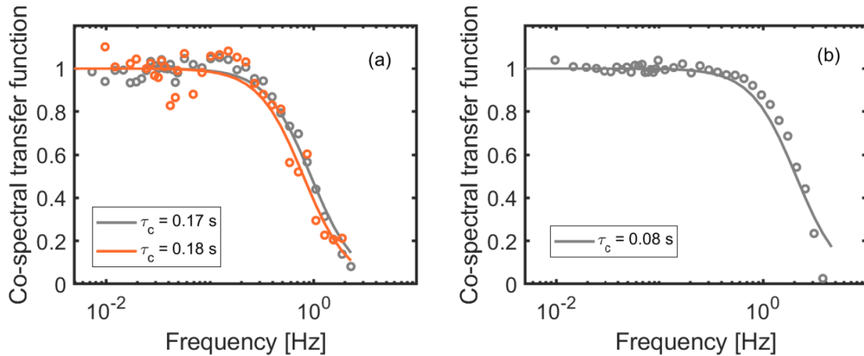
Figure 4: Frequency response functions estimated for (a) the prototype and (b) the reference systems. For transfer function estimation, unstable conditions were chosen (sensible heat flux > 25 \text{ W m}^{-2} ) with a limitation of wind speed from 2.5 to 3.5 \text{ m s}^{-1} . The period was taken from the beginning of measurements till the software update on 21 July 2022 (grey curves and symbols). For the prototype system, the response function was estimated also from 21 July (after the software update; orange) till 31 July 2022.
