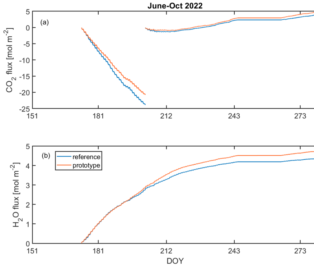
Figure 9: Cumulative fluxes for \text{CO}_2 (a) and \text{H}_2\text{O} (b) measured by the reference (blue) and the prototype (orange) systems. For \text{CO}_2 , the cumulative value is reset to zero on 21 July 2022 (doy 202.4) due to a major software update. Cumulative curves were calculated over the periods when measurements from both systems were available; no gap-filling was done.
