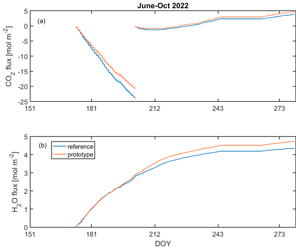
Figure 9: Cumulative fluxes for CO 2 (a) and H 2 O (b) measured by the reference (blue) and the prototype (orange) systems. For CO 2 , the cumulative value is reset to zero on 21 July 2022 (doy 202.4) due to a major software update. Cumulative curves were calculated over the periods when measurements from both systems were available; no gap-filling was done.
