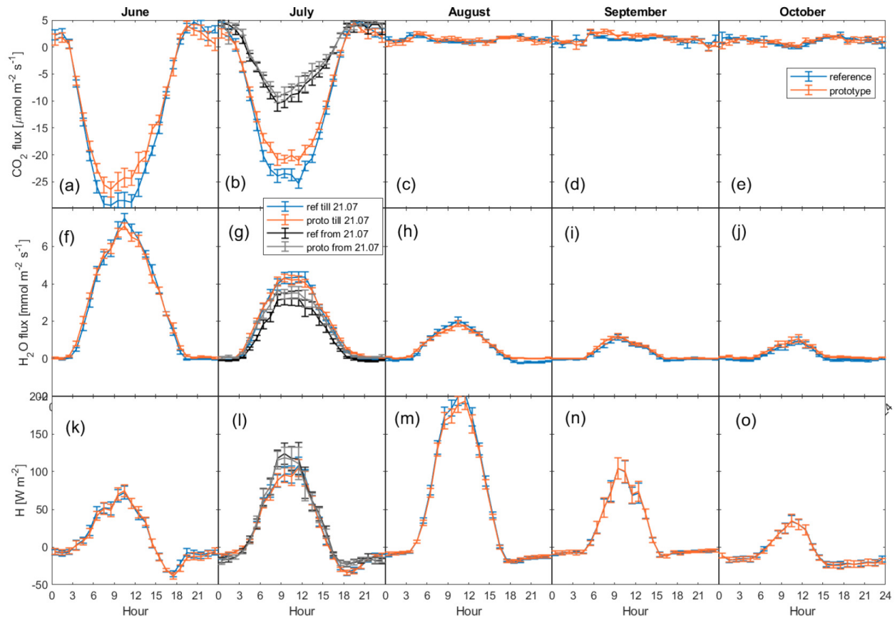
Figure 8: Monthly mean diurnal variation for CO 2 (a-e), H 2 O (f-j) and sensible heat H (k-o) fluxes. In July (b, g, l), the period after the software update on 21 July 2022 is differentiated by black for the reference and grey for the prototype system. The error bars represent 1 standard error of the hourly bin averages. The magnitude of the fluxes after 21 July is significantly lower for CO 2 (b) due to decline in carbon assimilation rates towards the end of the month.
