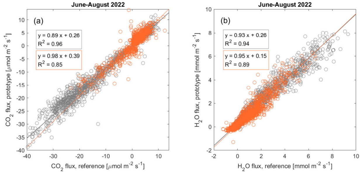
Figure 7: Comparison of 30 min average fluxes (a – \text{CO}_2 , b – \text{H}_2\text{O} ) of the prototype system with the reference system. The fitting parameters were obtained by using the orthogonal regression method. Grey and orange colours represent the measurements (and regressions statistics in respective bounding boxes) prior to and after the software update on 21 July 2022, respectively.
