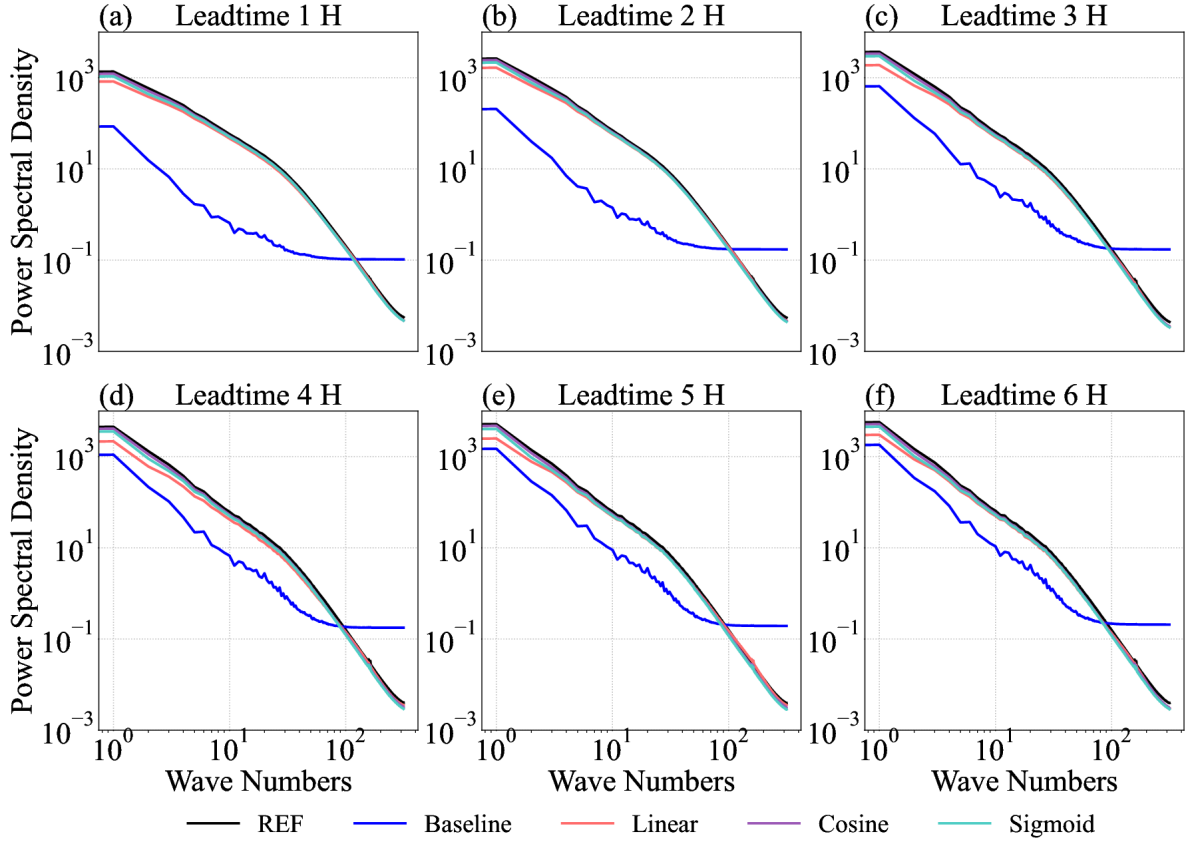
235 Fig. 4. Comparison of power spectra density for Errors in different forecast lead time. The black and blue solid lines denote the errors of deterministic nowcast (REF) and baseline, respectively. While the orange, purple and teal solid lines denote DDPM predictions with different noising schedule (Linear, Cosine and Sigmoid).
