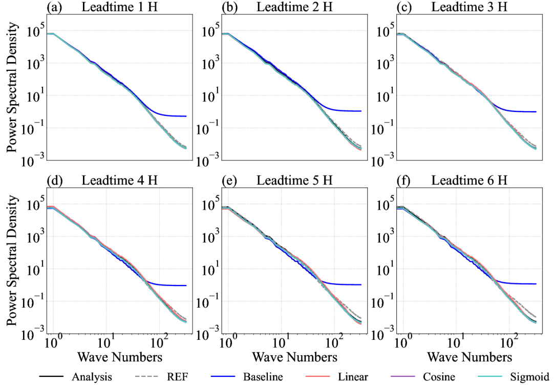
Fig. 5. Comparison of power spectra density for wind speed nowcasts in different forecast lead time. The black solid lines are the analysis field (Analysis) and the grey dashed lines and blue solid lines denote deterministic nowcast (REF) and baseline, respectively. While the orange, purple and teal solid lines denote DDPM ensemble nowcasts with different noising schedule (Linear, Cosine and Sigmoid).
