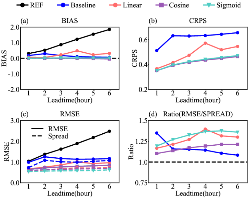
Fig. 6. Verification metrics for deterministic and ensemble mean nowcasts over the test period. (a) BIAS, (b) CRPS, (c) RMSE (solid lines) and ensemble spread (dashed lines). (d) Ratio of RMSE to SPREAD. In all panels, the black solid line denotes the deterministic nowcast (REF), the blue line represents the ensemble nowcasts from the climatological baseline, while the orange, purple, and teal lines correspond to the three DDPM noising schedules (Linear, Cosine, and Sigmoid), respectively.
