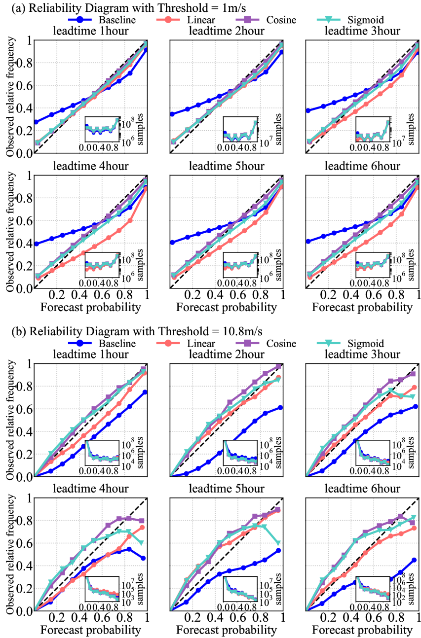
Fig. 10. Probability diagram of wind ensemble nowcasting in different lead time for the four schedules with threshold 1 \text{ m s}^{-1} (a) and 10.8 \text{ m s}^{-1} (b). The inset in each subplot denotes the corresponding statistics samples.
