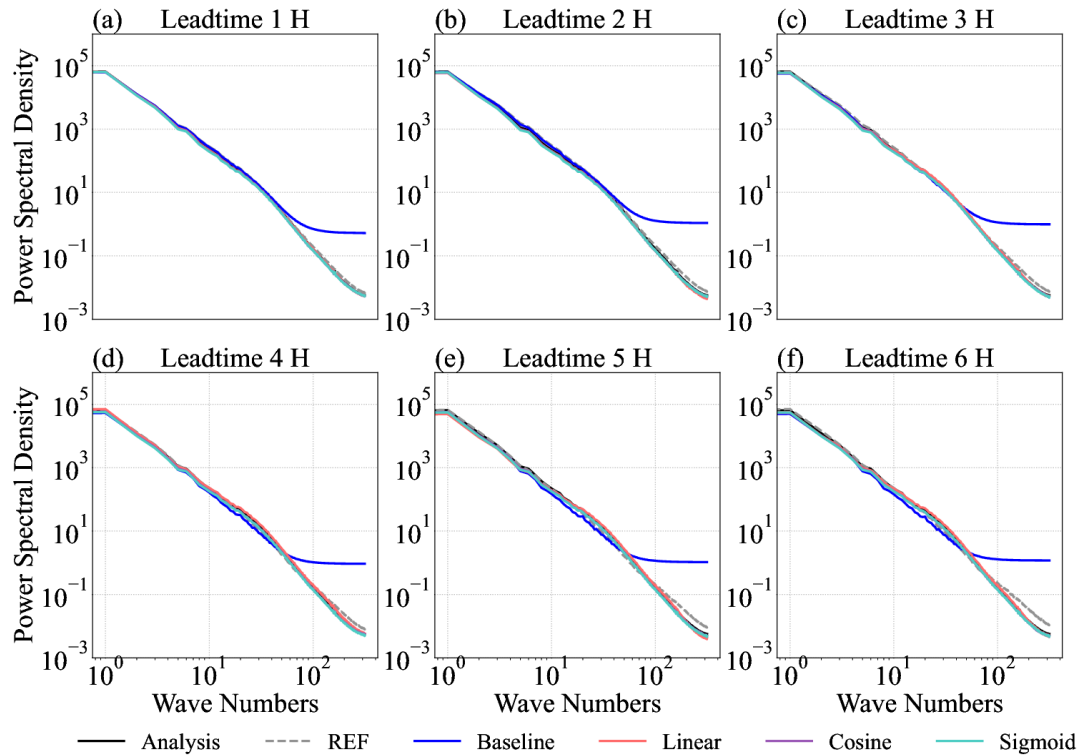
Fig. 5. Comparison of power spectra density for wind speed nowcasts in different forecast lead time. The black solid lines are the analysis field ( Analysis ) and the grey dashed lines and blue solid lines denote deterministic nowcast (REF) and baseline, respectively. While the orange, purple and teal solid lines denote DDPM ensemble nowcasts with different noising schedule (Linear, Cosine and Sigmoid).
