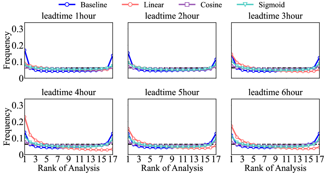
Fig. 9. Talagrand Diagrams of wind ensemble nowcasts for different ensembles.
