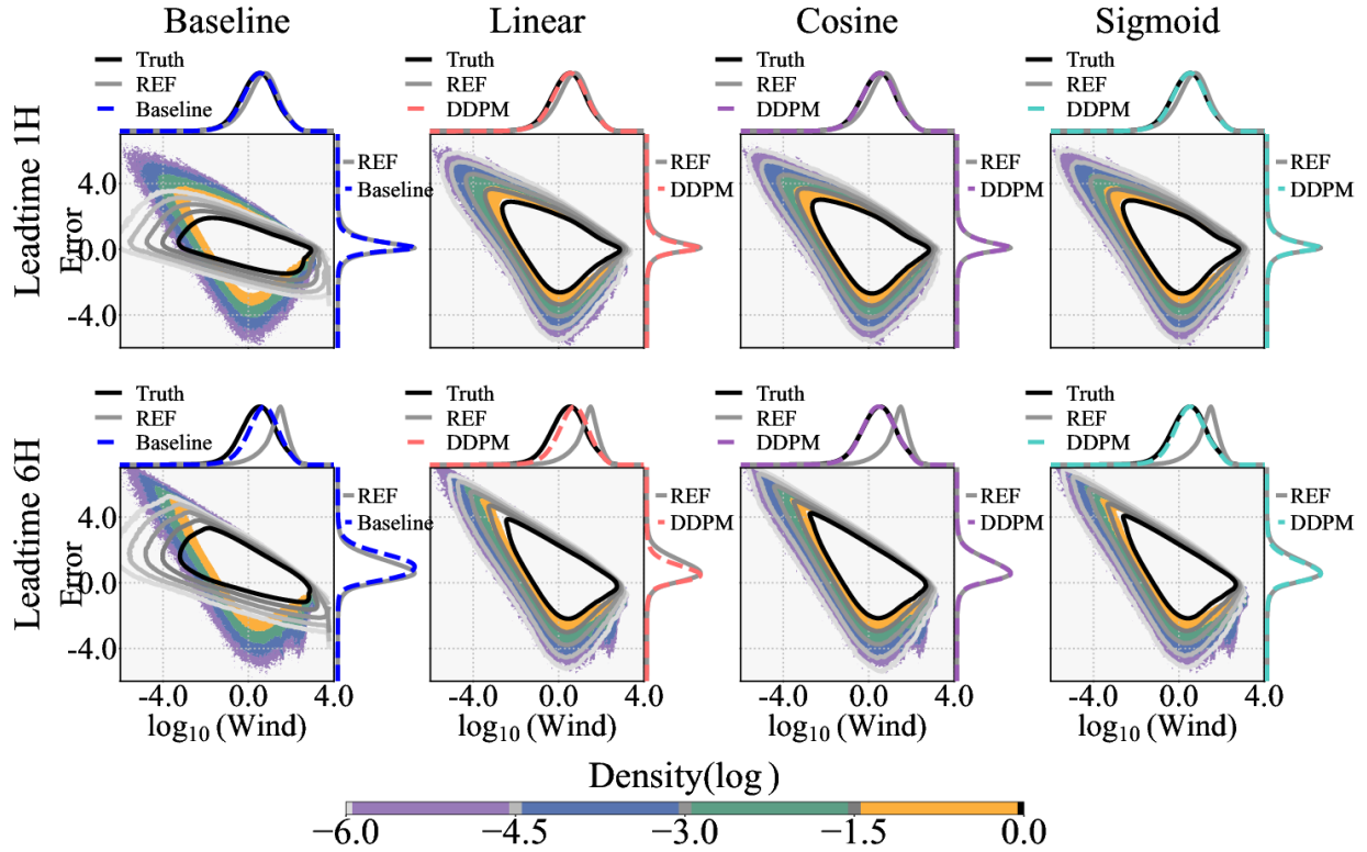
Fig. 3. Joint distribution of error and wind speed for the 1-hour (top row) and 6-hour (bottom row) forecast. The shaded contours and contour lines represent the deterministic reference (REF) and ensemble predictions of baseline or DDPM, respectively. Marginal distributions of logarithmic wind speed (top x axis) and error (right y axis) are shown for observations (Truth, black solid), the deterministic forecast (REF, grey solid), and the DDPM ensemble (dashed).
