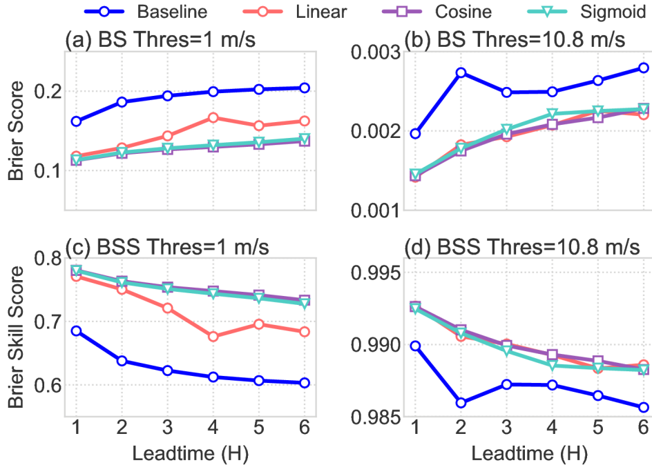
Fig. 8. Brier Score (BS) and Brier Skill Score (BSS) of the wind speed ensemble nowcasts as a function of forecast lead time for two wind speed thresholds. (a, c) Threshold: 1 m s -1 . (b, d) Threshold: 10.8 m s -1 . In all panels, results are shown for the climatological baseline (blue) and the three DDPM noising schedules: Linear (orange), Cosine (purple), and Sigmoid (teal).
