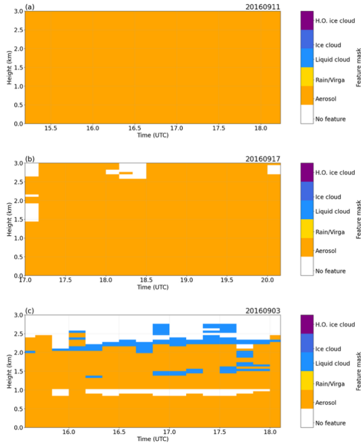
Figure C. Feature mask from Raman Lidar on (a) September 11, 2016 (case #1), (b) September 17, 2016 (case #2), and (c) September 3, 2016 (case #3).
