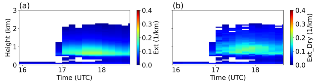
Figure D2. Time–height cross sections of Raman-lidar aerosol extinction for Case (10 September 2016). (a) Lidar extinction coefficient (Ext, km -1 ). (b) Dry-corrected aerosol extinction coefficient (Ext_Dry, km -1 ) directly used in the RNCCN.
