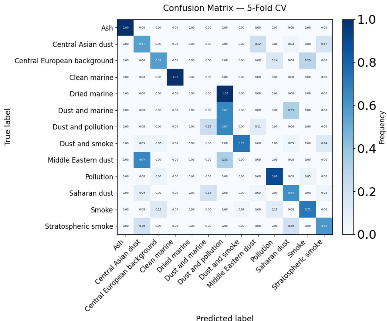
Figure B. Row-normalized confusion matrix from 5-fold stratified cross-validation. Each row represents the true aerosol class, and each column shows the predicted class. Values on the diagonal represent the accuracy for each class, while off-diagonal values indicate misclassifications.
