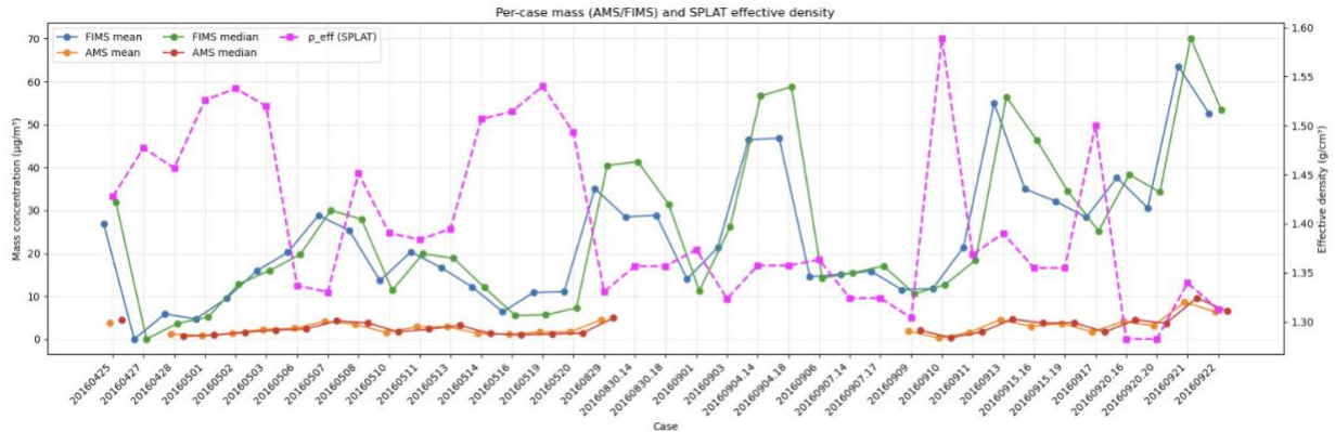
Figure A. Per-case aerosol mass derived from the Fast Integrated Mobility Spectrometer (FIMS) and the Aerosol Mass Spectrometer (AMS), together with Single Particle Lagrangian Integrated Trajectory (SPLAT)–derived effective particle density ( \rho_{\text{eff}} ). FIMS aerosol mass (mean and median) is estimated from measured aerosol size distributions using the case-specific effective density ( \rho_{\text{eff}} ), while AMS mass represents non-refractory submicron aerosol species, including sulfate ( \text{SO}_4^{2-} ), nitrate ( \text{NO}_3^- ), ammonium ( \text{NH}_4^+ ), chloride ( \text{Cl}^- ), and organic aerosol (Org).
