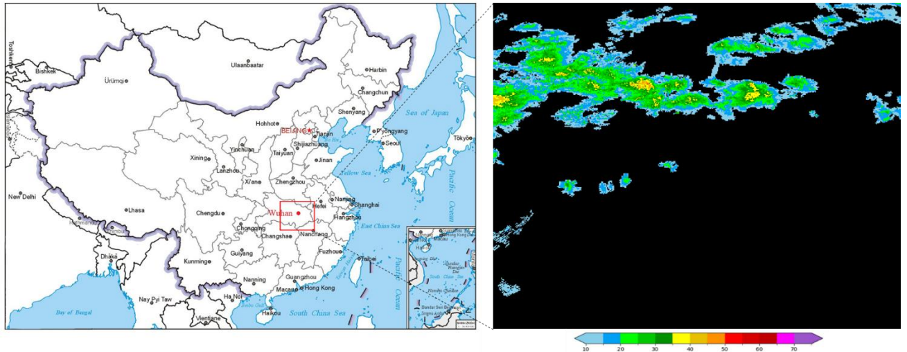
Figure 1 Study area (left) and an example of radar mosaic reflectivity (right).
