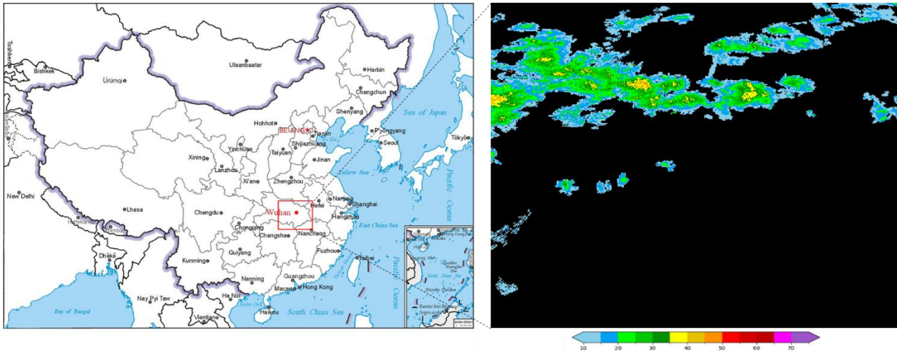
96 97 Figure 1 Study area (left) and an example of radar mosaic reflectivity (right).
