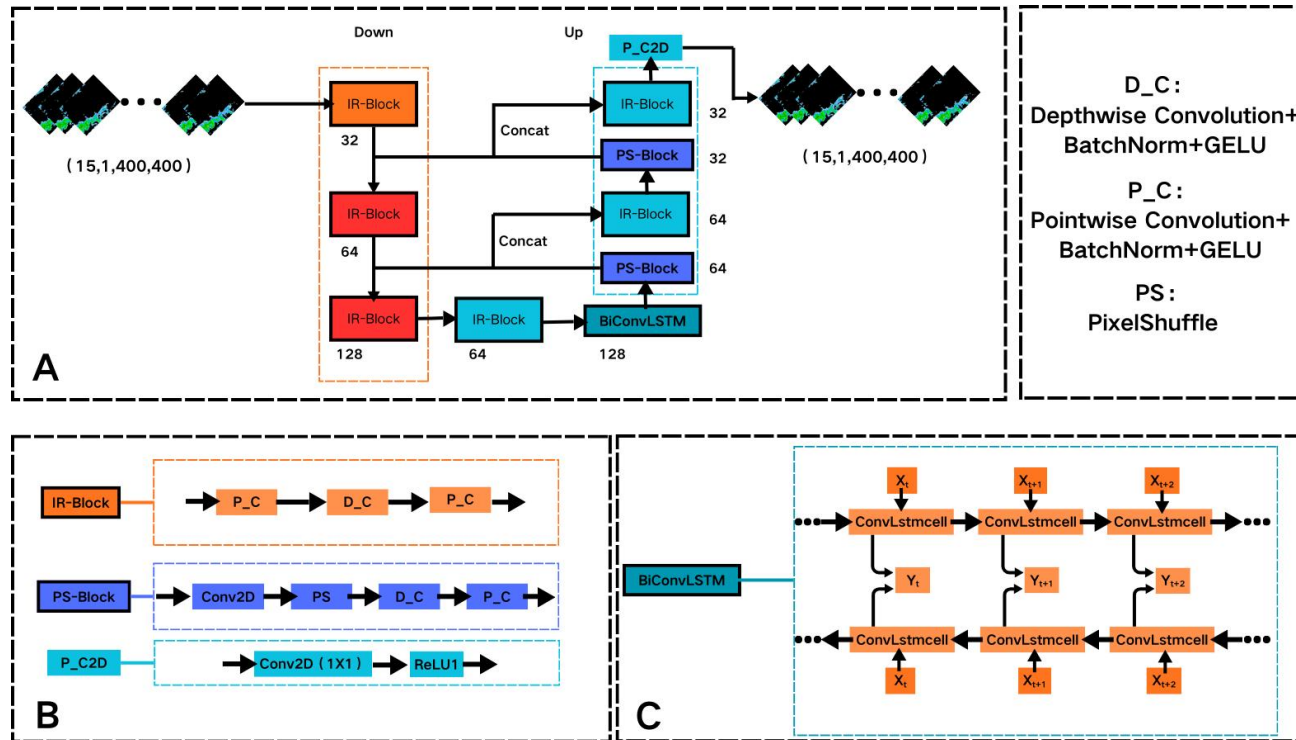
Figure 4 Structure diagram of the BiConvLSTM-UNet model
