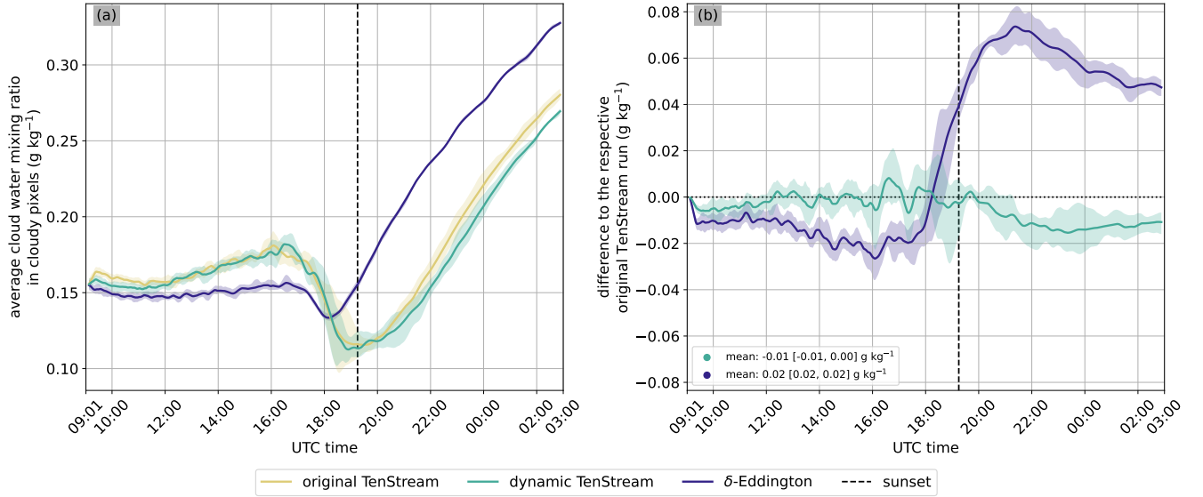
Figure 5. Temporal evolution of the average cloud water mixing ratio q_c in cloudy pixels (a) and differences relative to the corresponding TenStream reference run (b). The As in Fig. 4, the colored lines show the ensemble mean for each radiative transfer solver, while the shaded areas indicate one-standard-deviation across the corresponding five-member ensemble spreads. The legend in panel (b) provides temporal mean differences and their standard deviations minimum-to-maximum ranges. By isolating changes in in-cloud condensate from changes in cloud depth, this plot complements Fig. 4 (b). As in this preceding figure, the vertical line marks the time of sunset, and a 15-minute running mean was applied to the data before plotting.
