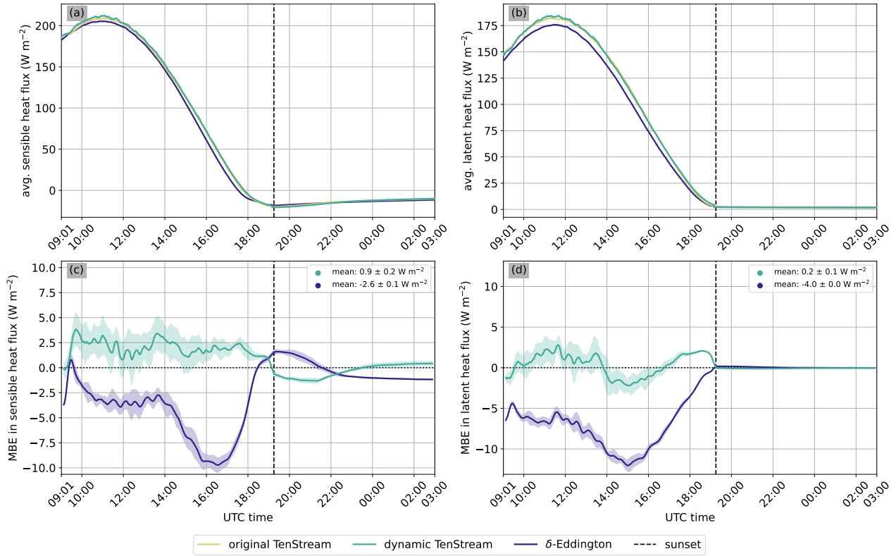
Figure 10. Temporal evolution of the domain-averaged sensible (a) and latent (b) heat fluxes for all six simulations considered the three five-member ensembles discussed in this evaluation paper . Panels (c) and (d) show the corresponding differences relative to the respective TenStream reference run . In all panels, with temporal the colored lines show the ensemble mean differences for each radiative transfer solver, while the simulations coupled to shaded areas indicate one standard deviation across the different solvers listed in the corresponding five-member ensemble. The legends (values for the control runs are provided in brackets) panels (c) and (d) provide temporal mean differences and their standard deviations . To improve readability, a 15-minute running mean was applied to the data in panels (c) and (d) before plotting . The vertical line in each plot panel marks the time of sunset.
