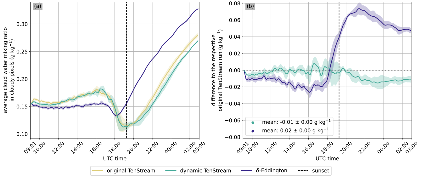
Figure 5. Temporal evolution of the average cloud water mixing ratio q_c in cloudy pixels (a) and differences relative to the corresponding TenStream reference run (b). The colored lines show the ensemble mean for all six (five in panel (b)) PALM simulations considered in this evaluation each radiative transfer solver, while the shaded areas indicate one standard deviation across the corresponding five-member ensemble. The legend in panel (b) provides temporal mean values, with the numbers for the corresponding control runs given in brackets differences and their standard deviations. By isolating changes in in-cloud condensate from changes in cloud depth, this plot complements Fig. 4 (b). As in this preceding figure, the vertical line marks the time of sunset, and a 15-minute running mean was applied to the data before plotting.
