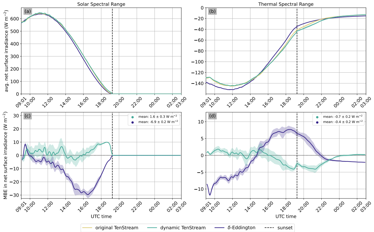
Figure 9. Temporal evolution of the domain-averaged net surface irradiance in the solar (a) and thermal (b) spectral ranges for the six simulations considered three five-member ensembles discussed in this evaluation paper. Panels (c) and (d) show the corresponding differences relative to the respective TenStream reference run. In all panels, with temporal the colored lines show the ensemble mean differences for each radiative transfer solver, while the simulations coupled to shaded areas indicate one standard deviation across the different solvers listed in the corresponding five-member ensemble. The legends (values for the control runs are given in brackets) panels (c) and (d) provide temporal mean differences and their standard deviations. To improve readability, a 15-minute running mean was applied to the data in panels (c) and (d) before plotting. The vertical line in each plot indicates panel marks the time of sunset.
