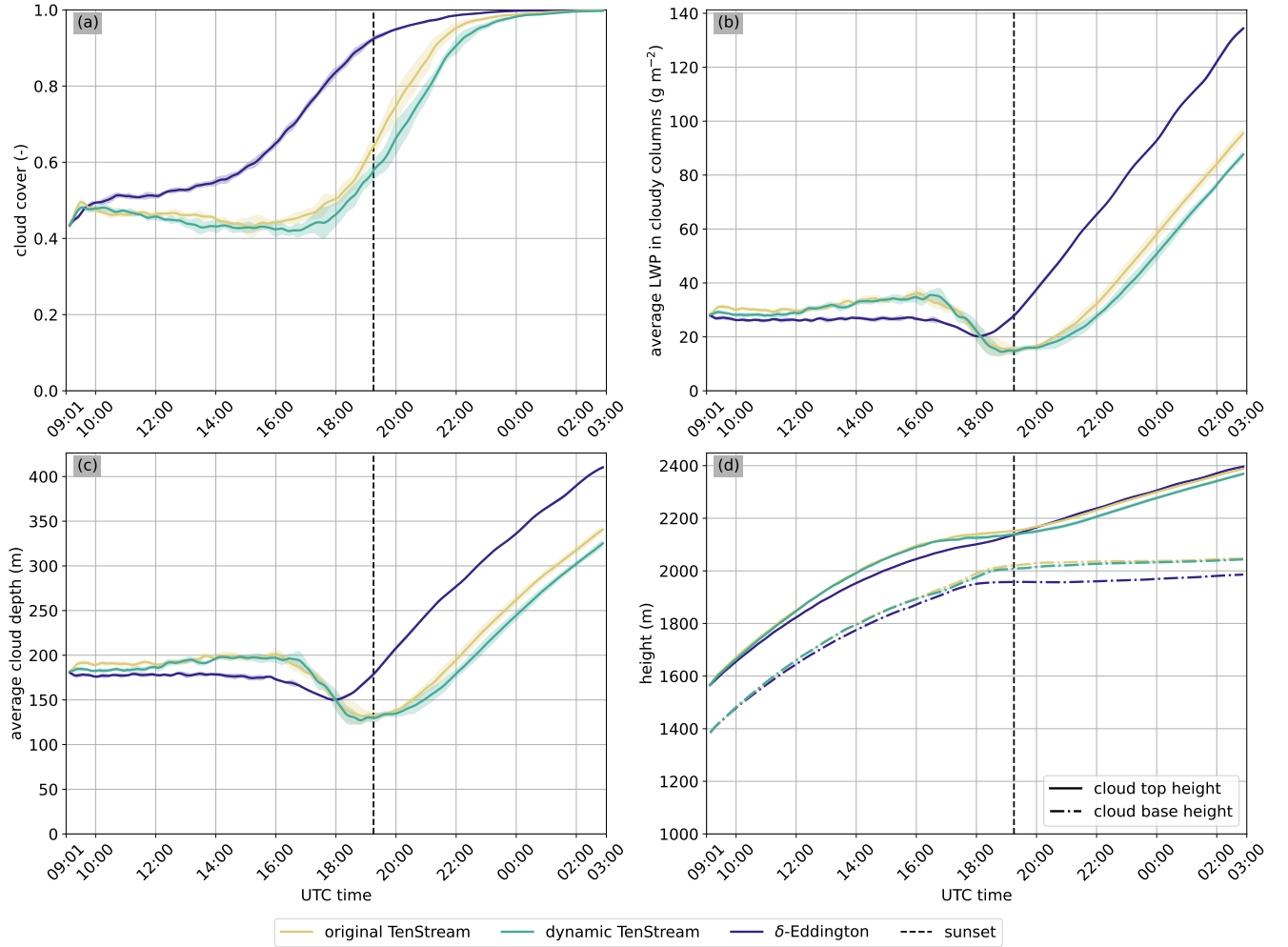
Figure 4. Temporal evolution of cloud cover (a), average liquid water path in cloudy columns (b), average cloud depth (c), and cloud top and base heights (d) for the six-restart runs simulations introduced in Sect. 2.1.4. The colored lines show the ensemble mean for each radiative transfer solver, while the shaded areas indicate one standard deviation across the corresponding five-member ensemble. The vertical line in all the plots indicates panels marks the sunset time. To improve readability, a 15-minute running mean was applied to the data before plotting.
