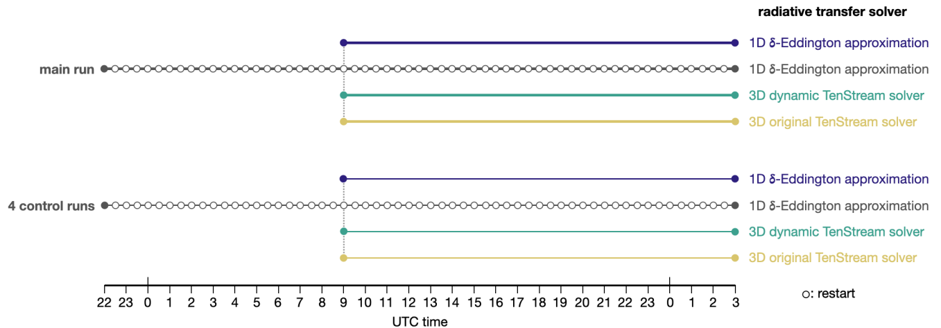
Figure 2. Schematic illustration of all PALM simulations discussed in this paper. On 14 June 2023 at 22:00 UTC, two five simulations, a main run and a four statistically independent but otherwise identical control run runs ( both all shown in gray here), were started. These two five initial model runs were driven by 1D radiation and restarted every 30 minutes, as visualized indicated by the open circles in their respective timelines. Starting at 09:00 UTC on 15 June 2023, three additional restart runs were launched from each of the two these five initial runs. All these in total six 15 restart runs were calculated in one go . They only performed without further restarts and differed only in the radiative transfer model applied: the purple runs were driven by a 1D \delta -Eddington approximation, the turquoise ones by the dynamic TenStream solver, and the ochre ones by the original TenStream solver, resulting in a five-member ensemble for each radiative transfer solver . Filled circles, in contrast to the open circles, visualize the start and end points of each PALM simulation.
