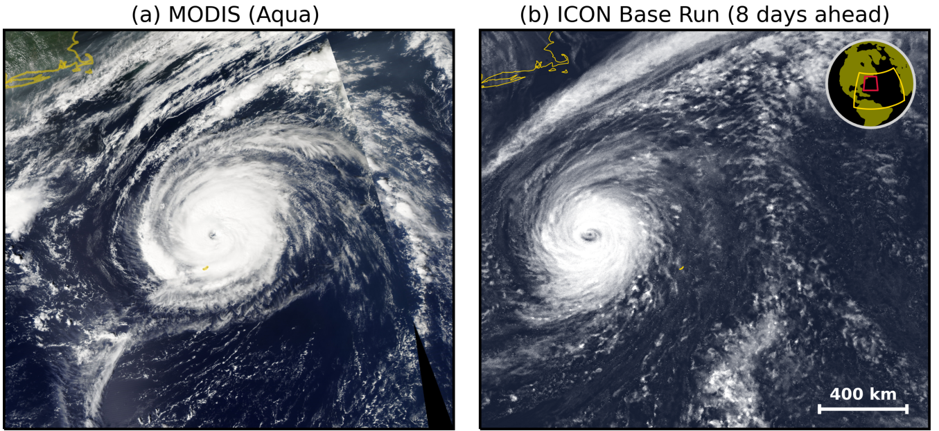
Figure 5. Top view of hurricane Paulette from (a) observations and (b) simulations. A regional cutout in the Atlantic ocean was defined reaching from -74.0 to -53.4 ^{\circ} E and from 25.0 to 43.2 ^{\circ} N. Subpanel (a) shows a true-colour image acquired by the Moderate Resolution Imaging Spectroradiometer (MODIS) instrument on the NOAA-AQUA satellite during an ascending orbit at overpass time on 14 September 2020, around 18:00 UTC. Subpanel (b) provides a simulation of the reflected solar radiation flux, normalized between 100 and 750 \text{W m}^{-2} from our ICON base run, which was initialized on 7 September 2020 at 0 UTC. The time, geographical region and projection have been matched between the observation and the simulation. The color scale and map in (b) have been adjusted to ensure visual consistency with (a). The length scale of 400 km is shown in the lower right corner of (b) and the inset in the upper right corner of (b) shows the location of the image cutout (red outline) and the inner base run domain (yellow outline) in the Atlantic ocean.
