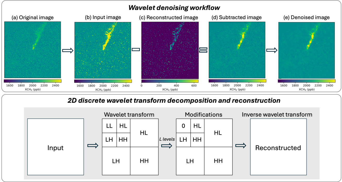
Figure 1. Wavelet denoising workflow. (a): an original image example; (b): output of pre-processing; (c): output of wavelet transform and inverse wavelet transform with low frequencies removed; (d): output after subtracting (c) from (b); (e): output of applying soft thresholding wavelet denoising to (d). Wavelet denoising workflow and illustrative decomposition process. The figure is organized into two rows to distinguish the data processing pipeline from the underlying wavelet transform operations. Top row (left to right): (a) original input image, (b) pre-processed input image, (c) reconstruction from wavelet transform with approximation coefficients removed, (d) residual image obtained by subtracting (c) from (b), and (e) final denoised image after applying soft-thresholding wavelet denoising to (d). Bottom row: illustration of the 2D discrete wavelet transform workflow, showing (i) decomposition into wavelet coefficients, (ii) modification of coefficients by removing the approximation components, and (iii) inverse transform reconstruction used to generate (c).
