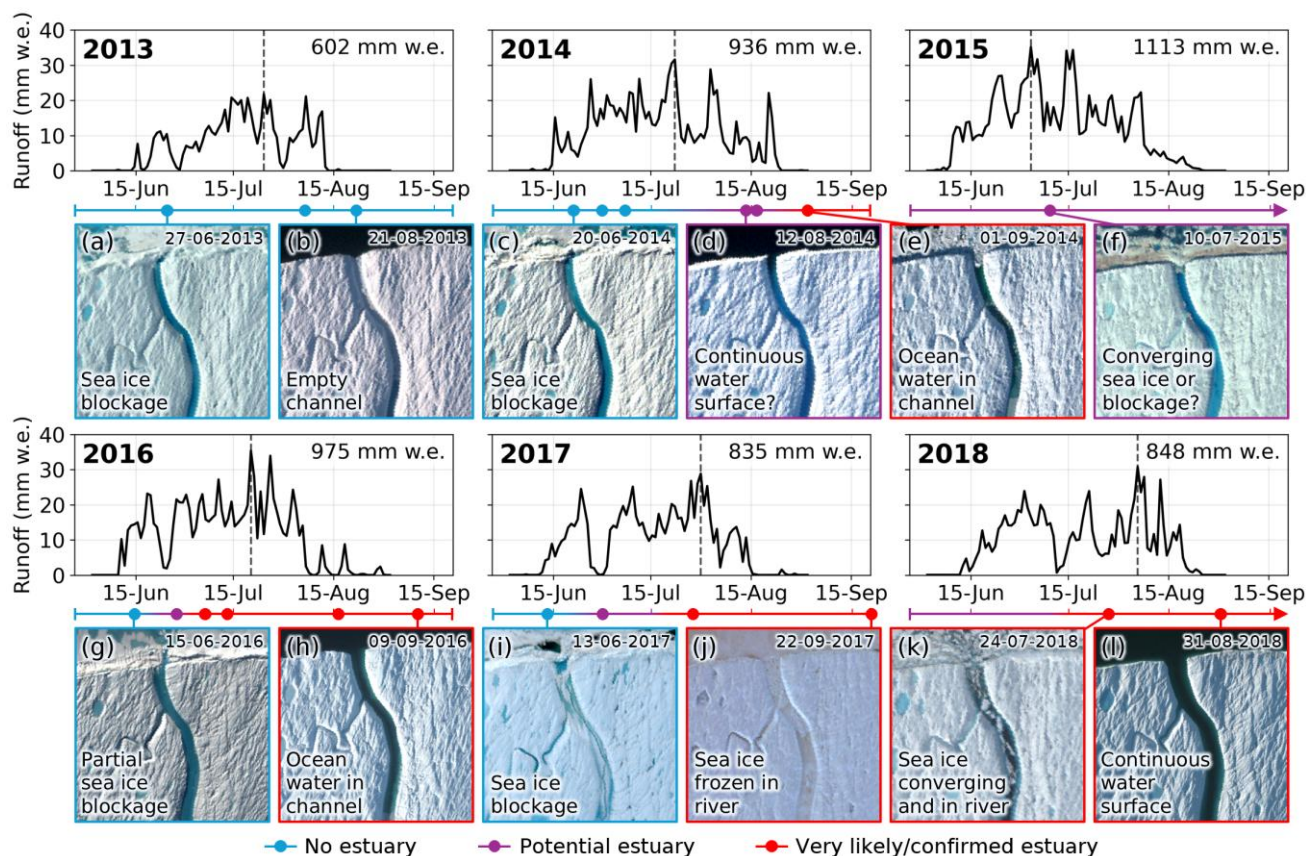
Figure 8: Timeline of Petermann ice-shelf estuary formation showing surface runoff and WorldView imagery from 2013 to 2018 (copyright Vantor 2025). Summer (1 June to 15 September) runoff over Petermann Ice Shelf from MAR is shown in black with a dashed line indicating peak runoff. A corresponding timeline coloured by likelihood of estuary presence ( blue for no estuary, purple for ambiguous, and red for estuary ) is shown below each of the runoff plots, with coloured circles on the timeline representing availability of cloud-free WorldView-2/3 images; 12 example images (a-l; all at the same spatial scale ) are shown below their respective coloured circles on the timeline and Images are labelled with relevant estuary formation criteria information. Gradients between two solid colours on the timeline indicate that a change in estuary likelihood occurred between two dates, but that the exact timing cannot be determined. At the end of each melt season, it is assumed that the conditions from the last cloud free image persist until refreezing. Additional images used to develop the timeline but not shown here can be found in Fig. S9.
