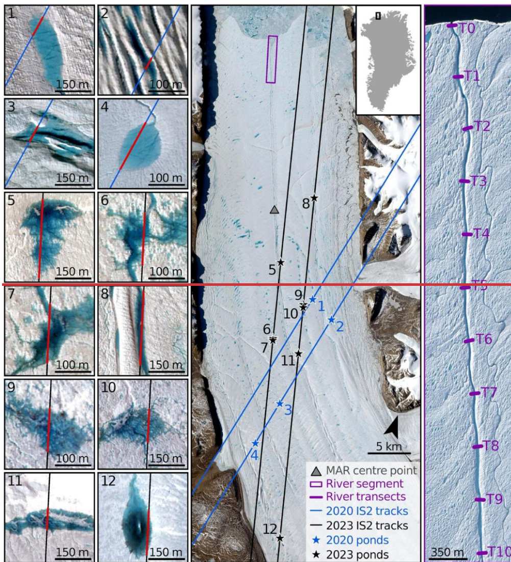
Figure 2: Sentinel-2 image of Petermann Ice Shelf from 27 June 2023, with locations of ponds, ICESat-2 beams, and river segments, and grounding zone (Ciraci et al., 2023) labelled, labelled. Inset map shows the location of Petermann Ice Shelf in northwest Greenland. WorldView-2 images of ponds 1-4 (copyright Vantor 2020), all acquired 17 August 2020, are shown with corresponding ICESat-2 beams in blue. WorldView-2 images of ponds 5-12 (copyright Vantor 2023), all acquired 27 June 2023, are shown with corresponding ICESat-2 beams in black. Pond-beam intersections are shown in red. A WorldView-2 image from 12 August 2014 of the final 5 km segment of the supraglacial river (copyright Vantor 2014) shows the locations of the transects used in Fig. 7 in purple.
