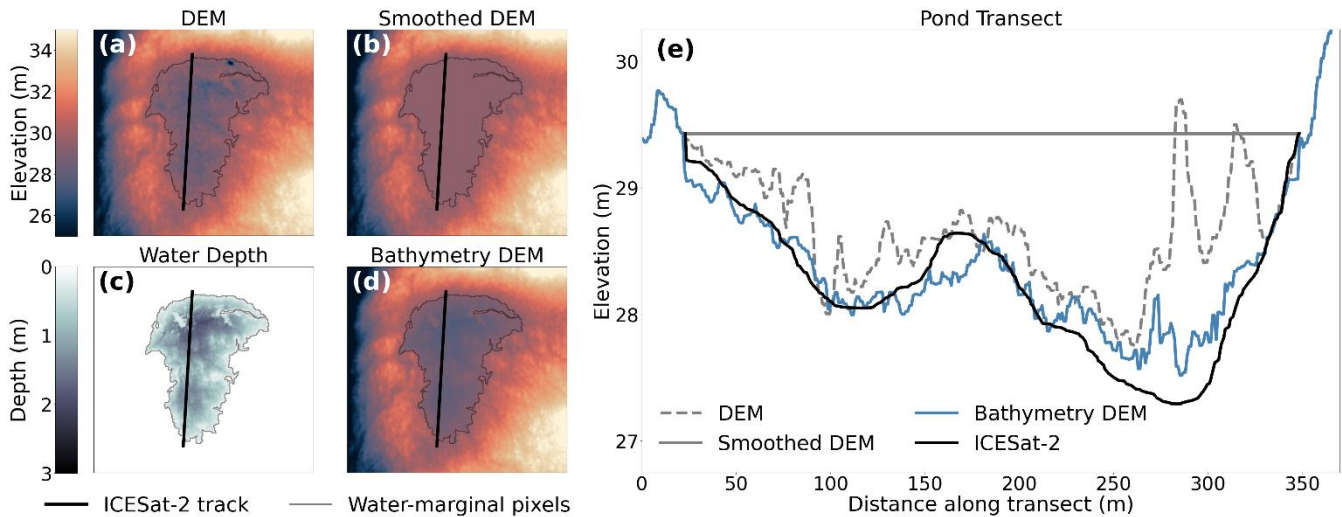
Figure 5: Example of bathymetry calculation for Pond 5. Subplots show (a) original WorldView DEM (Porter et al., 2022) DEM with water-marginal pixels in grey and ICESat-2 transect location in black, (b) Smoothed DEM with water surface set equal to mean water-marginal pixel elevation, and (c) meltwater depth calculated from WorldView-2 imagery, (d) Bathymetry DEM, equal to smoothed DEM surface minus water depth, and (e) elevation profiles along the ICESat-2 transect. Examples of bathymetry calculation for all ponds can be found in Fig. S3.
