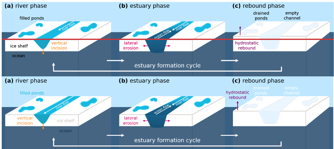
Figure 9: Schematic of the proposed estuary formation cycle. During the early melt season, the channel is in its river phase (a), where meltwater is exported from the ice shelf into the ocean through river flow, causing the river to incise vertically into the ice-shelf surface. Once the river incises to the point where the channel bottom reaches sea level, the estuary phase (b) begins. During this phase, meltwater export from the ice shelf is limited inhibited by mixing with seawater ocean water , leading to flow reversal in the lower part of the river channel, with seawater ocean water flowing up the channel. In this phase, lateral erosion rather than vertical incision dominates, causing the channel to widen. The rebound phase (c) occurs towards the end of the melt season as surface melting ceases and meltwater is offloaded from the ice-shelf surface, causing the most downstream part of the ice shelf to hydrostatically flex upwards, thereby raising the channel bottom above sea level; refreezing of seawater in the river channel likely also contributes to elevating the channel bottom above sea level. After surface melting has initiated in the subsequent summer, the river may start to flow again, and the estuary formation process recommences.
