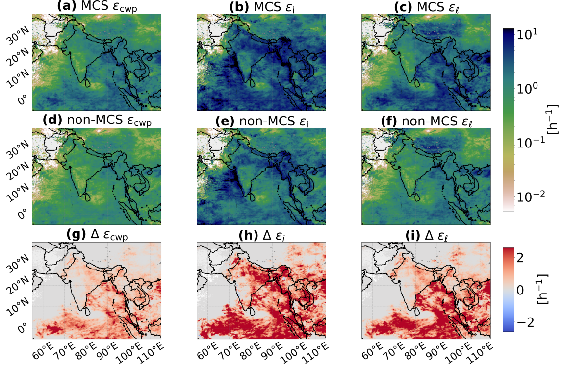
Figure 3. MCSs exhibit much higher \varepsilon with mean values 50% greater than for non-MCS convection across all phases. Spatial distribution of \varepsilon metrics over the Asian monsoon region for MCSs and non-MCS convection. The top row (a–c) shows MCS \varepsilon based on overall cloud water path ( \varepsilon_{\text{cwp}} ), ice water path ( \varepsilon_i ), and liquid water path ( \varepsilon_\ell ). The middle row (d–f) presents the corresponding non-MCS precipitation efficiencies, while the bottom row (g–i) shows the MCS–non MCS differences ( \Delta\varepsilon = \varepsilon^{\text{MCS}} - \varepsilon^{\text{non-MCS}} ).
