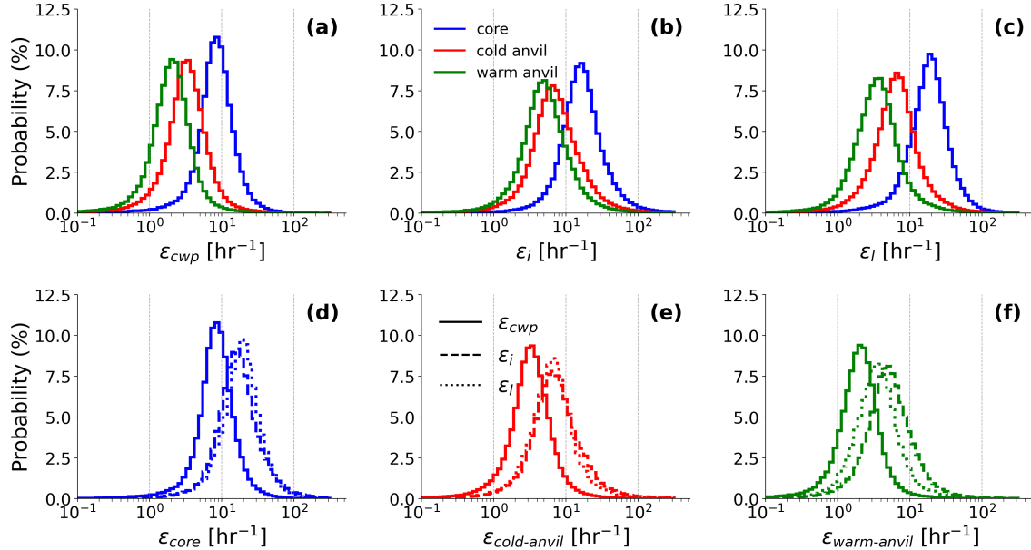
Figure 6. The core consistently has the highest \varepsilon values, followed by the cold and then warm anvils, reflecting the transition from deep convective to stratiform and non-precipitating cloud. Probability distributions of \varepsilon across MCS morphologies, defined by Tb thresholds in the FLEXTRKR data. Panels (a–c) show distributions of \varepsilon for the convective core (blue), cold anvil (red), and warm anvil (green) regions, computed for (a) overall precipitation efficiency ( \varepsilon_{cwp} ), (b) ice-phase efficiency ( \varepsilon_i ), and (c) liquid-phase efficiency ( \varepsilon_\ell ). Panels (d–f) regroup the distributions by MCS region to compare total and phase-partitioned \varepsilon within each sector: (d) for the core, (e) for the cold anvil, and (f) for the warm anvil. In panels (d–f), solid lines denote \varepsilon_{cwp} , dashed lines denote ice-phase efficiency ( \varepsilon_i ), and dotted lines denote liquid-phase efficiency ( \varepsilon_\ell ).
