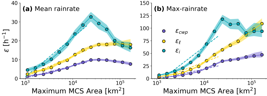
Figure 7. For both mean and maximum rain rates, \varepsilon increases with MCS size for areas less than 2 \times 10^4 km 2 . Scalings of the \varepsilon metrics versus MCS area for (a) lifetime mean rain rate and (b) lifetime maximum rain rate. The MCS area shown represents the full tracked evolution of PyFLEXTRKR systems, including stages before they satisfy the MCS identification criteria (minimum precipitation-feature area of 4 \times 10^4 km 2 ). Consequently, areas smaller than 4 \times 10^4 km 2 correspond to the developing stages of systems that subsequently evolve into MCSs. Curves show the total precipitation efficiency ( \varepsilon_{cwp} , purple), liquid-phase efficiency ( \varepsilon_l , yellow), and ice-phase efficiency ( \varepsilon_i , cyan). Dashed lines indicate log-linear fits to the \varepsilon -area relationship, computed only for MCS areas smaller than 2 \times 10^4 km 2 . Shading indicates the 95% bootstrap confidence interval on the binned median \varepsilon metrics within each MCS-area bin.
