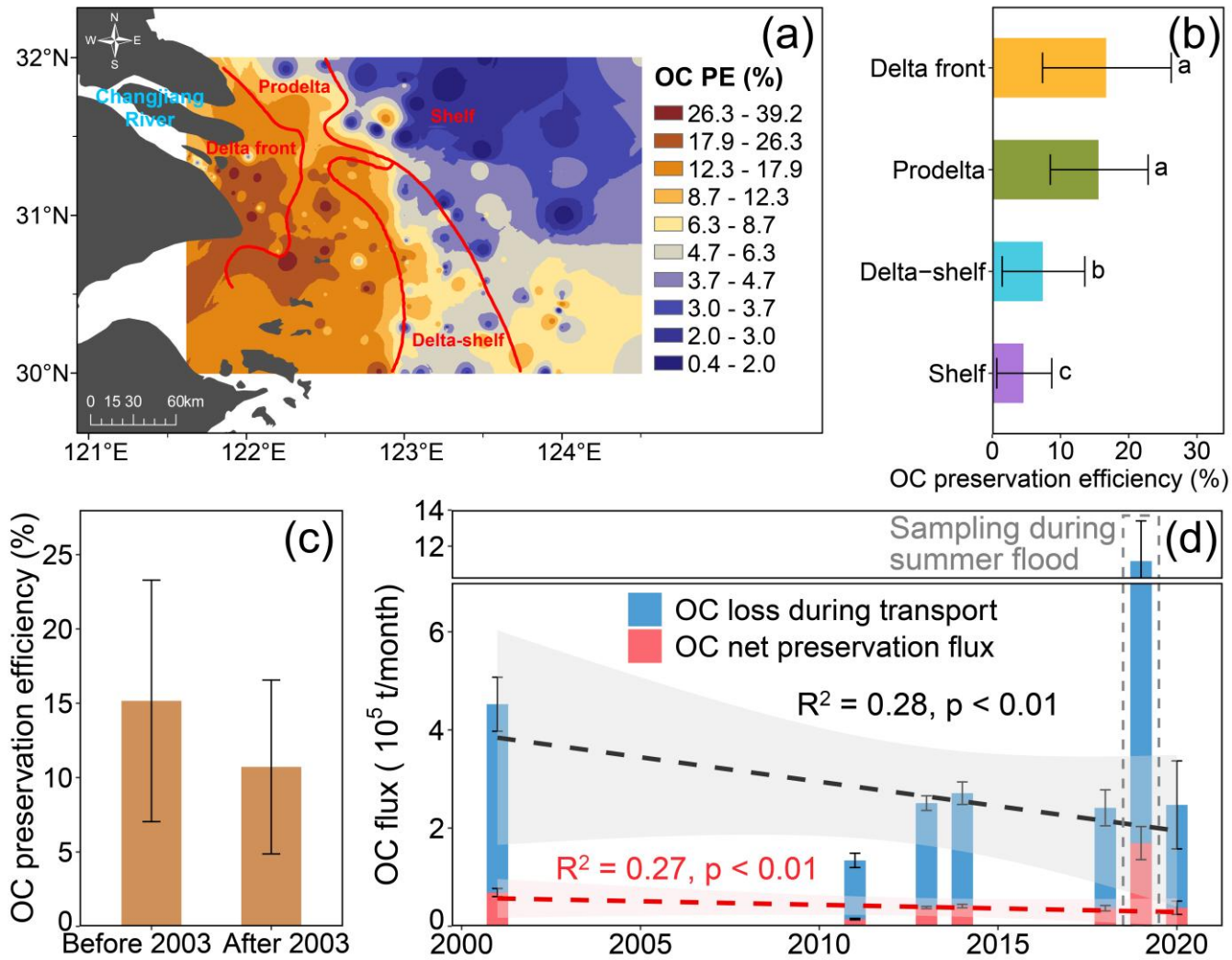
Figure 4 Spatial pattern of organic carbon (OC) preservation efficiency in the Changjiang subaqueous delta (a), and OC preservation efficiency in different sedimentary facies (b). Changes in OC preservation efficiency in the Changjiang subaqueous delta before and after 2003 (c). Temporal trends in the amount of OC preserved in deltaic sediments (red dashed line) and riverine OC flux (black dashed line) from 2001 to 2020, and the blue bars reflect OC loss (difference between amount of OC preservation and riverine OC flux) during sediment transport (d). The PE indicates preservation efficiency in panel (a). Different lowercase letters in panel (b) denote statistically significant differences ( p < 0.05 ) among sedimentary facies. In panel (d), the high value in 2019 (gray dashed
