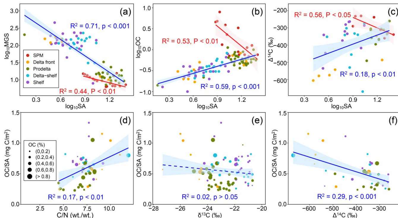
Figure 5 Relationships among medium grain size (MGS), specific surface area (SA), organic carbon (OC) properties, and SA-normalized OC loading (OC/SA) in suspended particulate matter (SPM) from the Changjiang Estuary and surface sediments from the Changjiang subaqueous delta. Relationships of SA with MGS (a), OC content (b) and \Delta^{14}\text{C} (c) in SPM and surface sediments. Relationships of OC/SA with C/N (d), \delta^{13}\text{C} (e), and \Delta^{14}\text{C} (f) in surface sediments. Solid and dashed lines indicate statistically significant ( p < 0.05 ) and non-significant ( p > 0.05 ) relationships, respectively. Shaded areas represent 95% confidence intervals.
