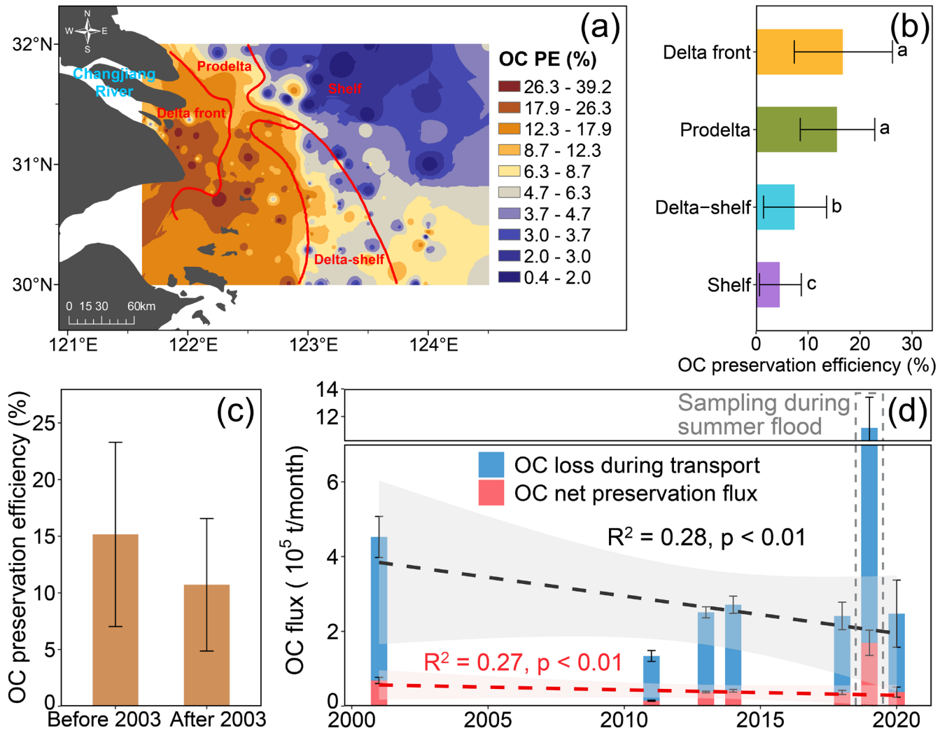
Figure 4 Distribution of organic carbon (OC) preservation efficiency in the Changjiang subaqueous delta (a), and OC preservation efficiency in different sedimentary facies (b). Comparison of OC preservation efficiency before and after 2003 (c). Temporal trends of the amount of OC preserved (red dashed line) in deltaic sediments and riverine OC flux (black dashed line) from 2001 to 2020, and the blue bars reflect OC loss (difference between amount of OC preservation and riverine OC flux) during sediment transport (d). The PE indicates preservation efficiency in panel (a). Different lowercase letters in panel (b) denote statistically significant differences ( p < 0.05 ) among sedimentary facies. In panel (d), the high value in 2019 (gray dashed circles) primarily induced by
