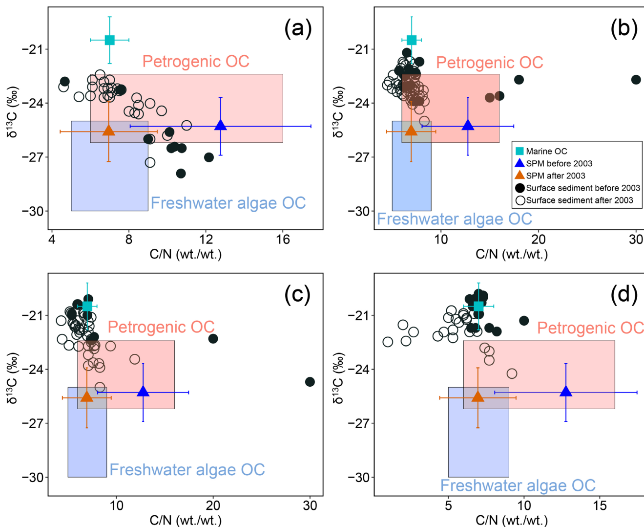
Figure 3 Relationships between \delta^{13}\text{C} and C/N in surface sediments in the Delta front (a), Prodelta (b), Delta-shelf (c) and Shelf (d) before and after 2003. Light red and blue areas represent ranges of \delta^{13}\text{C} and C/N corresponding to terrestrial organic carbon (OC) derived from petrogenic and freshwater algae sources, respectively, in terms of Lamb et al. (2006) and Menges et al. (2020). The marine OC end-member of \delta^{13}\text{C} is from -19.2‰ to -21.8‰ and of C/N is 6–8 (Xing et al., 2011; Bao et al., 2018).
