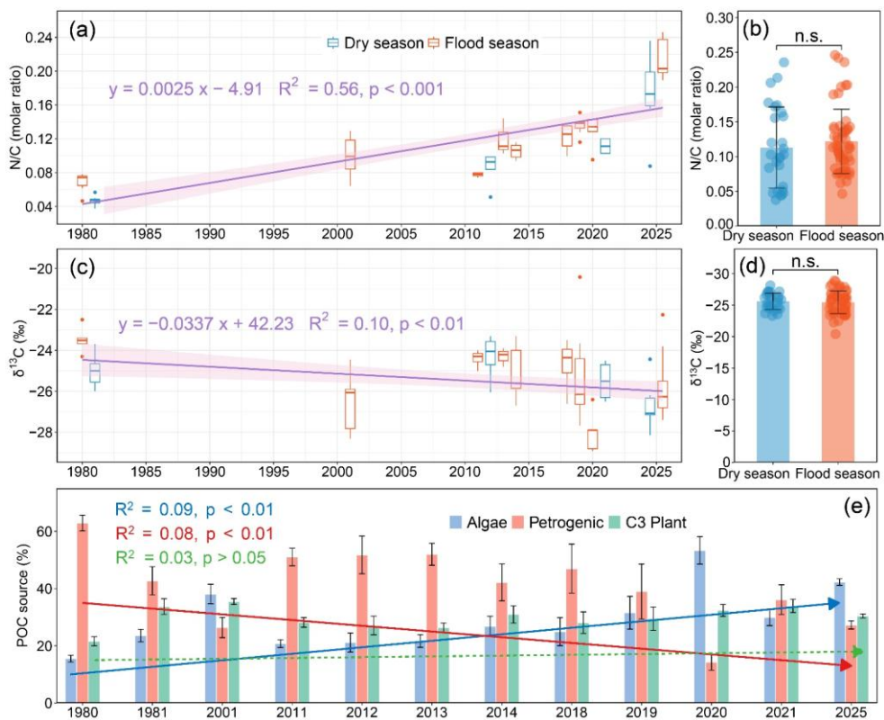
Figure 2 Temporal variations of N/C molar ratios (a) and \delta^{13}\text{C} values (c) in suspended particulate matter (SPM) collected in surface water in the Changjiang Estuary from 1980 to 2025, and the differences of N/C molar ratios (b) and \delta^{13}\text{C} values (d) between dry and flood seasons. Temporal trends of proportions of particulate organic carbon (POC) derived from different terrestrial sources (freshwater algae, petrogenic and C3 plant sources) estimated through a Bayesian End-member Mixing approach from 1980 to 2025 (e). Solid lines represent significant ( p < 0.05 ) linear associations, and the light purple areas around the line indicate 95% confidence interval. The n.s. indicates insignificant ( p > 0.05 ) differences.
