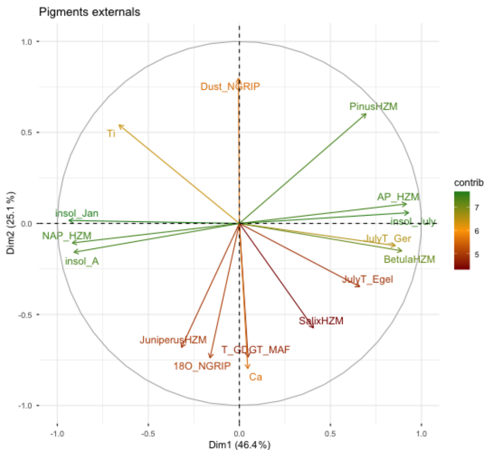
Figure B2. The biplot displays the correlation structure among the independent proxies considered for the Redundancy Analysis (RDA), revealing the primary environmental gradients driving the system. The first axis (Dim1, 46.4 %) represents the dominant climatic and vegetational gradient. It strongly opposes indicators of warmth and forest development (positive loadings: Betula , summer insolation, regional summer temperatures) against markers of cold, open steppe environments (negative loadings: Non-Arboreal Pollen (NAP), Juniperus , winter insolation). The second axis (Dim2, 25.1 %) captures the sedimentological signal, distinguishing allochthonous detrital inputs (positive loadings: Ti , NGRIP Dust) from autochthonous carbonate precipitation (negative loading: Ca ) and climate signals ( \delta^{18}\text{O}_{\text{NGRIP}} ). This analysis demonstrates the high collinearity between local vegetation and regional temperature records, justifying the VIF selection of a reduced subset of non-redundant variables for the final RDA model.
