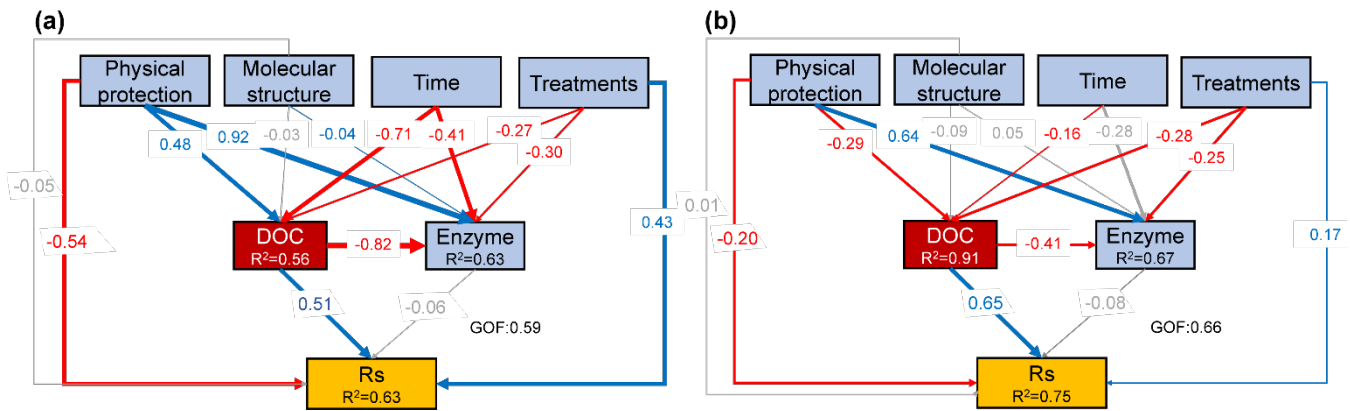
360 Figure 7: Path analysis results showing the direct and indirect controls of soil organic carbon (SOC) mineralization. Blue and red numbers indicate significant positive and negative relationships ( p < 0.05 ), whereas grey numbers indicate non-significant pathways. R^2 is the coefficient of determination, denoting the proportion of variance explained by the model. Panel (a) represents topsoil and panel (b) represents subsoil. Rs denotes the SOC mineralization rate during the thawing phase of each freeze–thaw cycle. Indicators of the latent variables are listed in Table S2, and their loadings are shown in Fig. S8.
