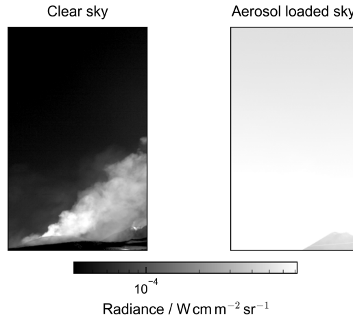
Figure 6. Grey-scale images demonstrating the considered range of sky brightness at 6380\text{ cm}^{-1} in the NIR.
