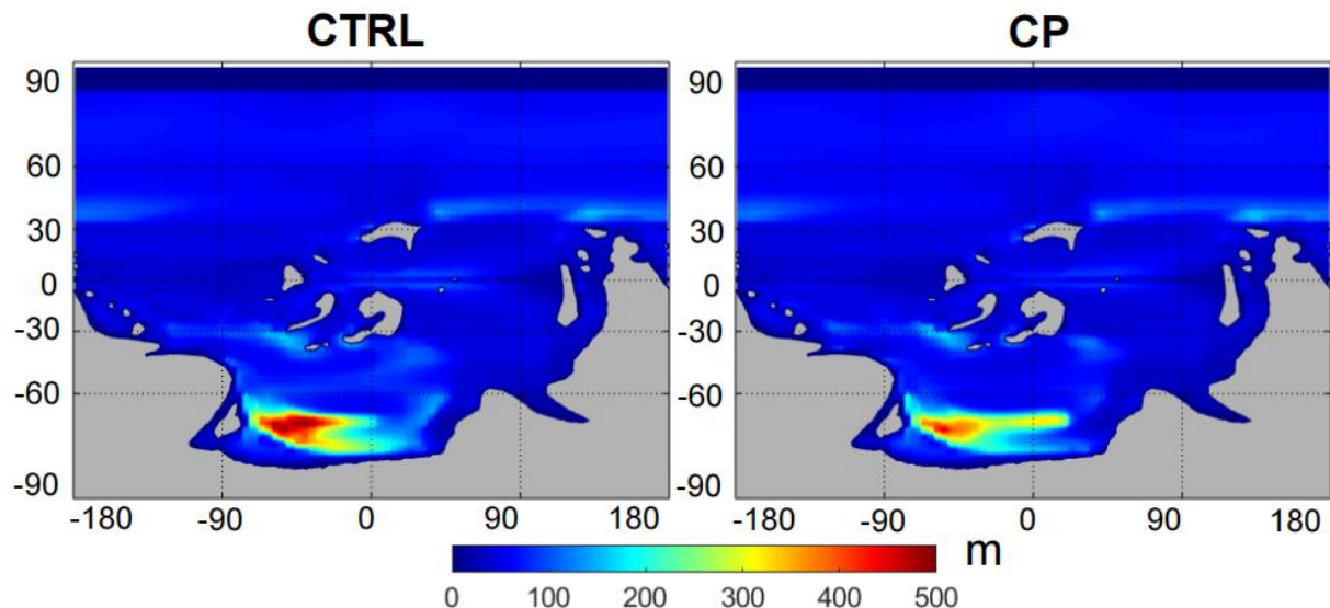
Figure C6: Comparison of mixed-layer depth between the CTRL and CP experiments. Shading indicates mixed-layer depth (m).
