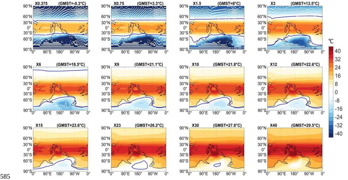
585 Figure C1: Late Ordovician climate sensitivity to CO 2 . Annual mean surface temperature under different PAL CO 2 conditions. White dots represent the extent of the cryosphere: sea ice is defined based on the annual mean sea ice fraction (indicating perennial ice), while land ice is defined as areas where the annual mean water-equivalent snow depth exceeds 1 m, representing potential regions for continental ice development. The results show that, in the uncoupled ice sheet scenario, a CO 2 level of 6 PAL marks the threshold for initiating continental ice formation, whereas only when greenhouse gas concentrations drop sufficiently low (~1 PAL) can land ice marginally extend to around 60° S. The development of sea ice in the SH ocean lags that of land ice. The blue solid lines represent the 0 °C.
