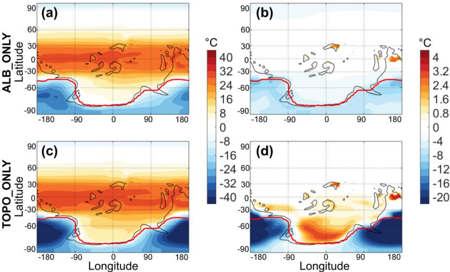
425 Figure 11: Surface temperature responses in the slab-ocean sensitivity experiments isolating ice-sheet albedo and topography effects. Left panels (a, c) show the annual mean surface temperature in the ALB_ONLY (a) and TOPO_ONLY (c) experiments. Right panels (b, d) show the differences relative to the CTRL, highlighting the temperature response exclusively due to ice-sheet albedo (b) and topography (d). The red contour in each panel denotes the ice-sheet margin in the full glacial configuration.
