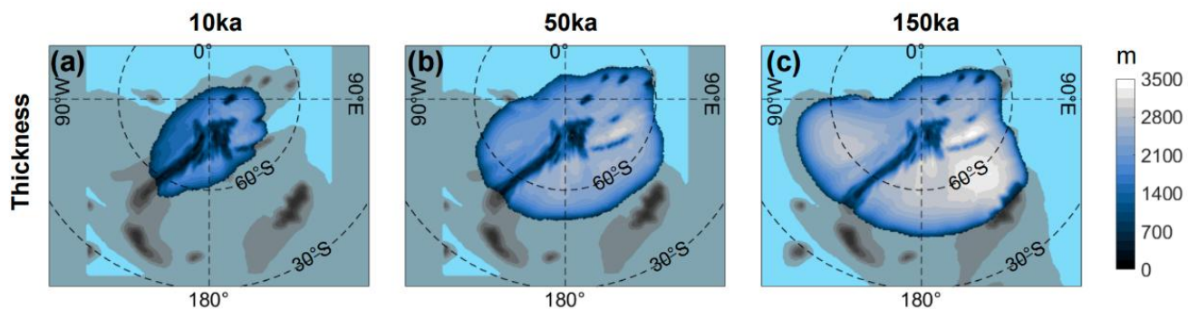
Figure C2: land-ice thickness in case CP. Three snapshots from the coupled framework simulation at (a) 10 ka, (b) 50 ka, and (c) 150 ka. Latitude is shown at 30° intervals.
