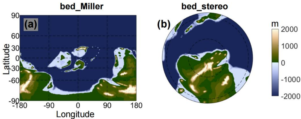
Figure 1: Late Ordovician palaeogeography. (a) Late Ordovician palaeogeography under the Miller projection. (b) As (a), but with a stereographic projection centered at the South Pole.
