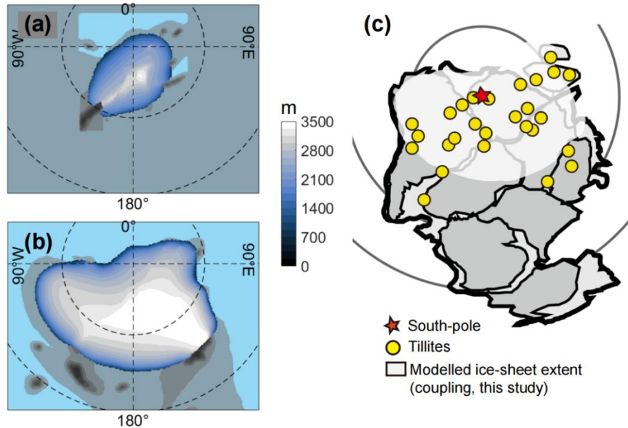
Figure 2: Late Ordovician glacial tillites and ice sheet surface. (a) Equilibrium result of the ice sheet surface topography (blue-grey color) simulated by the offline method at 6 PAL. The bedrock topography is indicated by a greyscale whose colorbar is not shown here but more details can be found in Fig. 1. (b) As (a), but with coupled climate and ice sheet models. Latitude is shown at 30^\circ intervals. (c) Locations of glacial deposits (Cocks and Torsvik, 2021).
