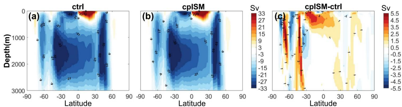
Figure 9: Oceanic meridional overturning circulation. Panels show the ocean meridional overturning streamfunction for (a) case CTRL, (b) case CP and (c) the difference (CP minus CTRL). Negative values indicate counterclockwise circulation.
