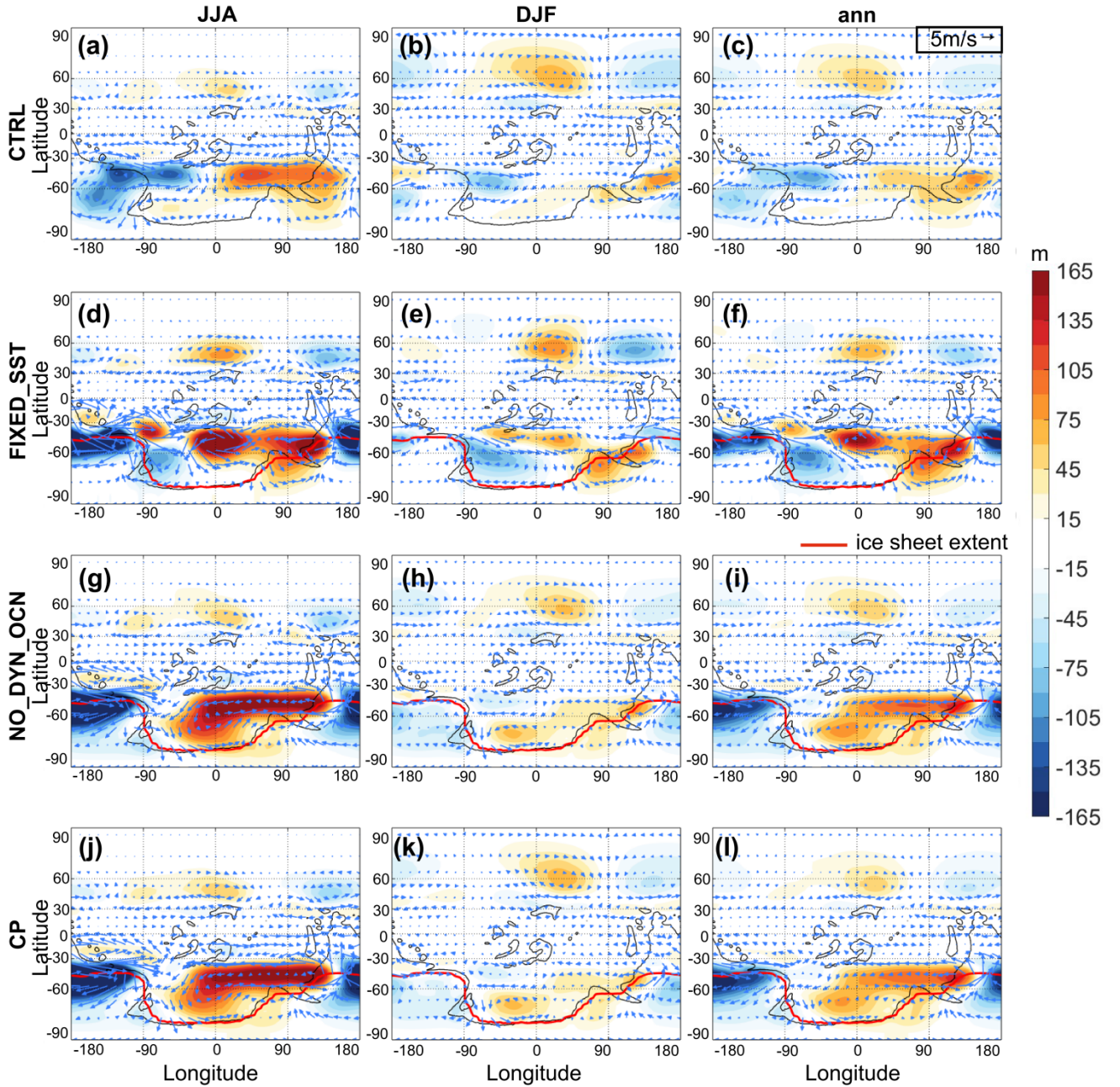
Figure 6: Structure of the stationary waves. (a-c) 500 hPa geopotential height and wind field from the CTRL, with zonal average subtracted. (d-f) As (a-c), but for the prescribed-SST experiment results. And (g-i) for the case NO_DYN_OCN, (j-l) for the coupled experiment.
