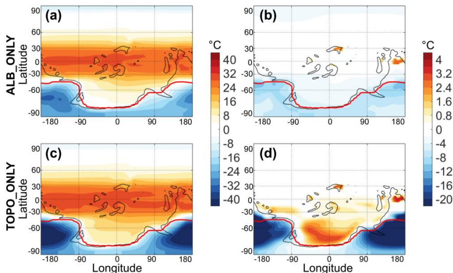
Figure 11: Surface temperature responses in the slab-ocean sensitivity experiments isolating ice-sheet albedo and topography effects. Left panels (a, c) show the annual mean surface temperature in the ALB_ONLY (a) and TOPO_ONLY (c) experiments. Right panels (b, d) show the differences relative to the CTRL, highlighting the temperature response exclusively due to ice-sheet albedo (b) and topography (d). The red contour in each panel denotes the ice-sheet margin in the full glacial configuration.
