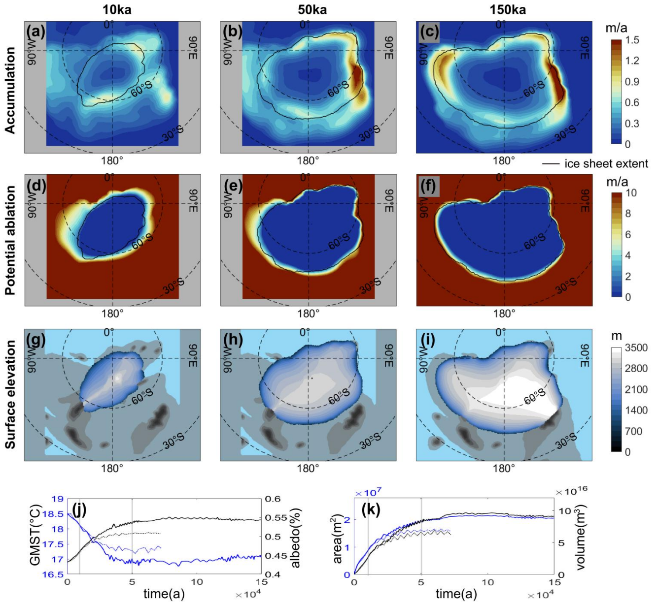
Figure 3: Contribution of accumulation and ablation to ice sheet growth. Three snapshots from the coupled framework simulation (CP) at (a, d, g) 10 ka, (b, e, h) 50 ka, and (c, f, i) 150 ka. The rows from top to bottom show accumulation, potential ablation, and surface elevation of the ice sheet, and the corresponding time series. In particular, when displaying time series, the left panel shows the evolution of GMST (°C; blue) and global annual mean land surface albedo (%) (black), and the right panel shows ice-sheet area (m 2 ; blue) and ice-sheet volume (m 3 ; black). Solid lines show the fully coupled experiment (CP), while dashed lines show the supplementary experiment in which the ice-sheet area was set to 0 during coupling (CP_NO_ALB). The black contour represents the ice-sheet edge. Latitude is shown at 30° intervals.
