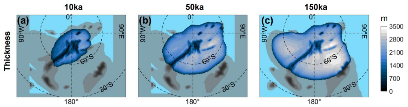
Figure C2: land-ice thickness in case CP. Three snapshots from the coupled framework simulation at (a) 10 ka, (b) 50 ka, and (c) 150 ka.
