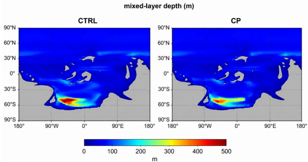
Figure C6: Comparison of mixed-layer depth between the CTRL and CP experiments. Shading indicates mixed-layer depth (m).
