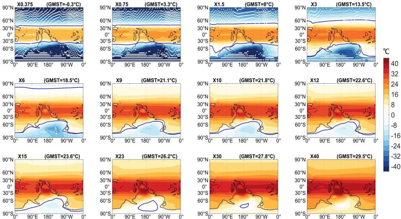
Figure C1: Late Ordovician climate sensitivity to \text{CO}_2 . Annual mean surface temperature under different PAL \text{CO}_2 conditions. White dots represent the extent of the cryosphere: sea ice is defined based on the annual mean sea ice fraction (indicating perennial ice), while land ice is defined as areas where the annual mean water-equivalent snow depth exceeds 1 m, representing potential regions for continental ice development. The results show that, in the uncoupled ice sheet scenario, a \text{CO}_2 level of 6 PAL marks the threshold for initiating continental ice formation, whereas only when greenhouse gas concentrations drop sufficiently low ( \sim 1 PAL) can land ice marginally extend to around 60^\circ\text{S} . The development of sea ice in the SH ocean lags that of land ice. The blue solid lines represent the 0^\circ\text{C} .
