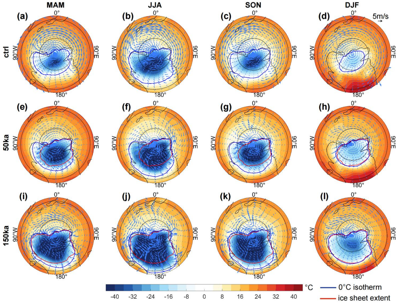
Figure 4: Surface wind field and temperature. (a-d) Surface wind field and surface temperature from the equilibrium of the CTRL for March, April, May (MAM); austral winter (June, July, and August; JJA); September, October, November (SON); and austral summer (December, January, and February; DJF). Two snapshots from the coupled framework simulation are shown in (e-h) 50 ka, (i-l) 150 ka. Note that in (e-h) and (i-l), the surface wind is shown as the difference from the CTRL. The 0 °C isotherm and ice-sheet extent are indicated by the blue and red contours, respectively. Latitude is shown at 30° intervals.
