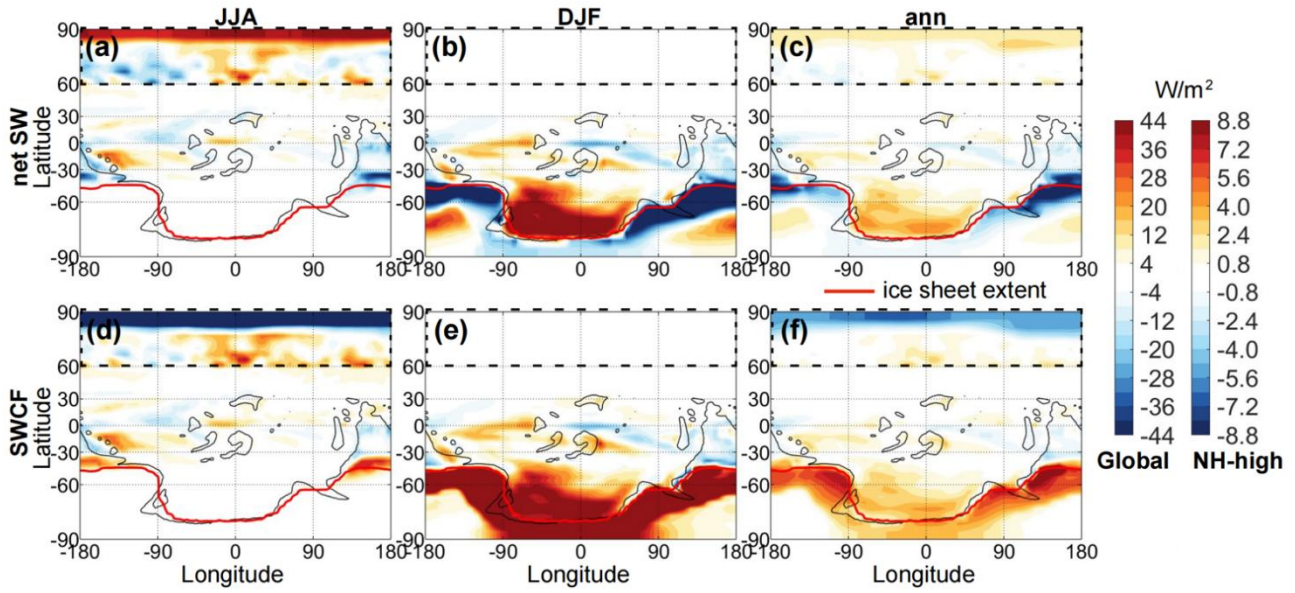
Figure 8: The differences in (a-c) net surface shortwave radiation and (d-f) shortwave cloud radiative forcing between the coupled and the control experiments. Note that the color range for high latitudes in the NH (black dashed box) has been adjusted, as the radiation changes in the NH are relatively minor.
