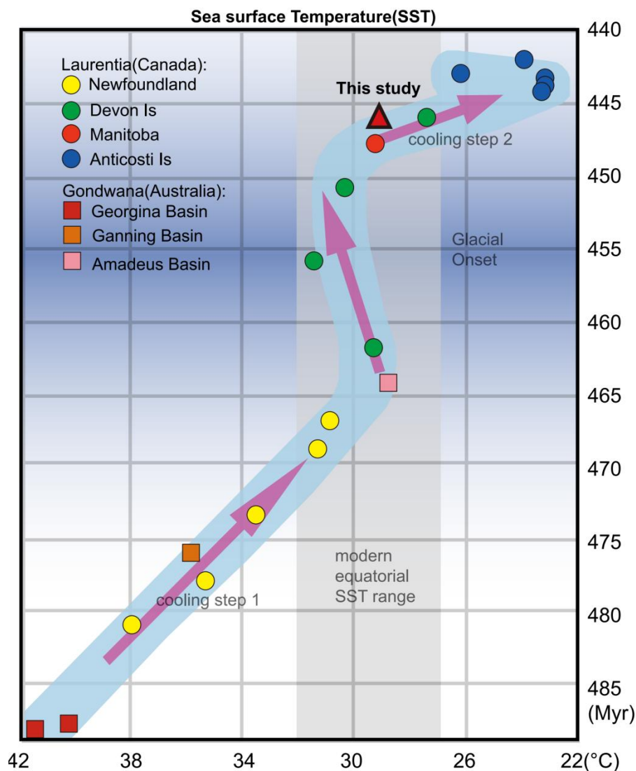
Figure C4: Tropical seawater temperature trend. Generalized tropical seawater temperature trend throughout the Ordovician, derived from conodont oxygen isotope compositions measured in situ. Temperature means are plotted for different analytical sessions. The blue line represents the primary first-order temporal trend of Ordovician sea-surface temperatures. The red triangle represent the tropical sea surface temperatures from this study. Note that these temperatures do not correspond directly in time but have been placed at the Mid-Ordovician based on corresponding temperatures. (Redrawn from Trotter et al., 2008)
