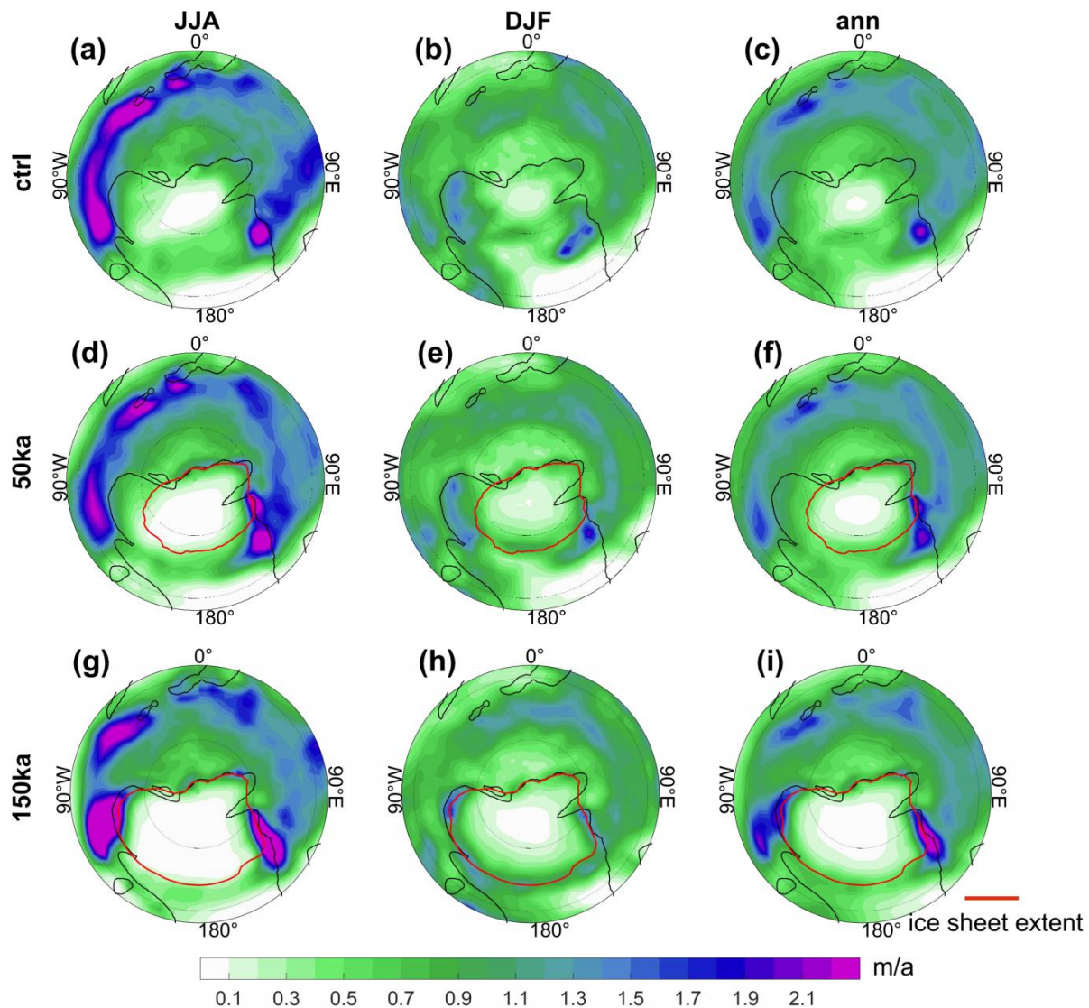
Figure C3: Evolution of precipitation fields. (a-c) Precipitation fields for the case CTRL. Two snapshots for the coupled run: (d-f) 50 ka, (g-i) 150 ka (equilibrium state). From left to right, the three columns represent the austral winter (June, July, and August; JJA); the austral summer (December, January, and February; DJF), and the annual mean, respectively.
