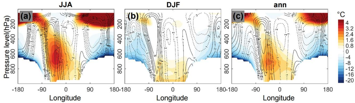
Figure 7: Difference in air temperature (color shading) and meridional wind (contours) along 65° S between the coupled and the control experiments. Solid and dashed contours indicate northerly and southerly wind anomalies, respectively. Note that the color scale is different when showing positive and negative temperature differences.
