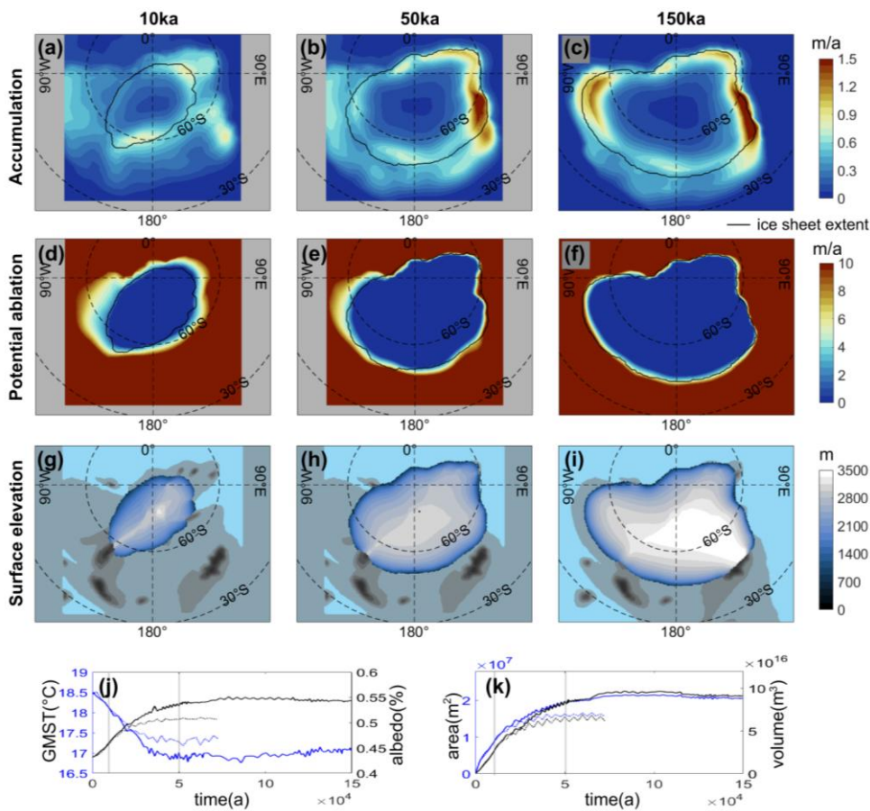
Figure 3: Contribution of accumulation and ablation to ice sheet growth. Three snapshots from the coupled framework simulation (CP) at (a, d, g) 10 ka, (b, e, h) 50 ka, and (c, f, i) 150 ka. The rows from top to bottom show accumulation, potential ablation, and surface elevation of the ice sheet, and the corresponding time series. In particular, when displaying time series, the left panel shows the evolution of GMST (°C; blue) and global annual mean land surface albedo (%; black), and the right panel shows ice-sheet area (m 2 ; blue) and ice-sheet volume (m 3 ; black). Solid lines show the fully coupled experiment (CP), while dashed lines show the supplementary experiment in which the ice-sheet area was set to 0 during coupling (CP_NO_ALB). The black contour represents the ice-sheet edge. Latitude is shown at 30° intervals.
