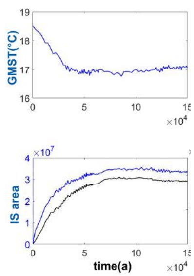
Figure B2: Ice Sheet Coupled Time Series. Time series of temperature, area(m 2 ), and volume(m 3 ) for ice sheet coupling
