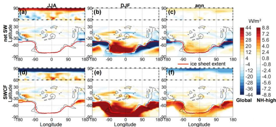
Figure 8: The differences in (a-c) net surface shortwave radiation and (d-f) shortwave cloud radiative forcing between the coupled and the control experiments. Note that the color range for high latitudes in the NH (black dashed box) has been adjusted, as the radiation changes in the NH are relatively minor.
