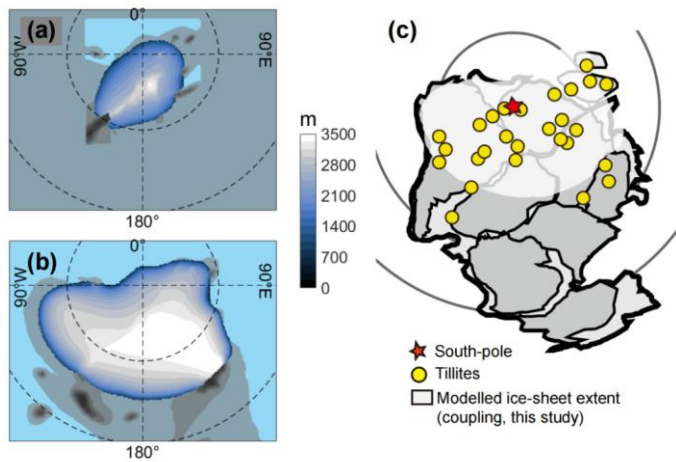
220 Figure 2: Late Ordovician glacial tillites and ice sheet surface. (a) Equilibrium result of the ice sheet surface topography (blue-grey color) simulated by the offline method at 6 PAL. The bedrock topography is indicated by a greyscale whose colorbar is not shown here but more details can be found in Fig. 1. (b) As (a), but with coupled climate and ice sheet models. Latitude is shown at 30^\circ intervals. (c) Locations of glacial deposits (Cocks and Torsvik, 2021).
