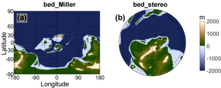
Figure 1: Late Ordovician palaeogeography. (a) Late Ordovician palaeogeography under the Miller projection. (b) As (a), but with a stereographic projection centered at the South Pole.
