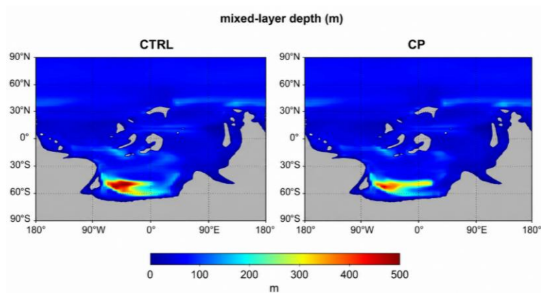
Figure C6: Comparison of mixed-layer depth between the CTRL and CP experiments. Shading indicates mixed-layer depth (m).
