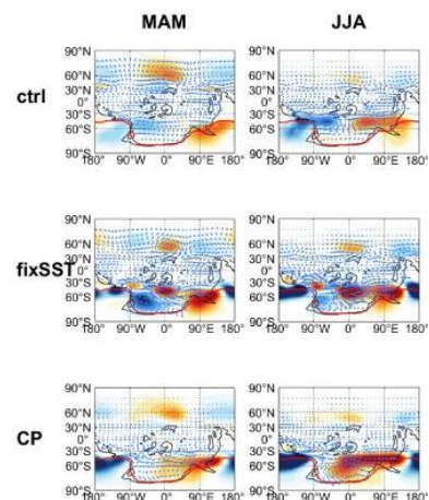
Figure B6: Stationary waves structure of the prescribed SST experiment. 500 hPa geopotential height and wind field from the control experiment, with zonal average subtracted. Top row: . Middle row: . Bottom row: .
