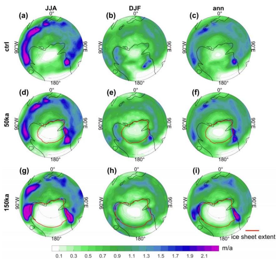
Figure C3: Evolution of precipitation fields. (a-c) Precipitation fields for the case CTRL . Two snapshots for the coupled run: (d-f) 50 ka, (g-i) 150 ka (equilibrium state). From left to right, the three columns represent the austral winter (June, July, and August; JJA); the austral summer (December, January, and February; DJF), and the annual mean, respectively.
