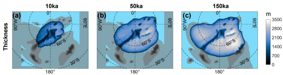
655 Figure C2: land-ice thickness in case CP. Three snapshots from the coupled framework simulation at (a) 10 ka, (b) 50 ka, and (c) 150 ka. Latitude is shown at 30° intervals.
