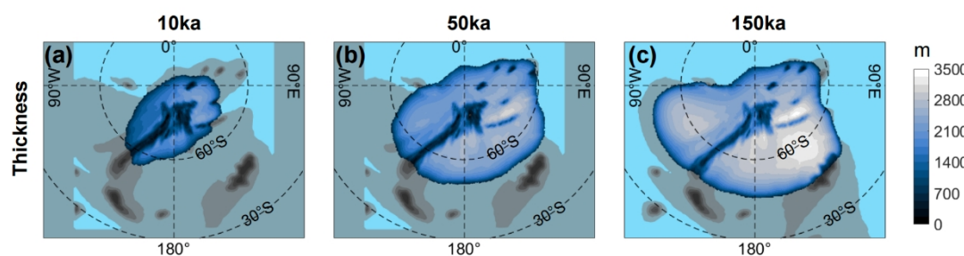
Figure R6 (Fig. S* in the supplementary materials). land-ice thickness in case CP. Three snapshots from the coupled framework simulation at (a) 10 ka, (b) 50 ka, and (c) 150 ka. Latitude is shown at 30° intervals.
