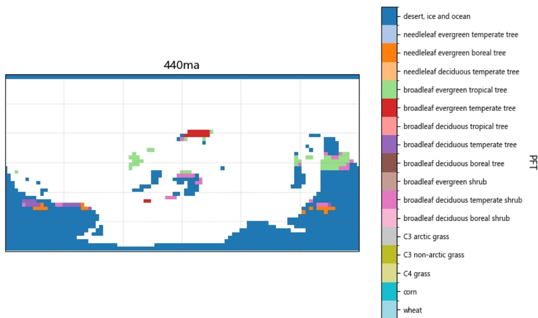
Figure R1. Global vegetation distribution at 440 Ma based on our CNDV simulations. Colors indicate plant functional types (PFTs), including forests (needleleaf and broadleaf, evergreen and deciduous), shrubs, grasses (C3 and C4), and crops (corn, wheat), as well as desert, ice, and ocean areas. This figure illustrates the baseline paleovegetation used in our climate-ice sheet coupled experiments.
