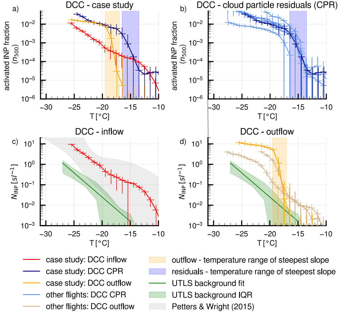
Figure 5. Panel a) shows INP-temperature spectra of flight F15. Red symbols indicate INPs measured in convective inflow, dark blue symbols show INPs from cloud particle residuals (CPR) sampled within DCCs, and orange symbols show INPs partly sampled in convective outflow. To allow convenient comparison between aerosol and cloud residual samples, the activated INP fraction ( N_{\text{INP}}/N_{500} ) is shown. Vertical and horizontal lines mark the 10th to 90th percentiles. Panel b) shows the activated INP fraction of CPR samples from DCCs during other flights of the CIRRUS-HL campaign. Panel c) shows INP concentrations with the convective inflow samples of F15 highlighted. Panel d) shows INP concentrations of DCC outflow samples. In panels a), c) and d), orange and blue shaded areas highlight the temperature range of the steepest slope of the INP spectra in the DCC outflow and in DCC CPR, respectively.
